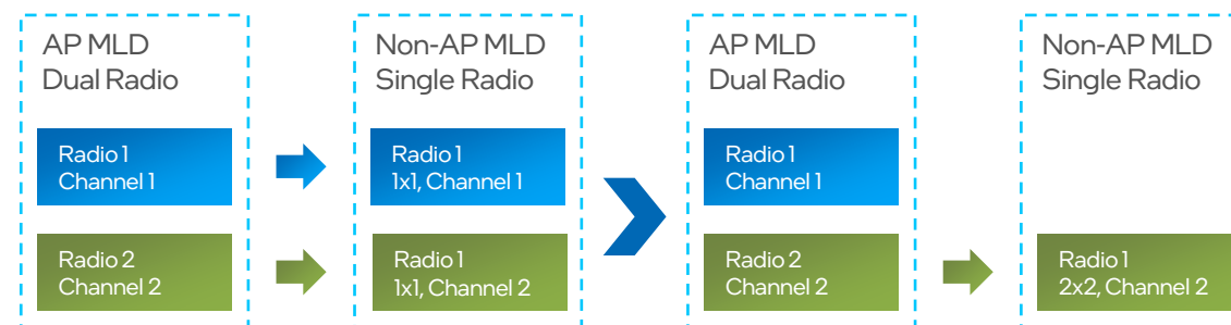
Enhanced Multi-link Single Radio (EMLSR) Operation
