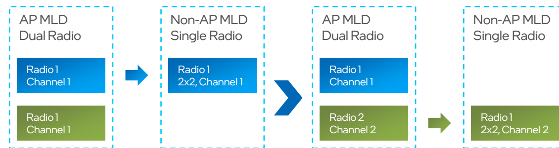
Multi-link Single Radio (MLSR) Operation
