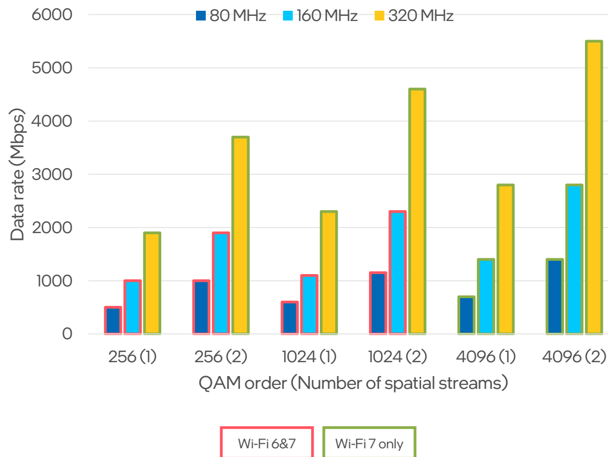
Wi-Fi 7 vs. Wi-Fi 6 Data Rate Comparison
