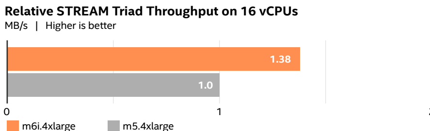
Figure 2. Relative STREAM Triad performance of the 16-vCPU m6i instance vs. the 16-vCPU m5 instance. Higher numbers are better.
