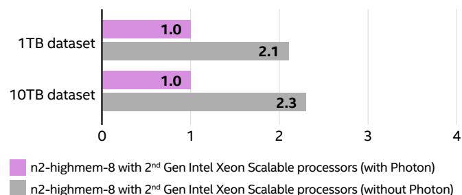
Figure 2. Normalized price/performance to run a decision support workload against a Databricks environment on GCP n2-highmem-8 VMs on both 1TB and 10TB datasets.
