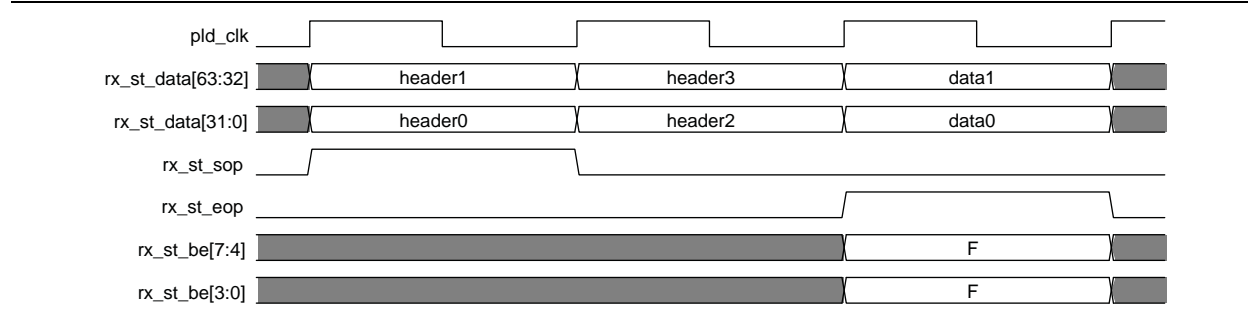
Figure 6-5. 64-Bit Avalon-ST rx_st_data<n> Cycle Definitions for 4-Dword Header TLPs with Qword Aligned Addresses
