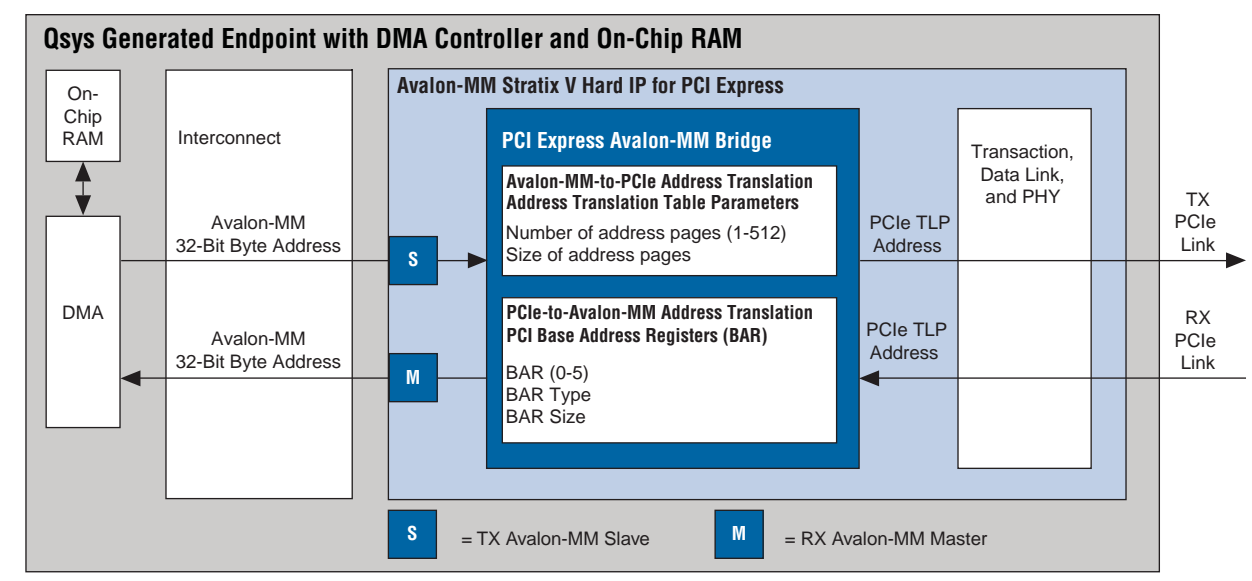
Figure 5-7. Address Translation in TX and RX Directions
