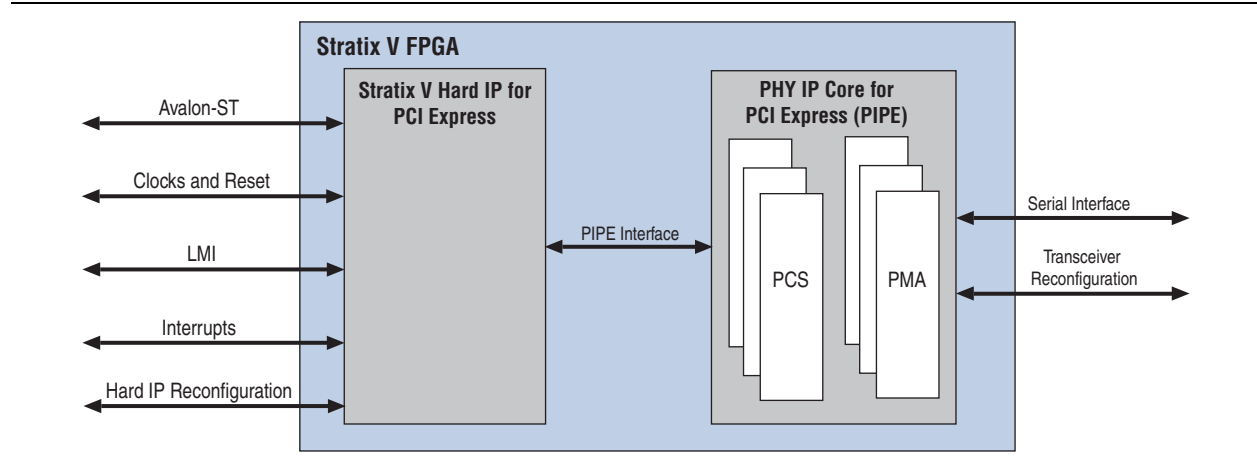
Figure 5-2. Key Interfaces in the Stratix V Hard IP for PCI Express
