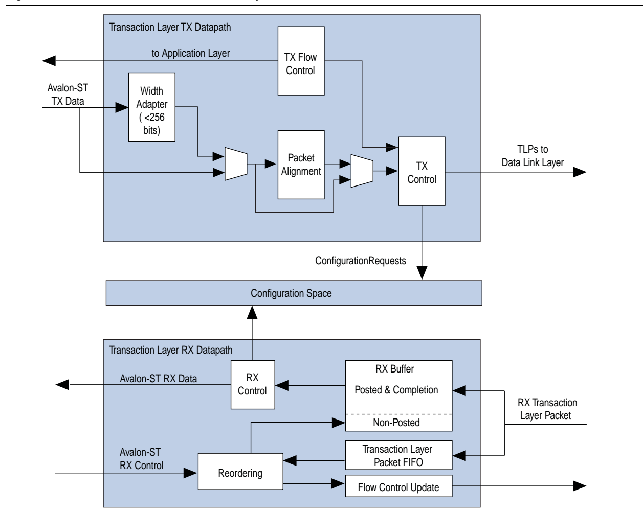
Figure 5-3. Architecture of the Transaction Layer: Dedicated Receive Buffer
