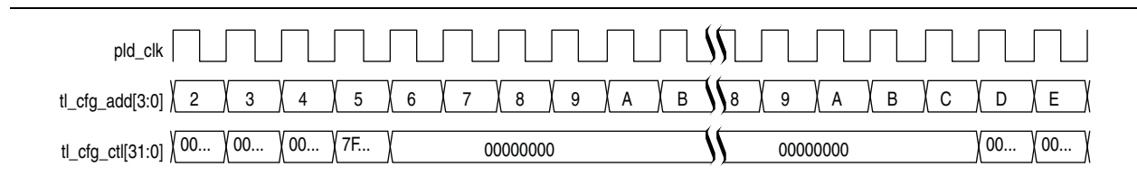
Figure 6-33. tl_cfg_ctl Timing
