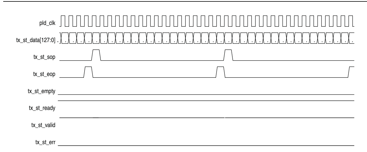
Figure 6-28. 128-Bit Back-to-Back Transmission on the Avalon-ST TX Interface
