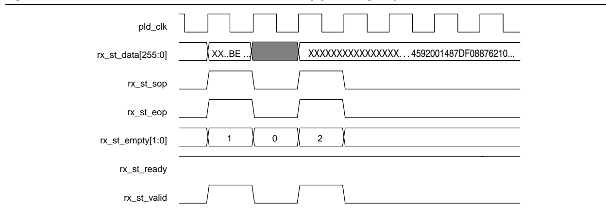
Figure 6-17. 256-Bit Avalon-ST RX Packets Use of rx_st_empty and Single-Cycle Packets
