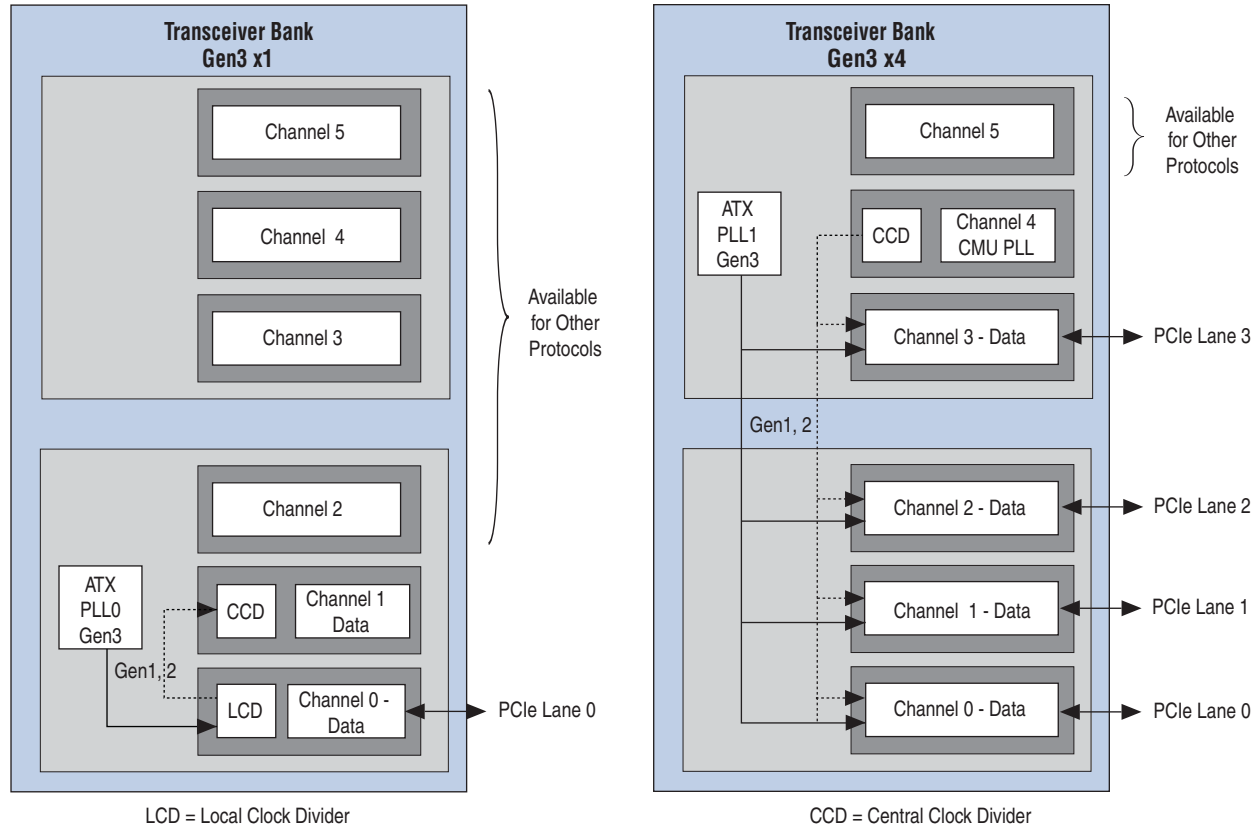
Figure 6-46. Channel Placement Gen3 \times 1 and \times 4
