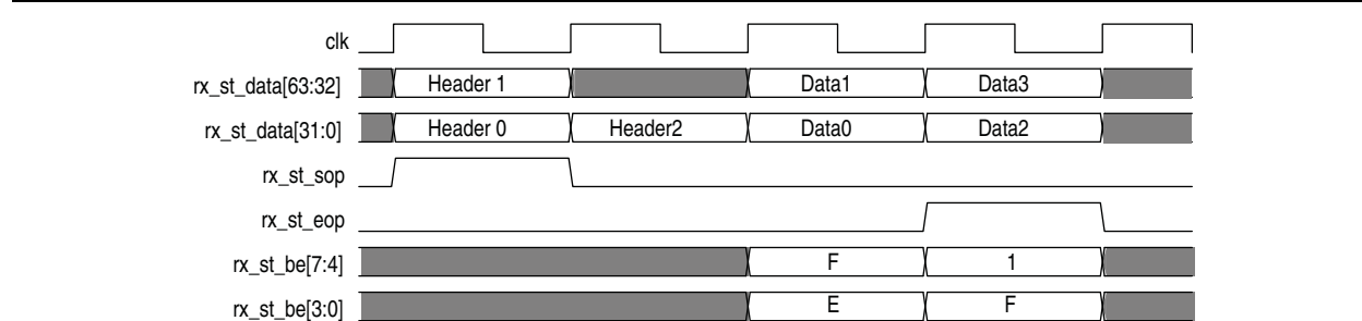
Figure 6-4. 64-Bit Avalon-ST rx_st_data<n> Cycle Definition for 3-Dword Header TLPs with Qword Aligned Address (1)
