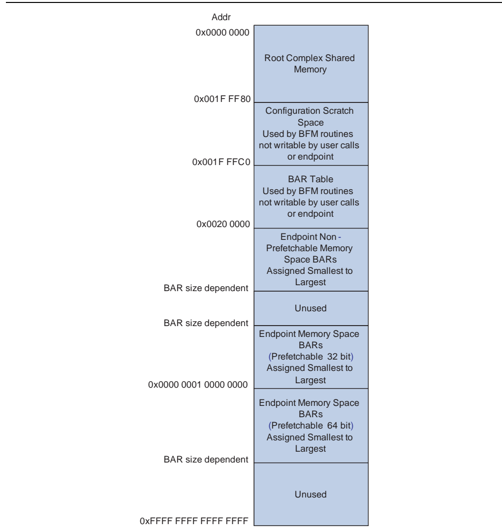
Figure 15-6. Memory Space Layout—No Limit
