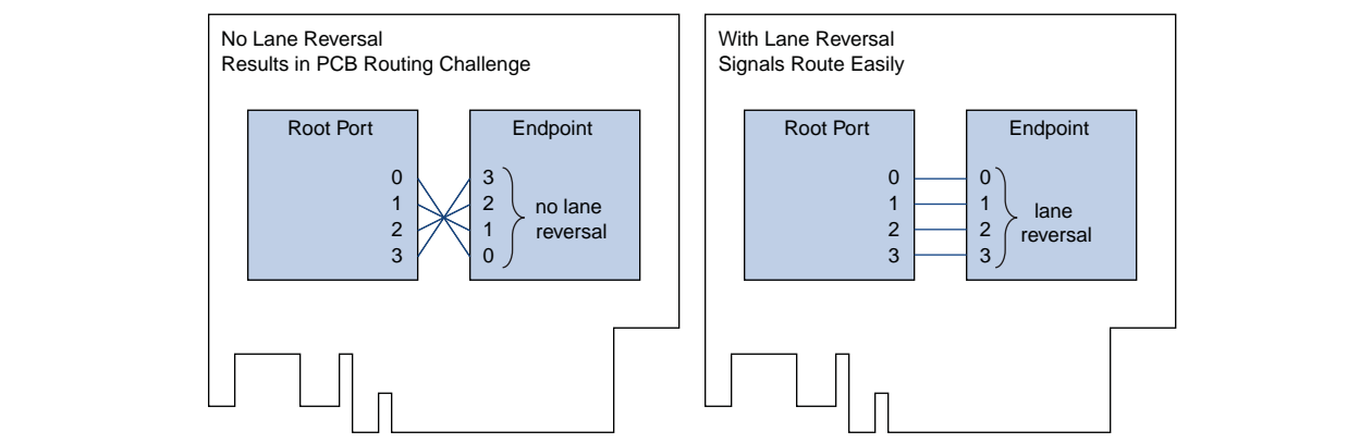
Figure 10-2. Using Lane Reversal to Solve PCB Routing Problems
