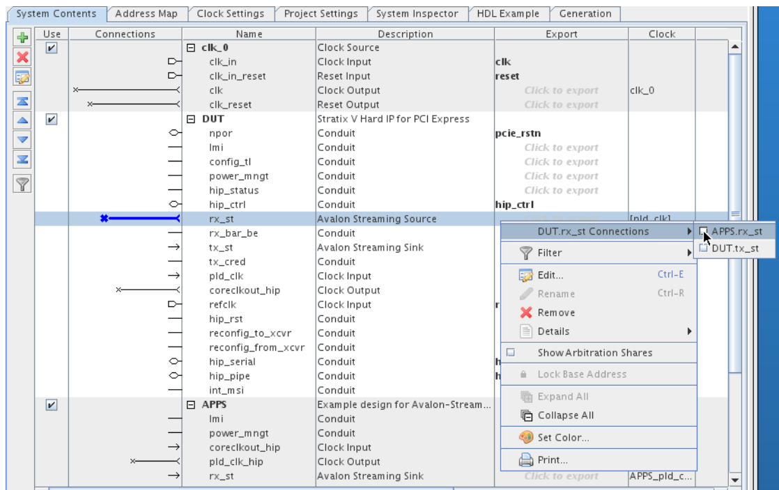
Figure 2-7. Connecting Signals Using the Right-Mouse Connections Menu
