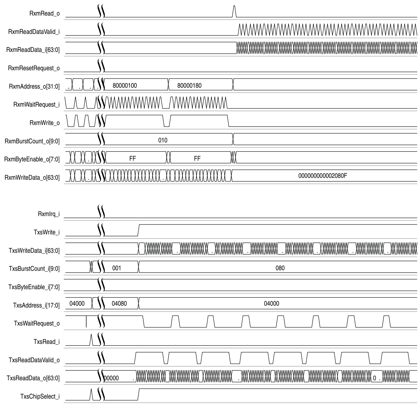
Figure 6-40. Simultaneous DMA Read, DMA Write, and Target Access
