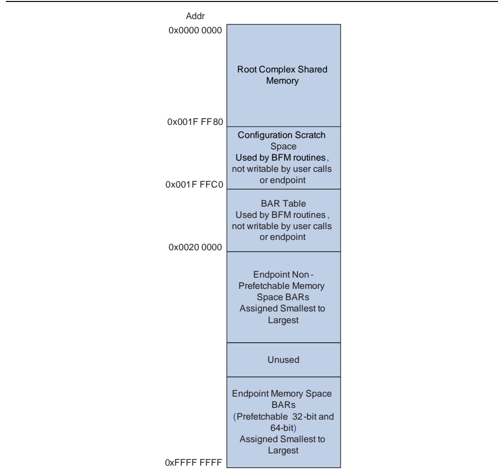
Figure 15-5. Memory Space Layout—4 GByte Limit
