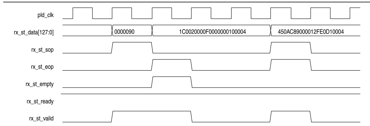
Figure 6-15. 128-Bit Packet Examples of rx_st_empty and Single-Cycle Packet
