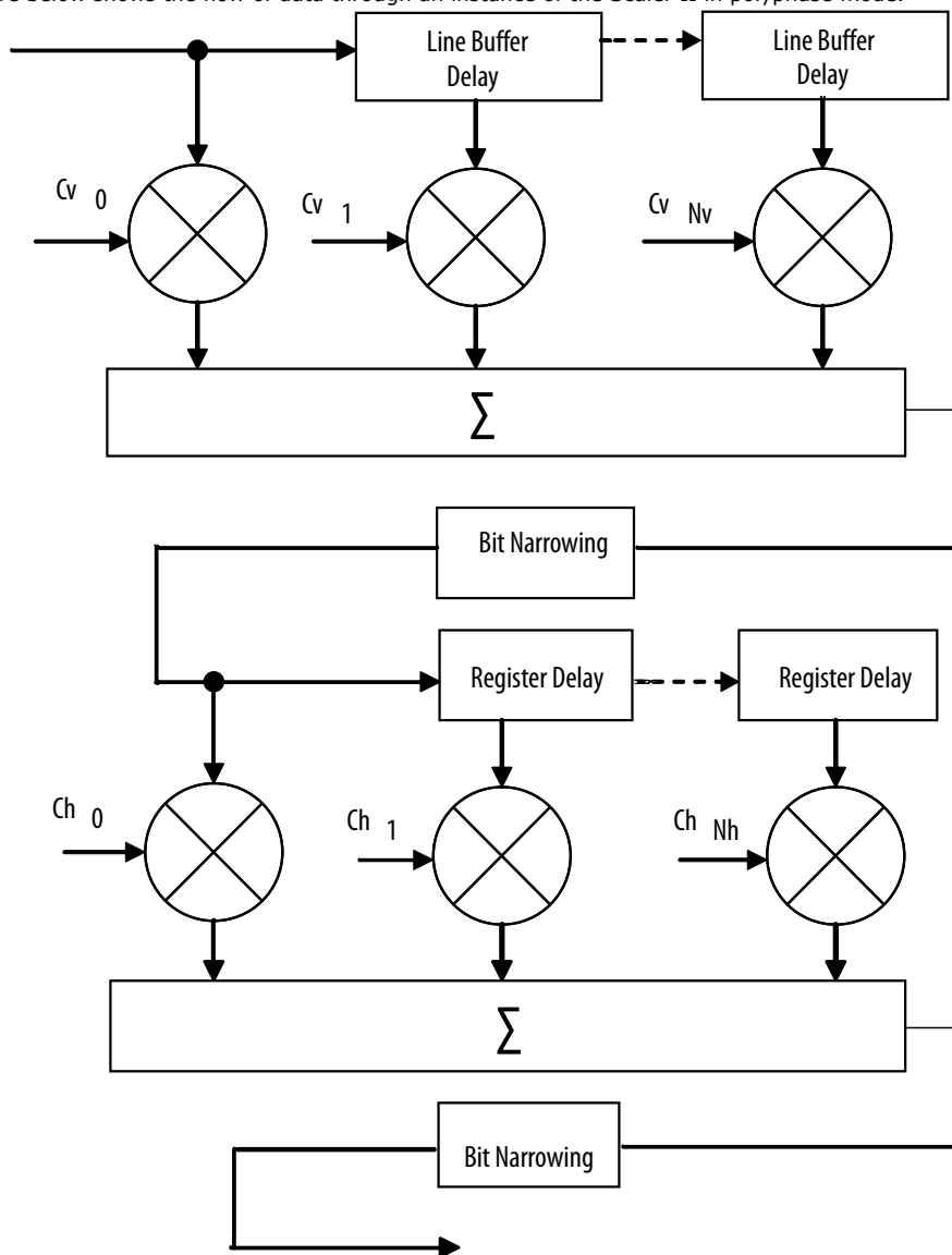
Figure 69. Polyphase Mode Scaler Block Diagram
