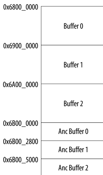
Figure 67. Example of Memory Map for Base Address 0x6800_0000
