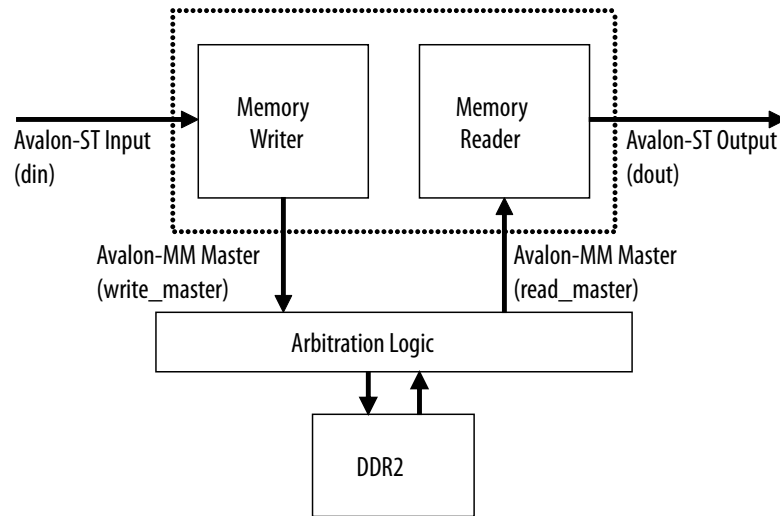
Figure 66. Frame Buffer Block Diagram
