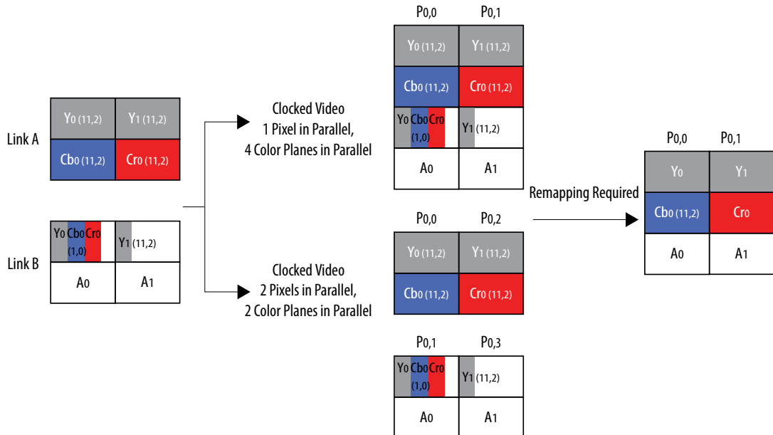
Figure 31. Clocked Video Input Interpretations of SMPTE-372 Dual Link 12-bit YCbCr Mapping
