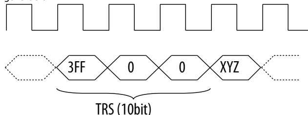
Figure 12. Time Reference Signal Format
