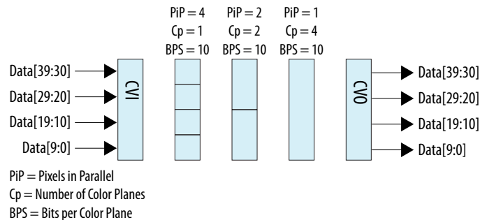
Figure 20. Variable Interpretation of Pixels on a Clocked Video Data Bus Based on Parameterization
