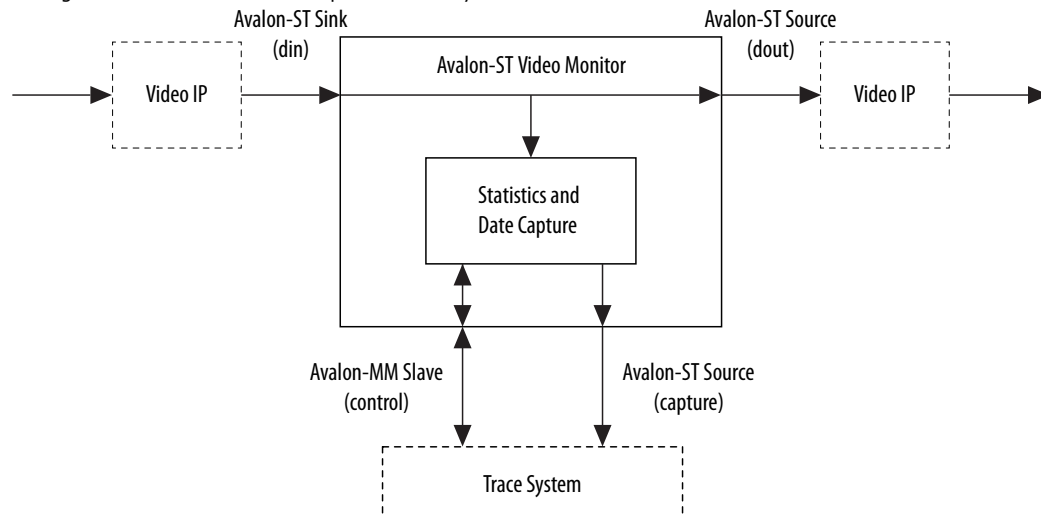
Figure 75. Avalon-ST Video Monitor Functional Block Diagram
