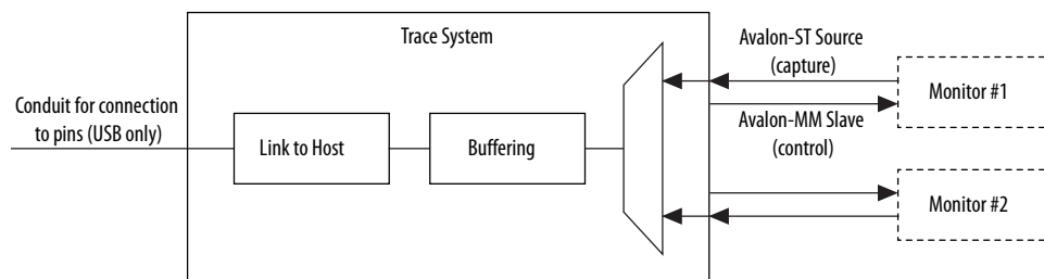
Figure 73. Trace System Functional Block Diagram
