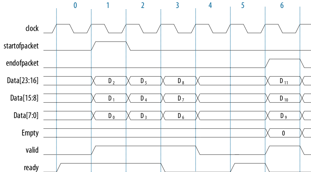
Figure 2. Avalon-ST Video Packet Transmission (Symbols in Parallel)
