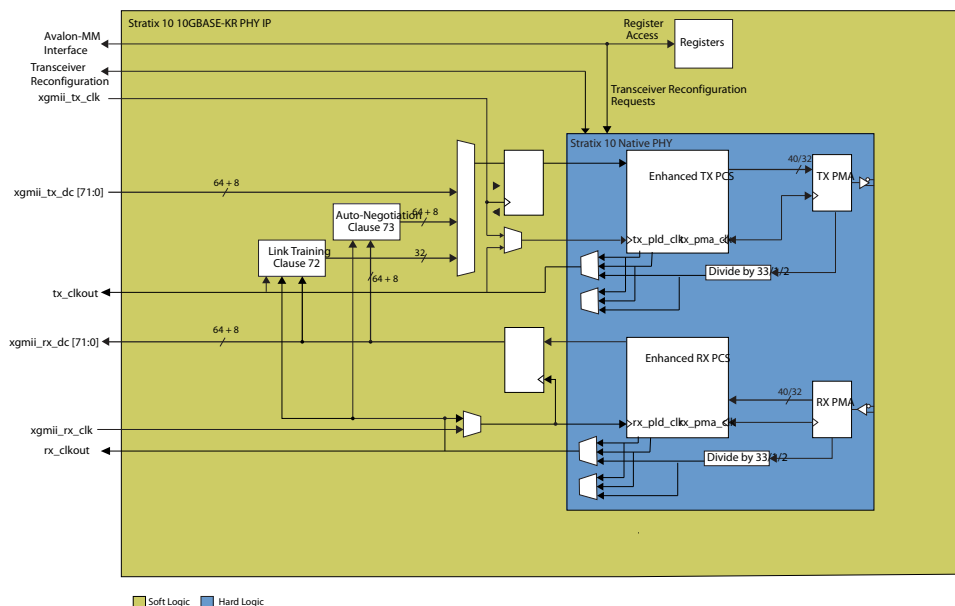
Figure 1. Intel Stratix 10 10GBASE-KR Block Diagram
