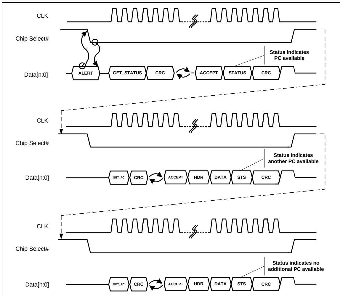
Figure 31: Pipelined Back-to-Back Bus Mastering Posted Write Transactions
