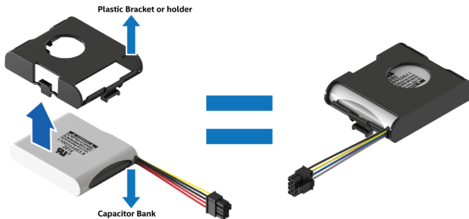
Figure 21 - AXSRMFBU7 Mounting Assembly
