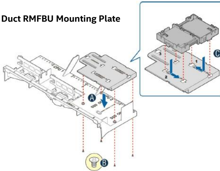
Figure 22 - RMFBU Assembly Installation
