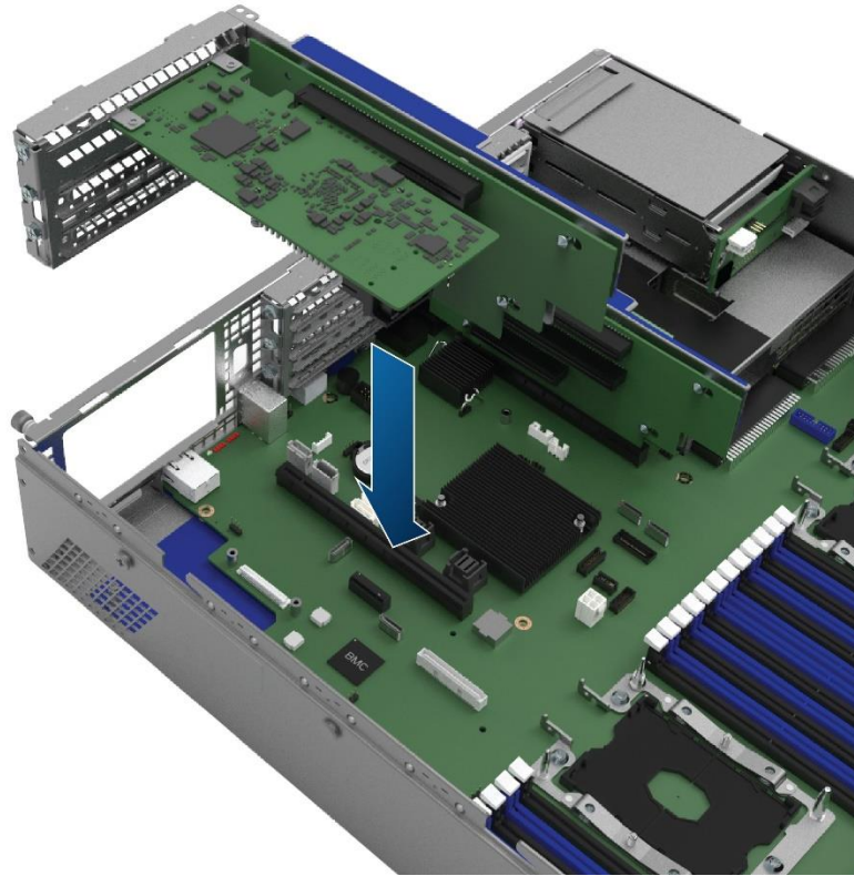
Figure 17 RAID Adapter Installation (insert riser card)
