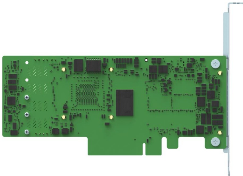
Figure 3 - Intel SAS RSP3DD080F RAID adapter Layout
