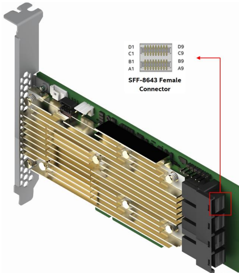
Figure 9. Intel® RSP3TD160F RAID Adapter SFF-8643 connector
