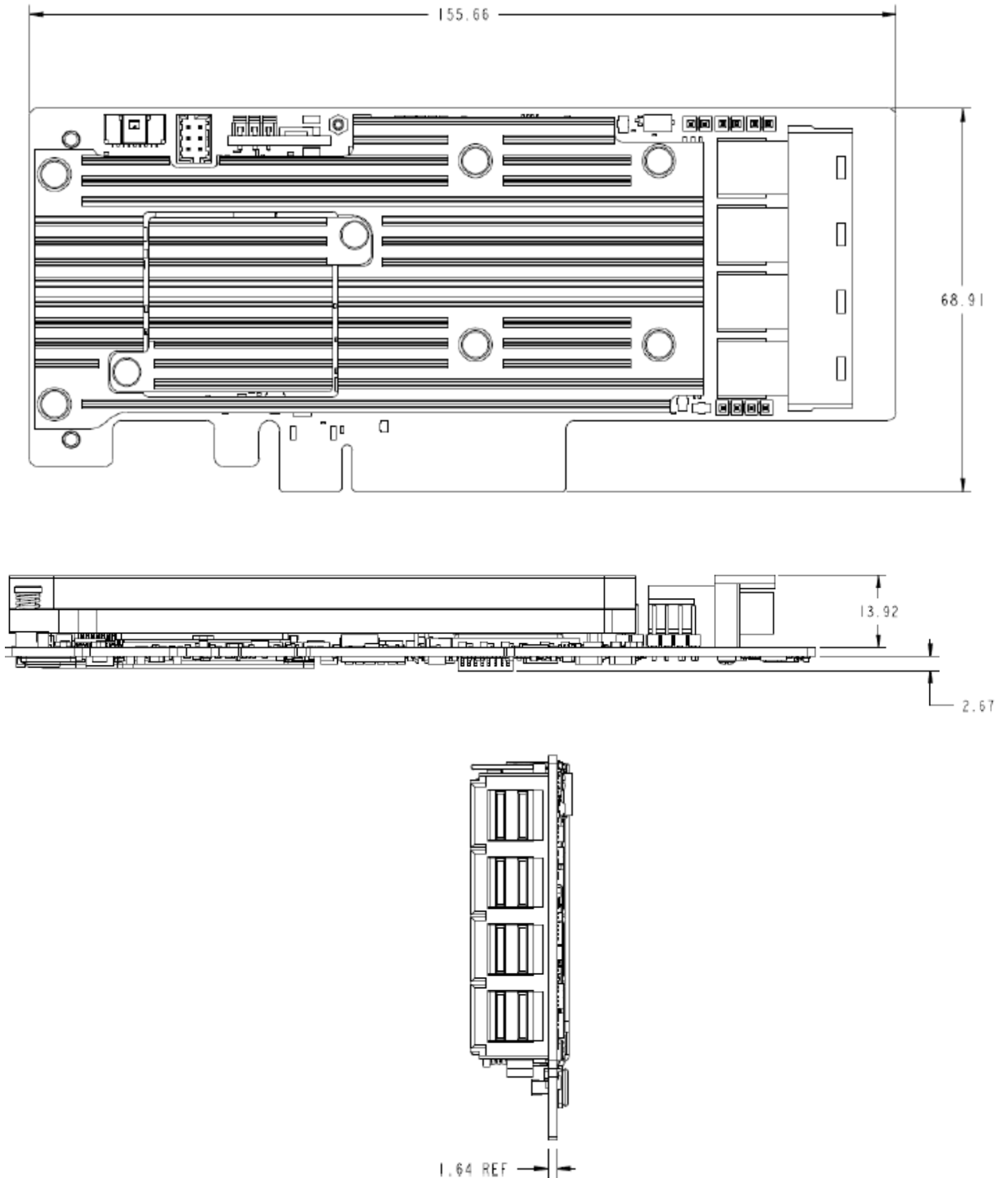
Figure 2 - Intel RSP3TD160F RAID adapter Dimensions
