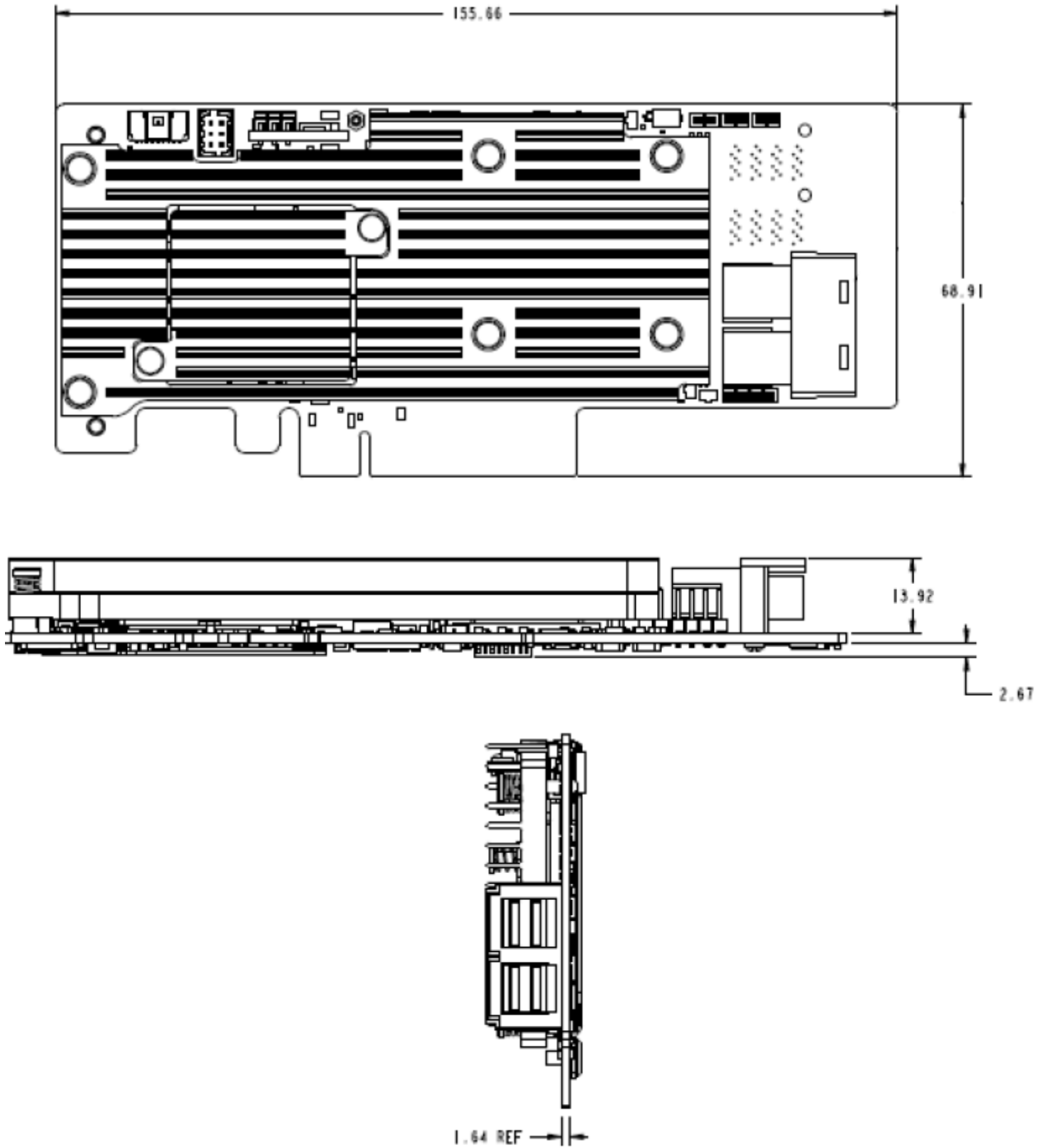
Figure 4 - Intel RSP3DD080F RAID adapter Dimensions
