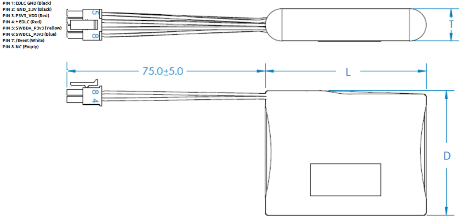
Figure 19. FBU345 layout
