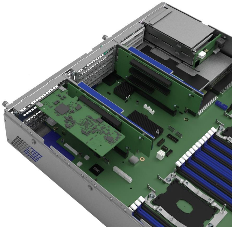
Figure 18 RAID Adapter Installation (adapter installed)
