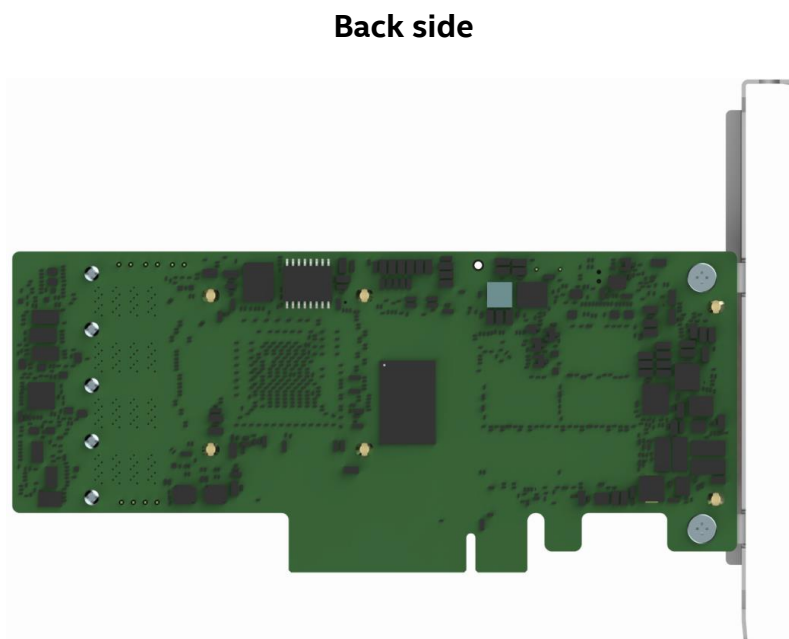
Figure 1 - Intel SAS RSP3TD160F RAID adapter Layout
