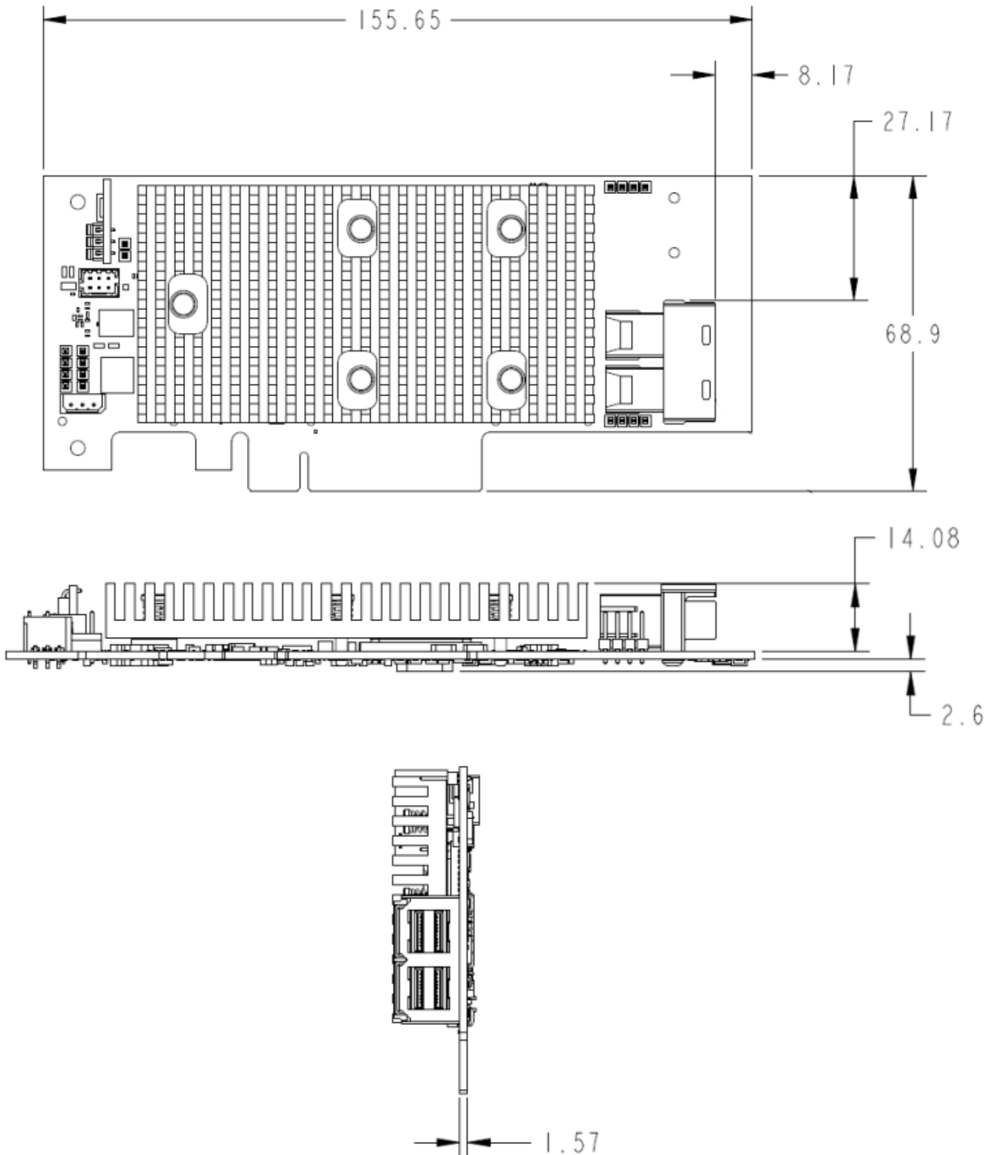
Figure 8 - Intel RSP3WD080E RAID adapter Dimensions
