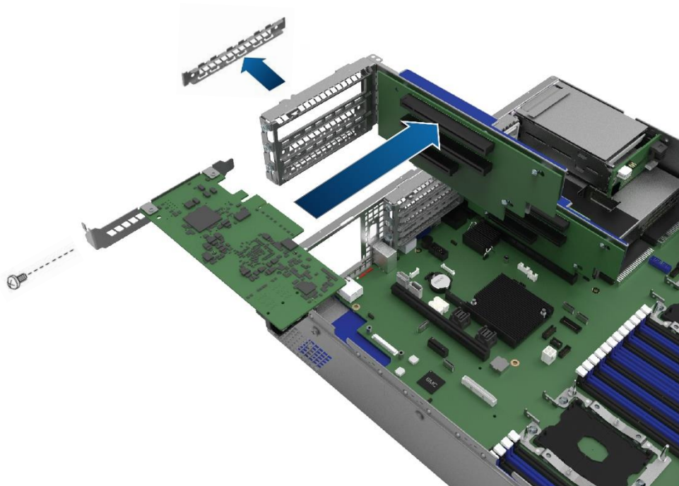
Figure 16 RAID Adapter Installation (insert adapter in slot)
