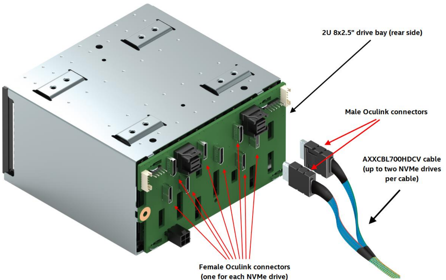
Figure 14. Connecting the AXXCBL700HDCV to the backplane
