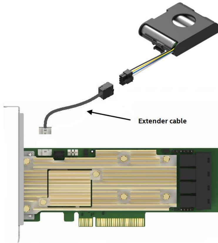
Figure 23 - Connecting the RMFBU7 to the RAID adapter
