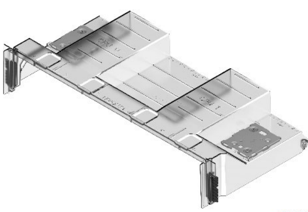
Standard Air Duct (Default) (2U processor heat sink configurations)
