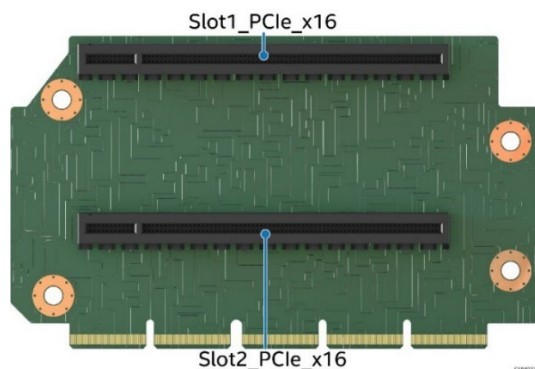
Figure 51. Two-slot PCIe* Riser Card for Riser Slot #2
