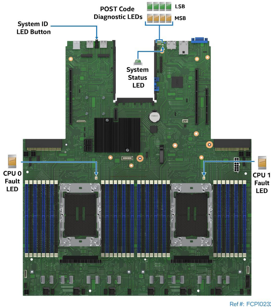
Figure 15. Intel® Light-Guided Diagnostics – LED Identification
