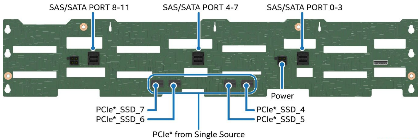
Figure 88. 12 x 3.5" HSBP Connector Identification – Back Side
