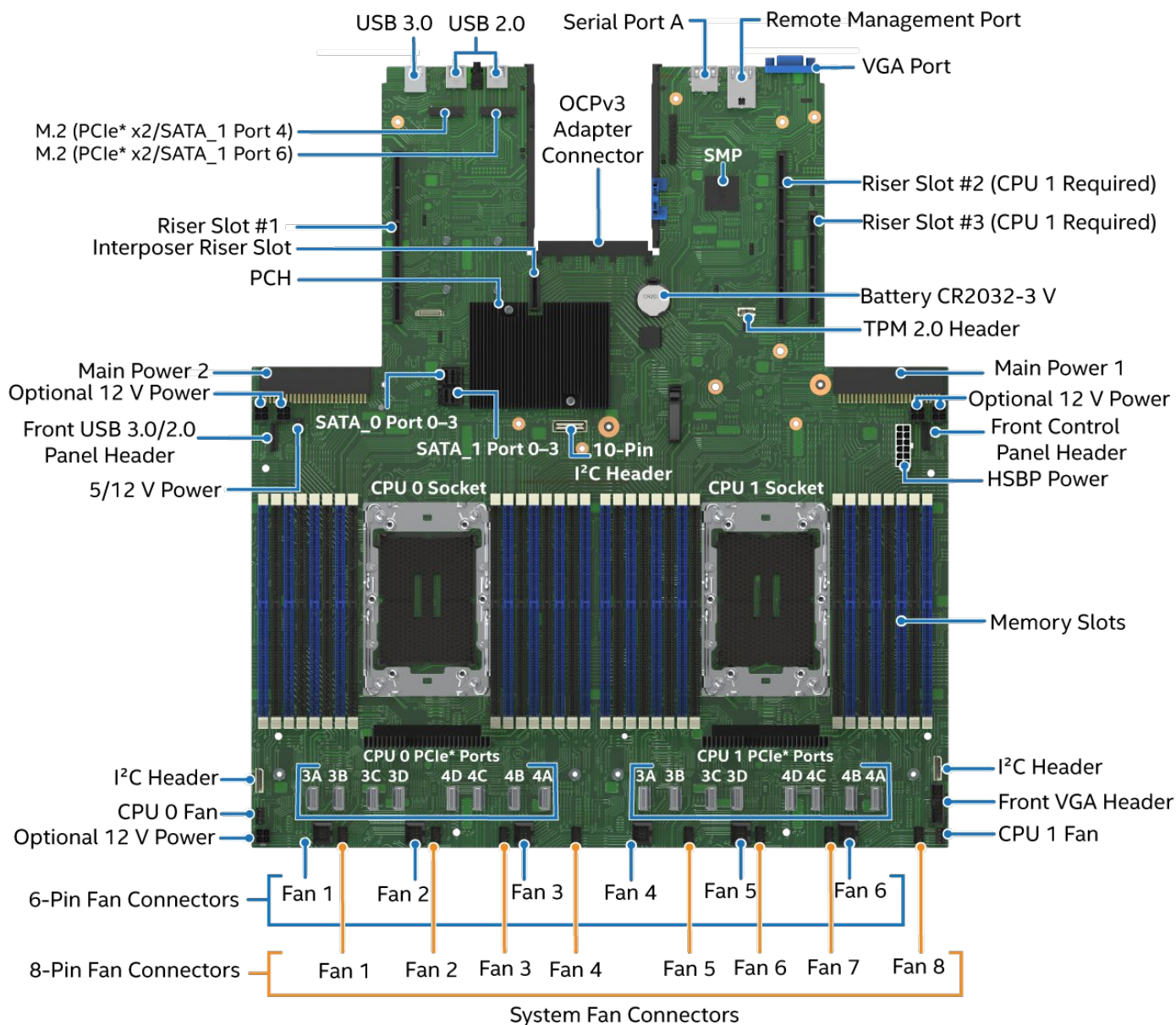
Figure 14. Intel® Server Board M50FCP2SBSTD Component / Feature Identification
