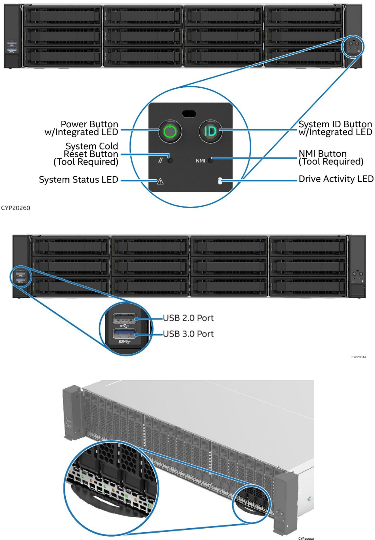
Figure 12. Front Panel Feature Identification
