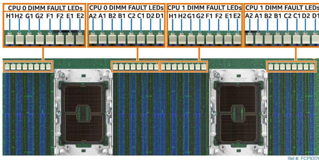
Figure 103. Memory Fault LED Location
