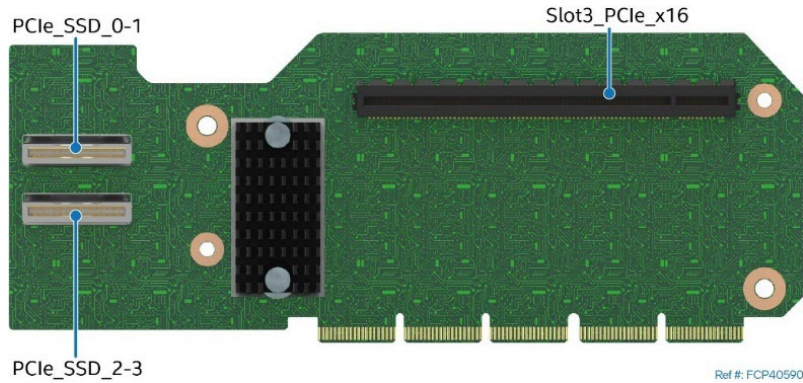
Figure 82. PCIe® NVMe® Riser Card for Riser Slot #1
