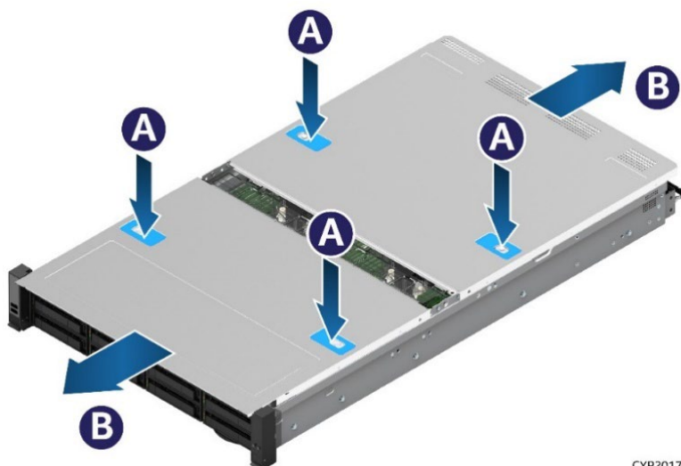
Figure 24. System Top Cover Removal
