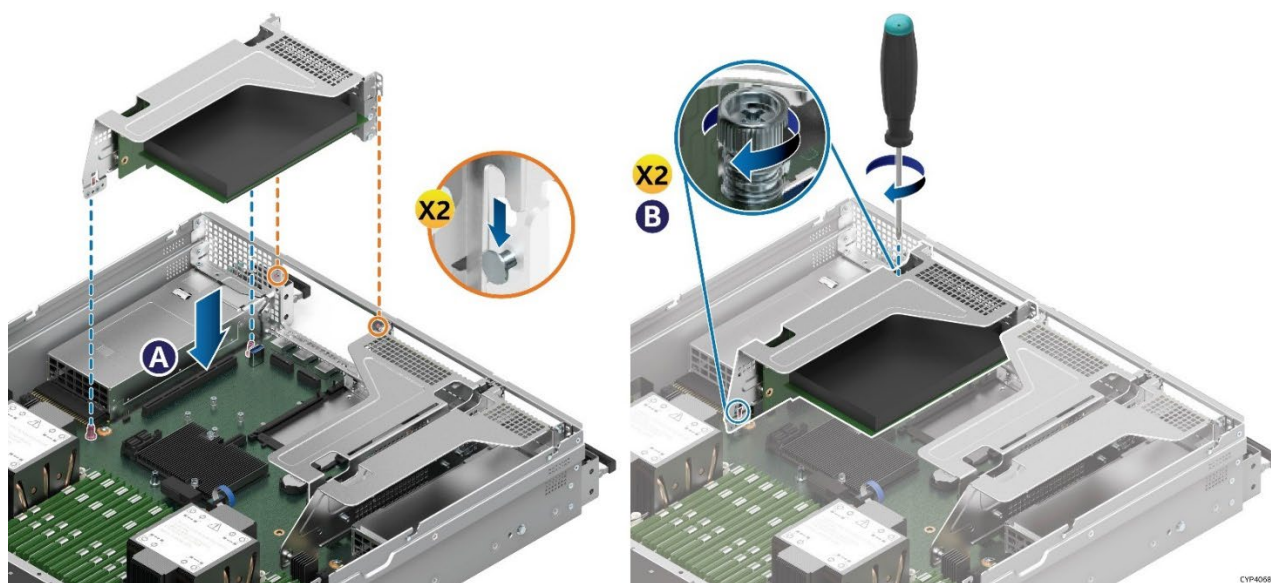
Figure 45. Riser Card Assembly Installation
