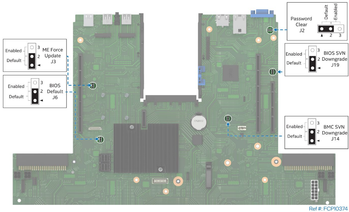
Figure 17. System Configuration and Recovery Jumpers
