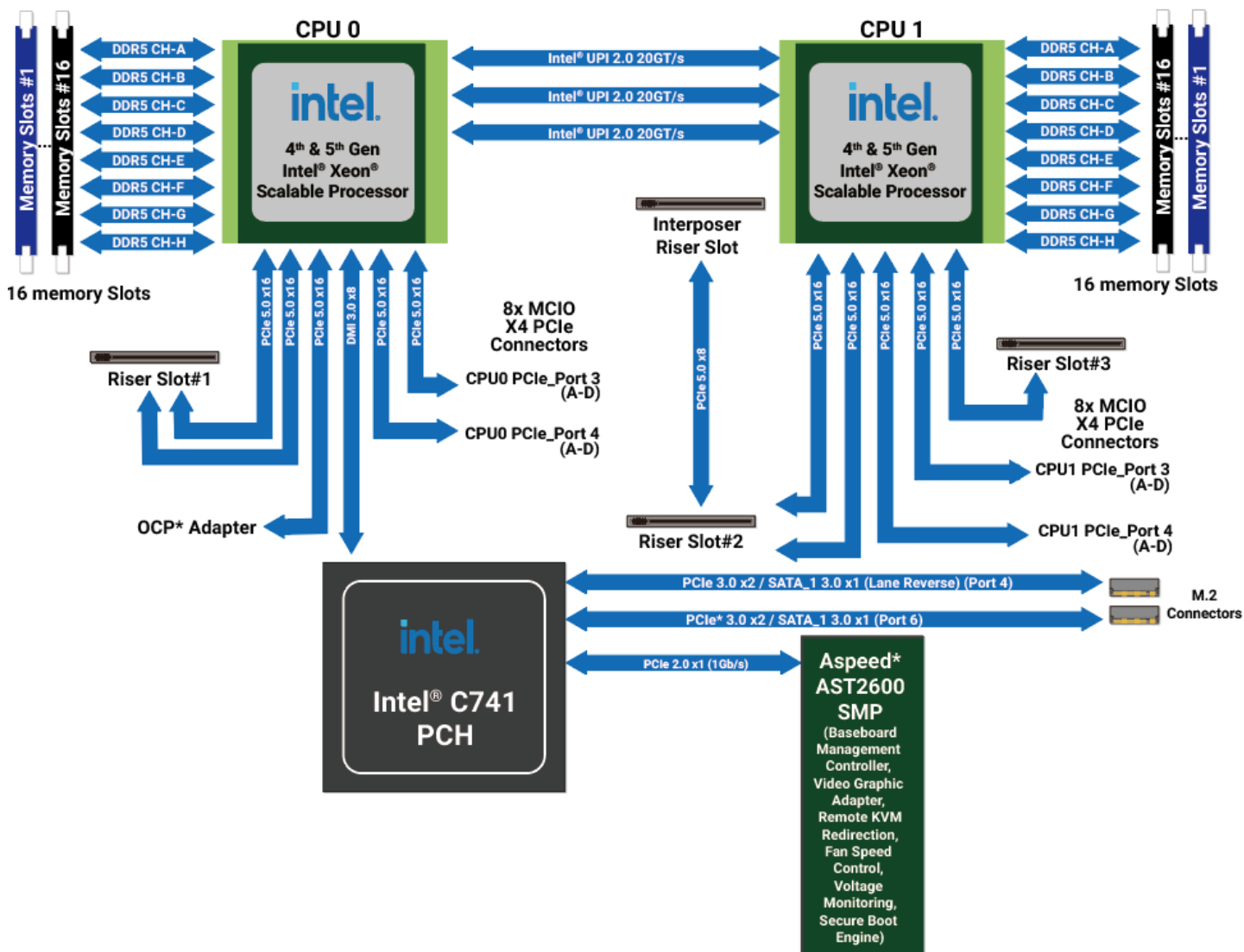
Figure 13. Intel® Server Board M50FCP2SBSTD Architectural Block Diagram
