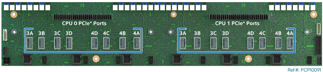
Figure 80. PCIe* MCIO Connectors
