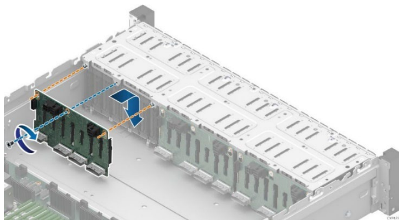
Figure 69. 2.5" Backplane Placement
