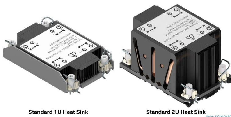
Figure 36. Supported Processor Heat Sinks
