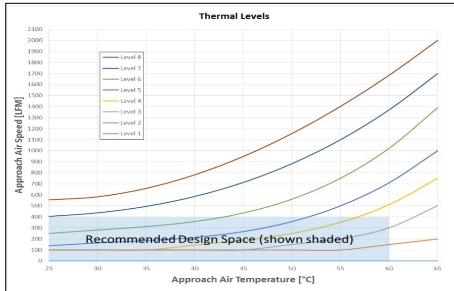
Figure 115. PCIe SIG Add-in cards thermal levels
