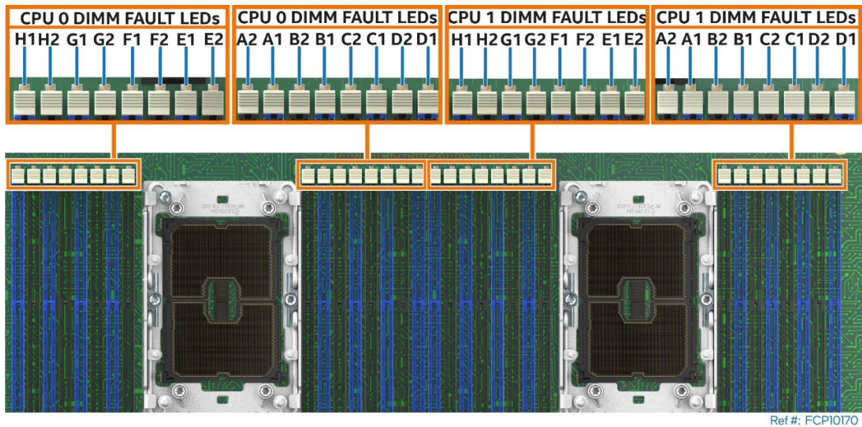
Figure 16. Intel® Light-Guided Diagnostics – Memory Fault LEDs
