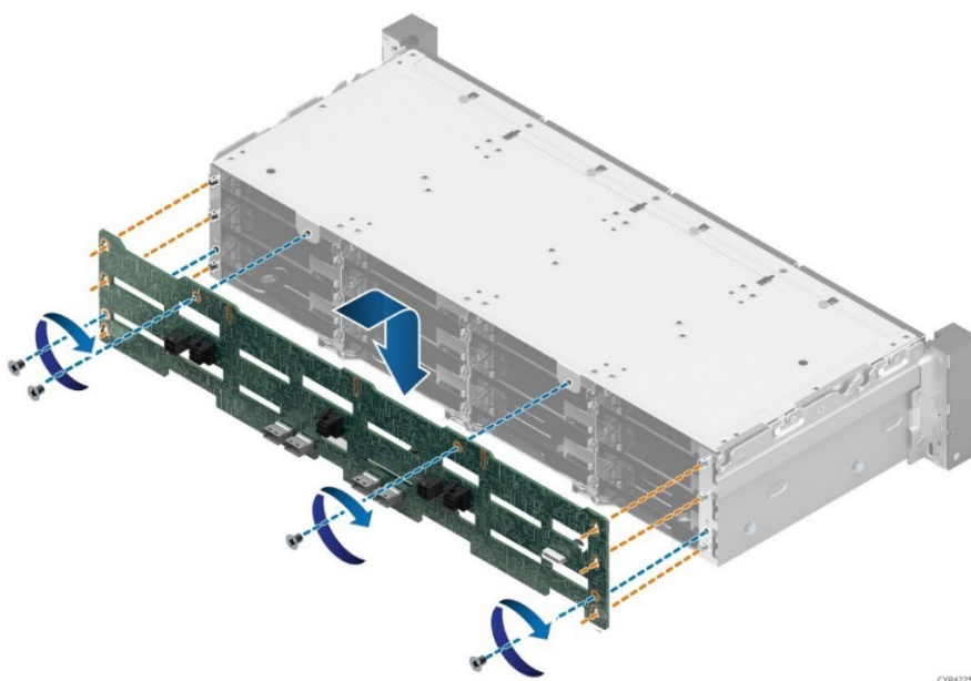
Figure 76. 3.5" Backplane Placement
