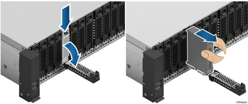
Figure 61. 7-mm Drive Removal from 2.5" Drive Bay
