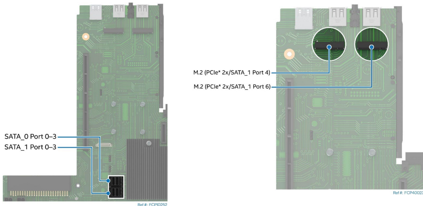
Figure 89. Onboard SATA Cable Connectors and M.2 SSD Connectors
