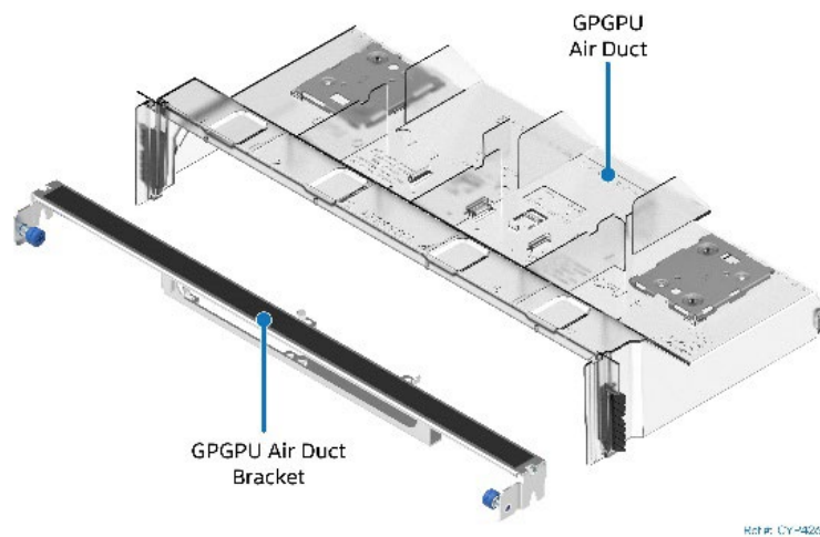
GPGPU Air Duct option (iPN - FCPGPGPUKit) (1U processor heat sink + GPGPU configurations)
