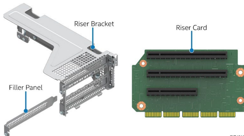
Figure 44. Riser Card Assembly Components
