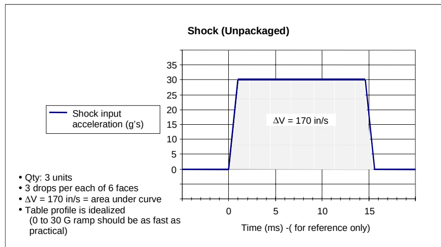
Figure 5. Unpackaged system shock input
