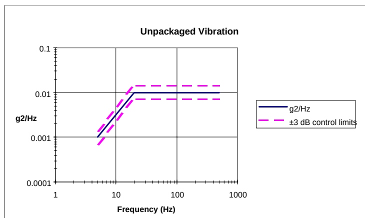
Figure 6. Unpackaged system vibration test input
