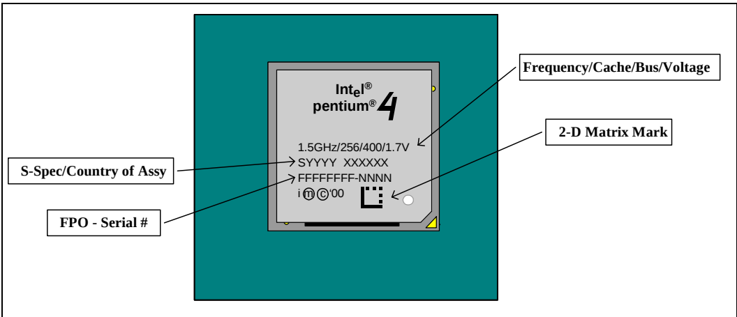
Figure 21. Processor Markings
