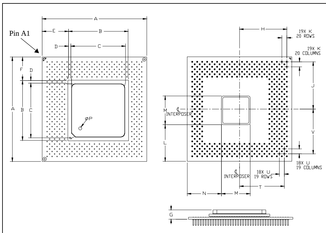
Figure 17. Processor Package
