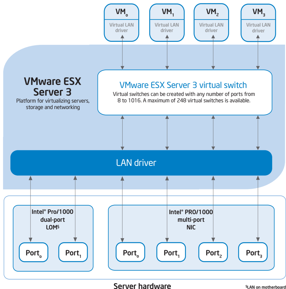
Figure 3. Recommended network configuration for Intel® architecture–based servers with VMware ESX Server* virtual machine monitor installed. ESX Server takes ownership of two ports for security, availability, and segmentation. The remaining ports are then available to virtual machine traffic.
