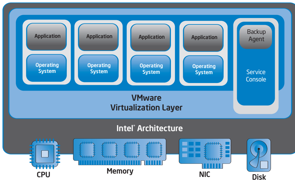
Figure 1. VMware Infrastructure 3* enables enterprises to create a virtual infrastructure, which provides a layer of abstraction between the computing, storage, and networking hardware and the software that operates on it. With a virtual infrastructure, users see resources as if the resources were dedicated to them. The administrator manages and optimizes resources transparently across the data center.
