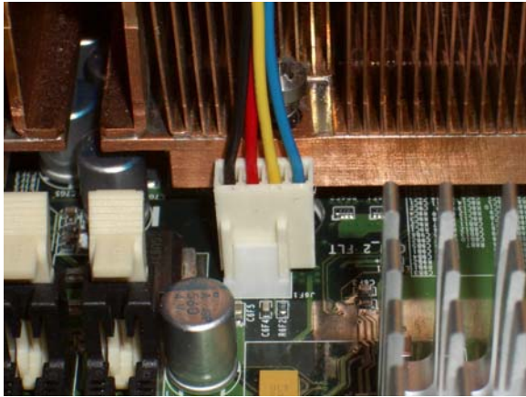
Figure 2. Processor 1 Fan Header
