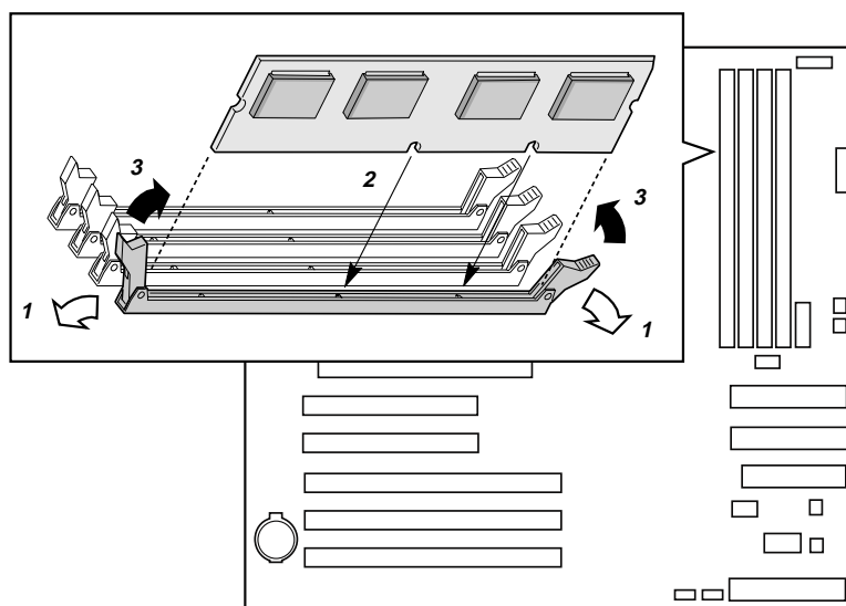
Figure 14. Installation de mémoire
