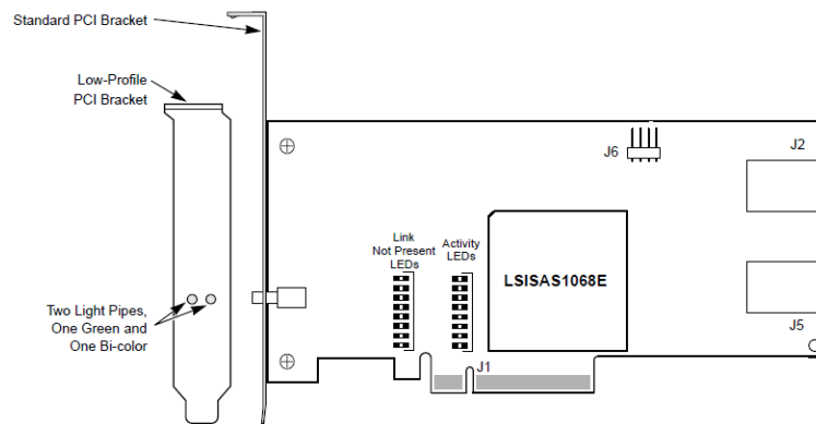
Figure 4. Card Layout
