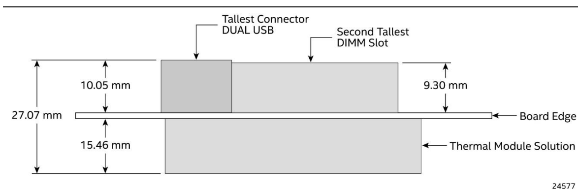
Figure 18. Board Height Dimensions
