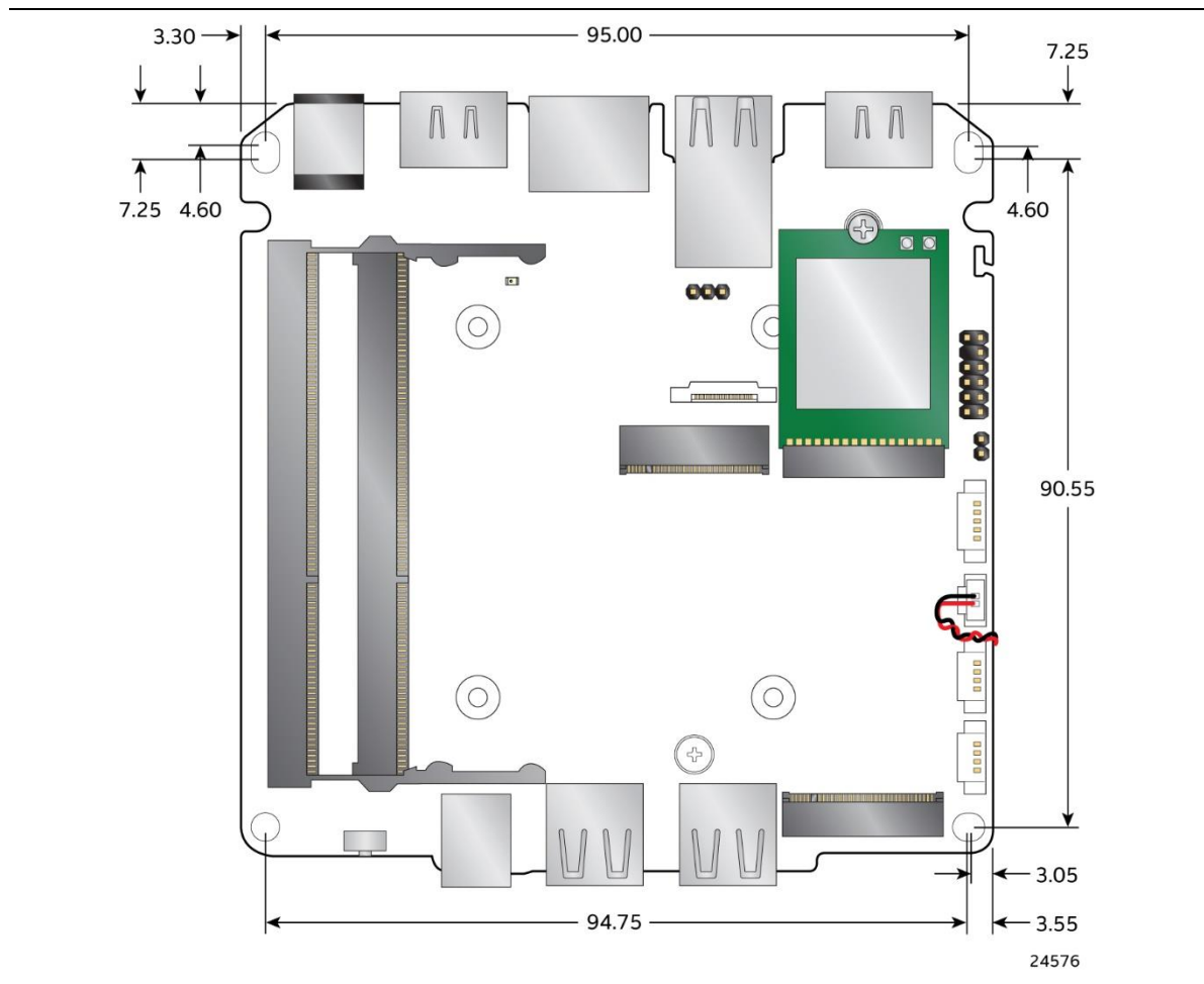
Figure 17. Board Dimensions
