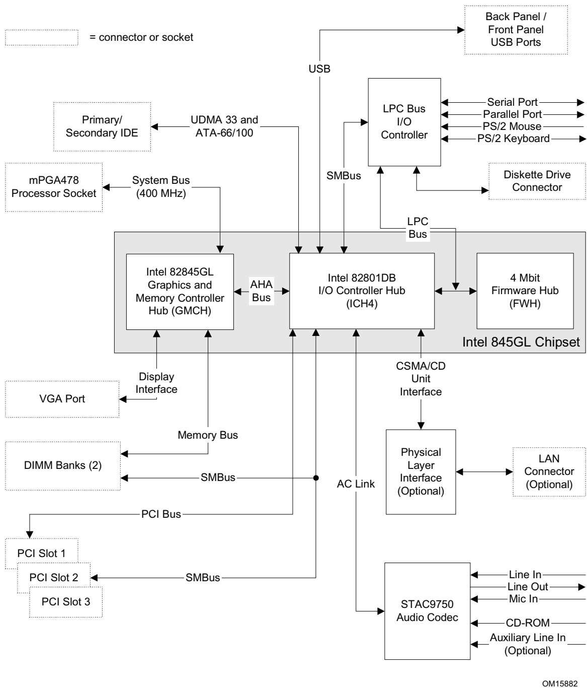
Figure 2. Block Diagram
