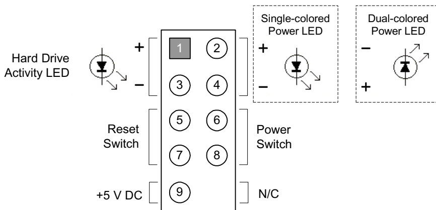
Figure 8. Connection Diagram for Front Panel Connector
