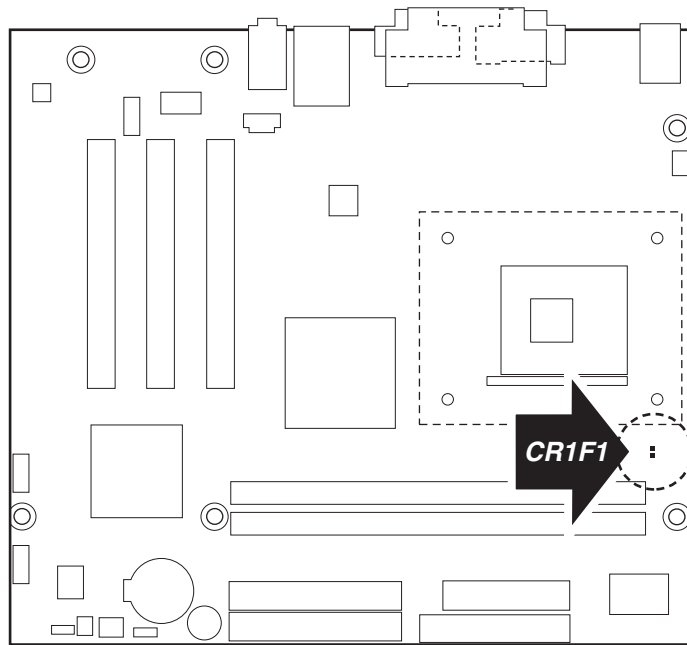
Figure 3. Location of the Standby Power Indicator LED on the D845GLVA Board
