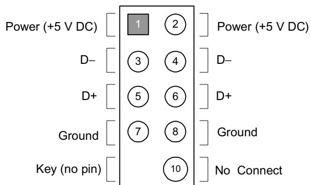
Figure 9. Connection Diagram for Front Panel USB Connector
