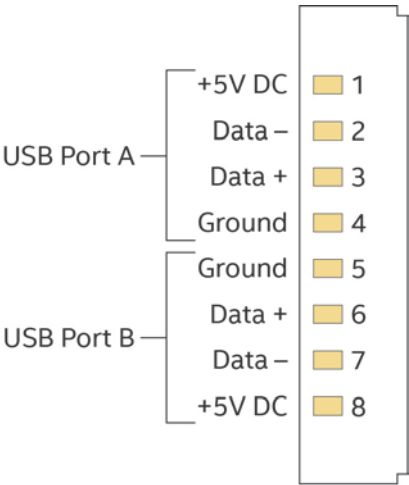
Figure 16. Connection Diagram for Internal USB 2.0 Dual-Port Header (1.25 mm Pitch)
