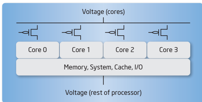
Figure 3. Integrated Power Gates enable idle cores to go to near-zero power independently.
