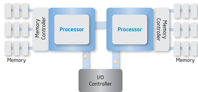
Figure 2. Intel® QuickPath Technology with dedicated per-processor memory and point-to-point connectivity.
