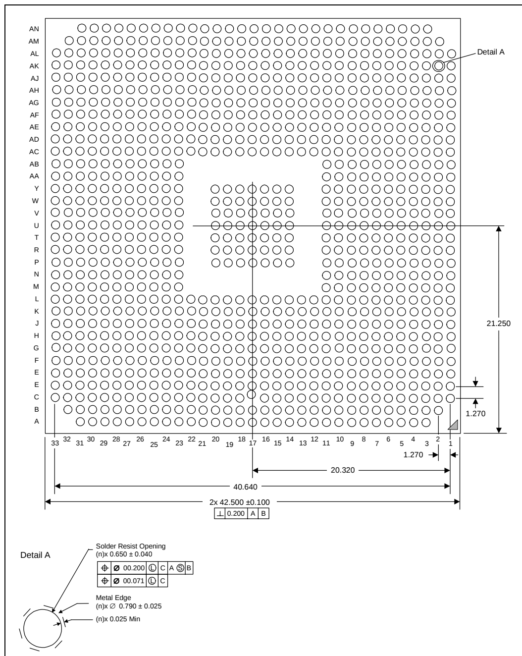
Figure 7-4. MCH Package Dimensions (Top View)
