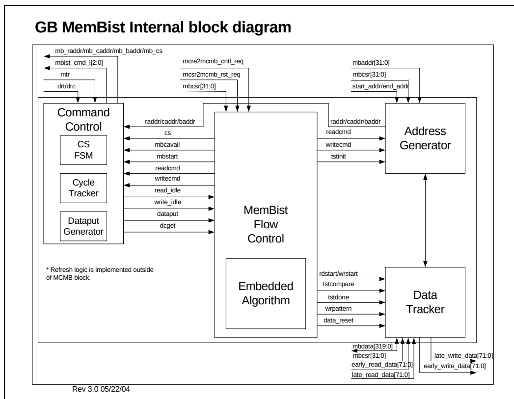
Figure 11-6. MemBIST Block Diagram
