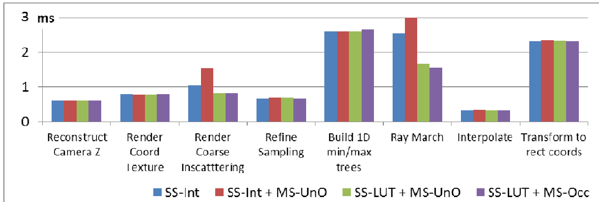
Figure 8. Performance of different stages of the algorithm on Intel HD graphics 5000 (1280x720 resolution).
