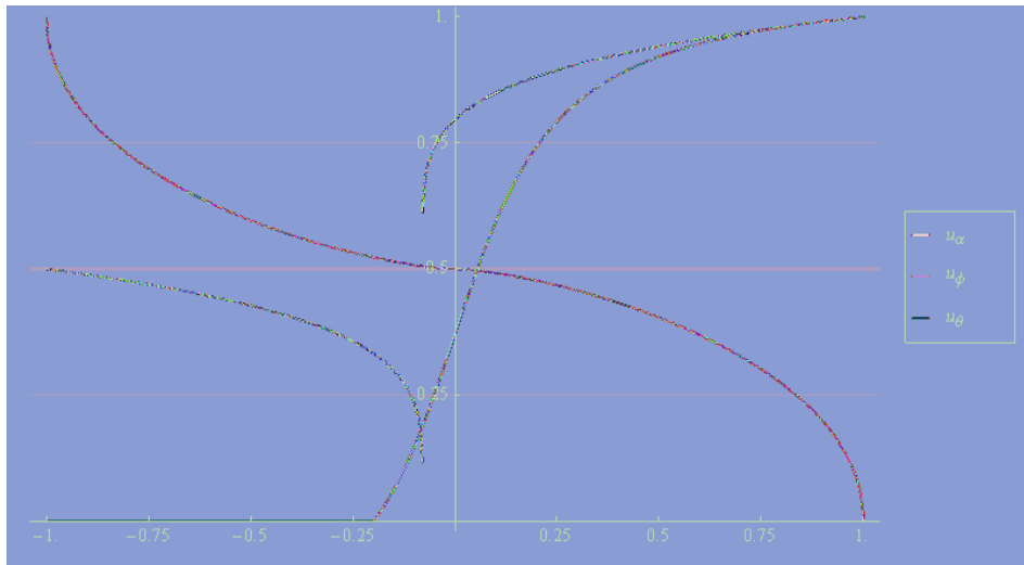
Figure 3. Non-linear parameterization.
