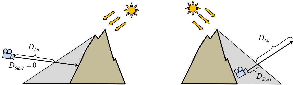
Figure 6. Total length D_{Lit} of the illuminated ray fraction and distance D_{Start} to the first lit point.
