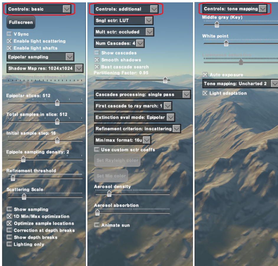
Figure 4. Left to right: basic, additional and tone mapping control sets.
