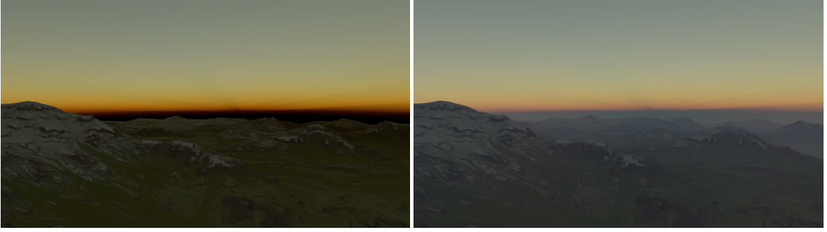
Figure 1. Twilight sky rendered with single scattering (left) and multiple scattering (right).
