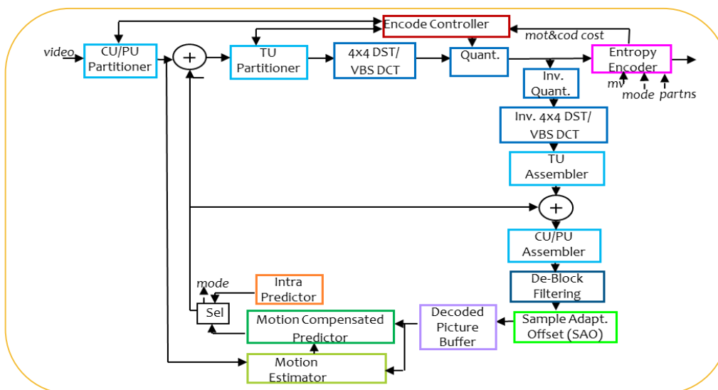
Figure 4 HEVC Encoder
