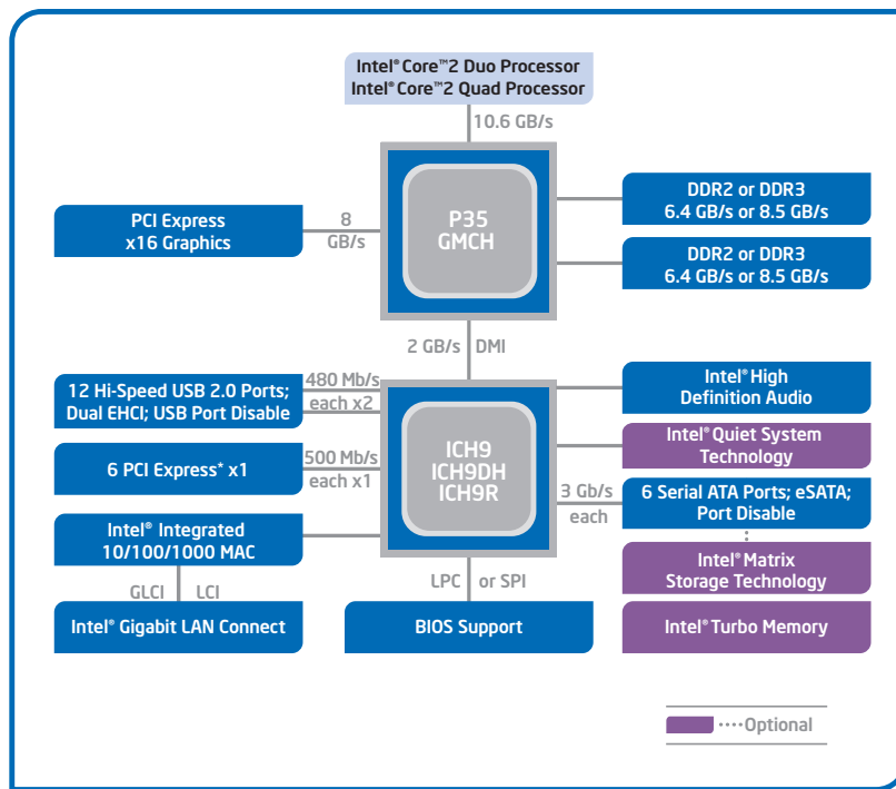
Intel® P35 Express Chipset Block Diagram
