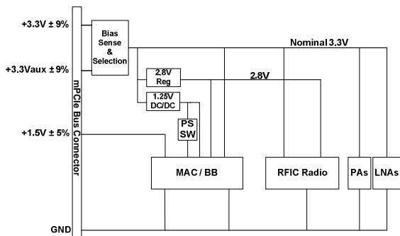
Figure 7: Bias network on the Intel PRO/Wireless 3945ABG Network Connection card
