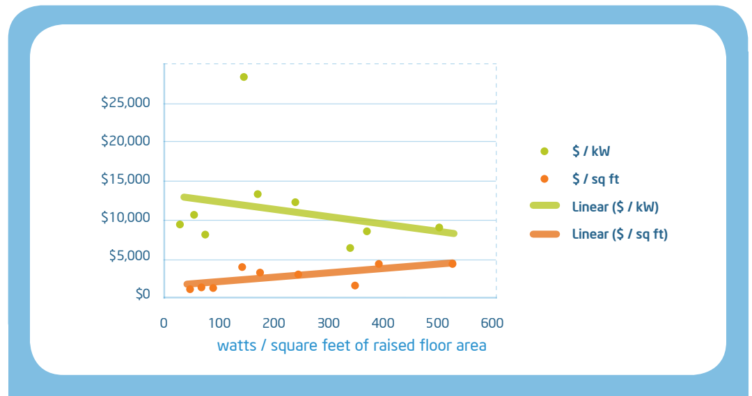
Figure 6. Data center cost metrics as a function of data center density
