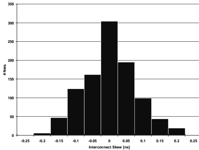
Figure 26. Monte Carlo results for host clock skew.
