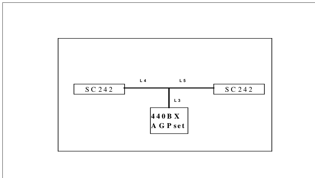
Figure 21. Recommended topology for dual processor design
