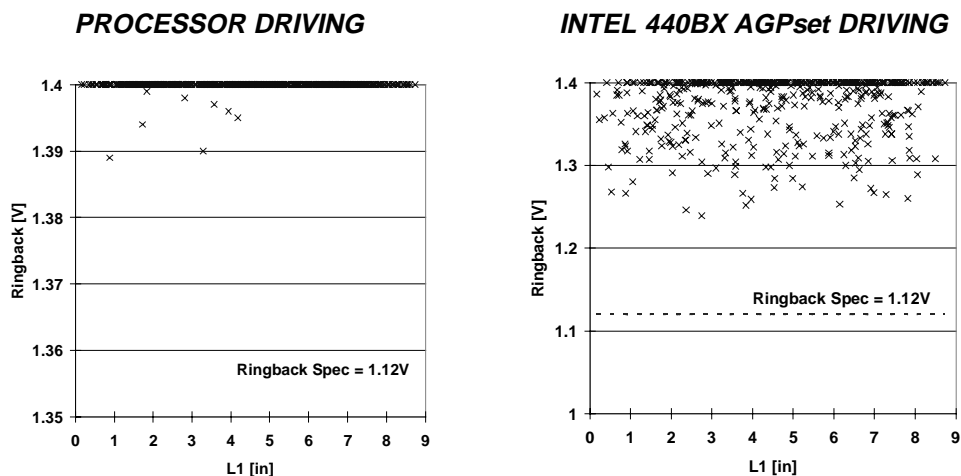
Figure 20. Monte Carlo signal quality for Uni-processor, based on parametric sweeps results
