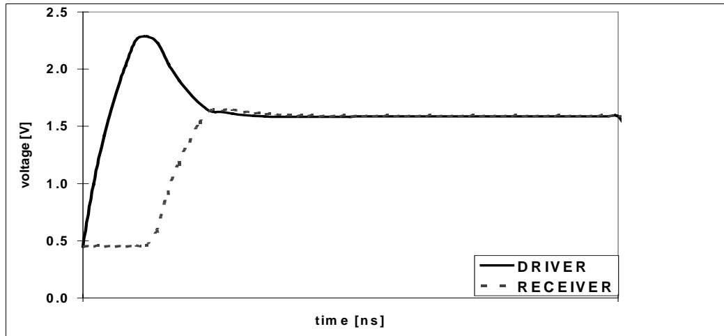
Figure 9. Waveform for the network in Figure 3 when driven with active pull-up
