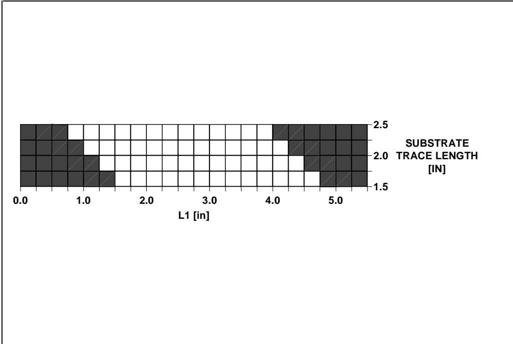
Figure 24. Solution space for single processor designs with single end termination (SET)
