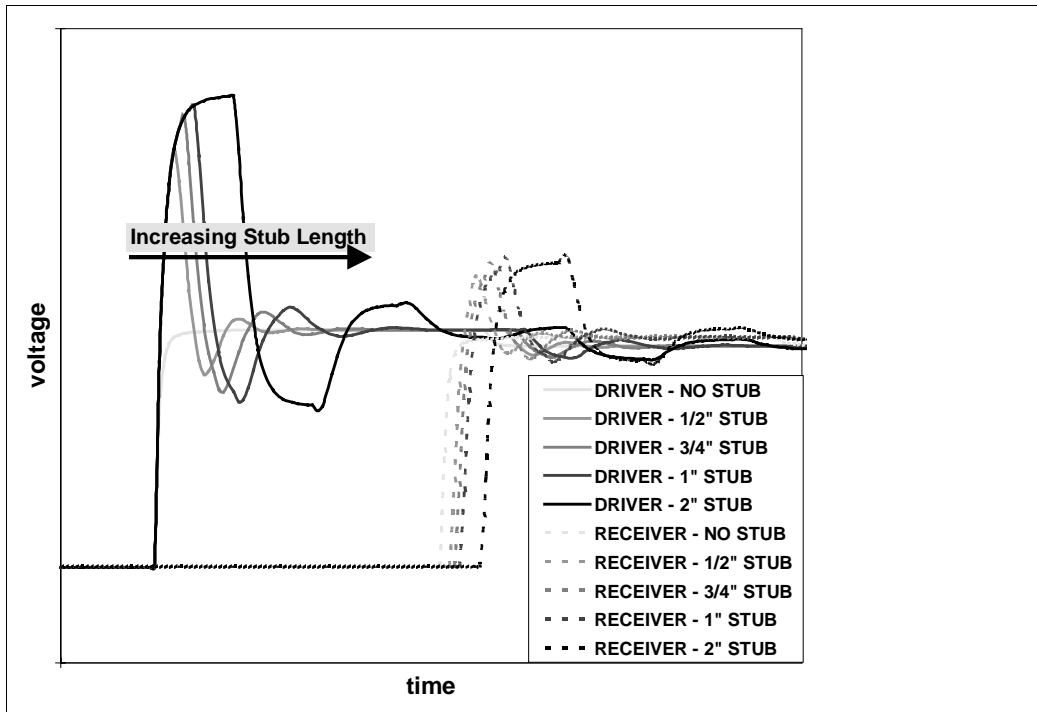
Figure 7. Ringing as a function of stub length for the network in Figure 3.
