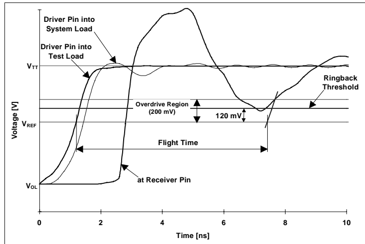
Figure 12. Flight time measurement with non-monotonic rising edge
