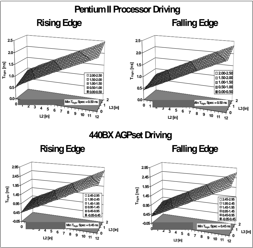
Figure 16. Parametric sweep minimum flight times for single processor design
