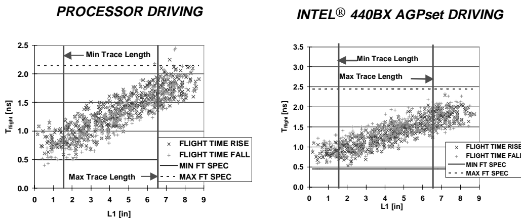
Figure 19. Monte Carlo flight times for Uni-processor, based on parametric sweeps results
