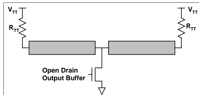
Figure 1. AGTL+ open drain buffer with external pull-up to V_{TT} .
