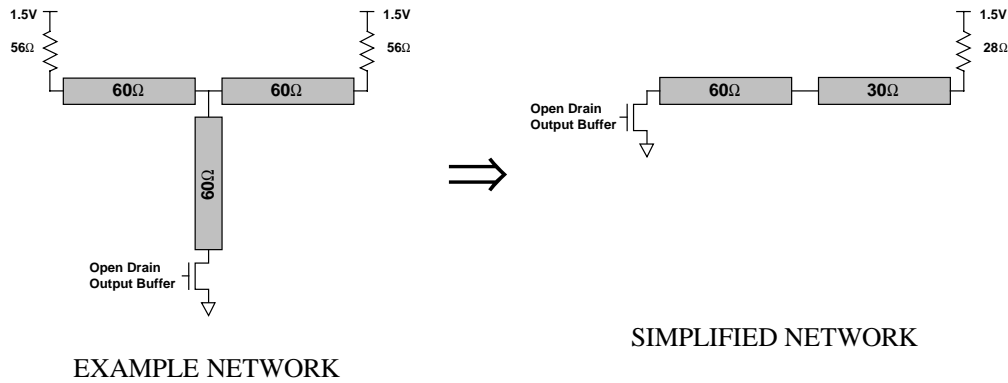
Figure 3. Example AGTL+ network.
