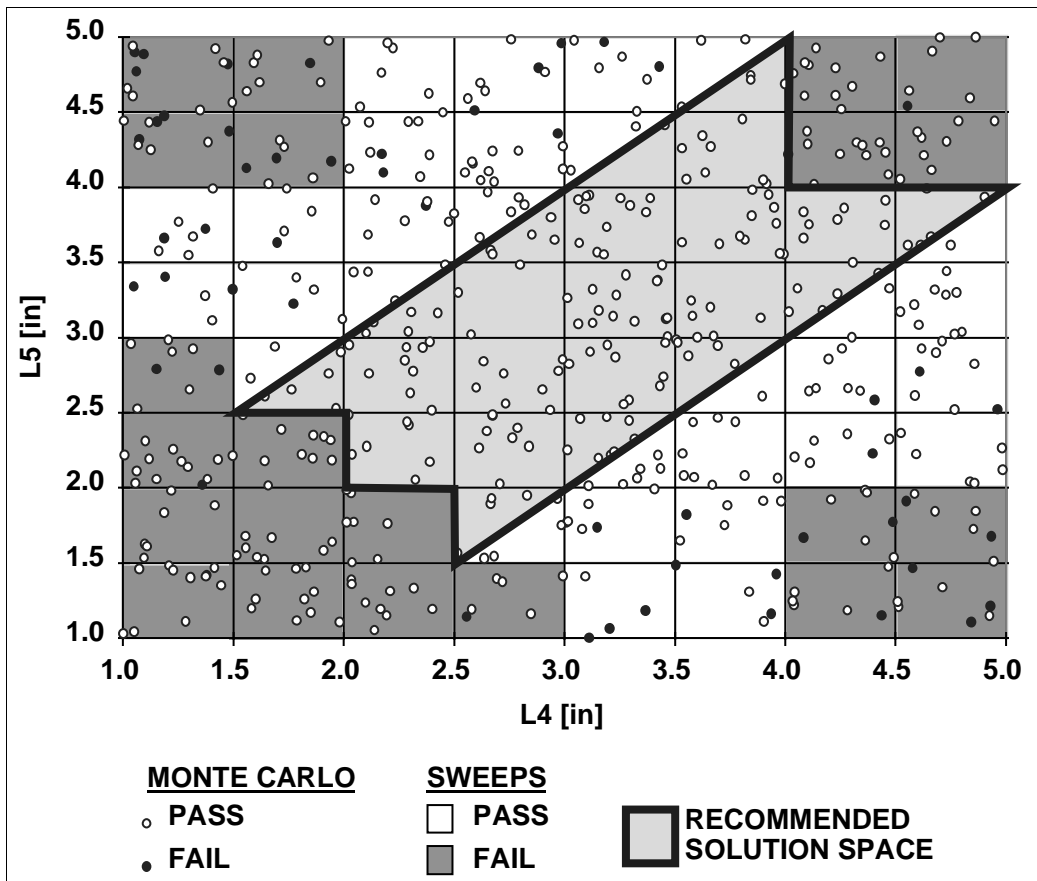
Figure 22. Dual processor solution space based on sweeps & Monte Carlo analysis
