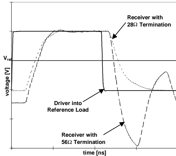
Figure 2. AGTL+ flight time dependence on R_{TT} .
