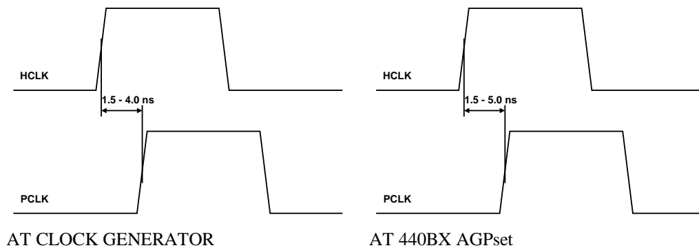
Figure 25. Host-to-PCI clock lag spec
