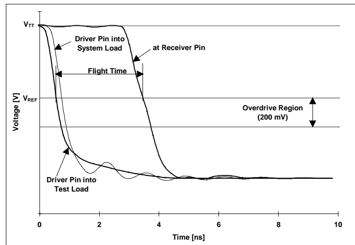
Figure 13. Example falling edge flight time measurement
