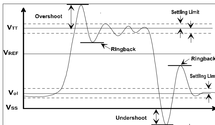
Figure 14. Overshoot, ringback, and settling time
