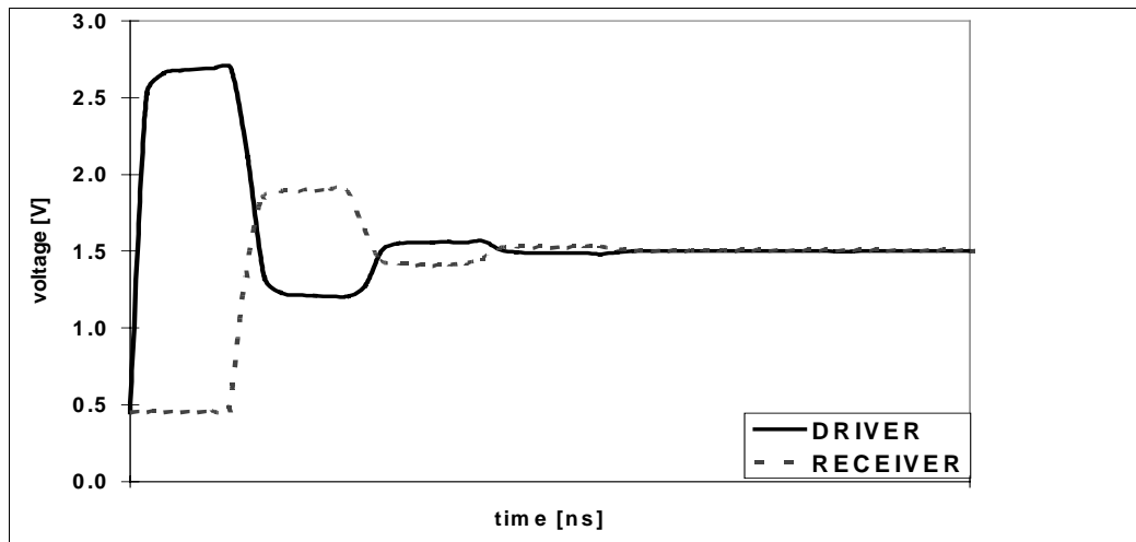
Figure 6. Waveform at the driver for the network in Figure 3.
