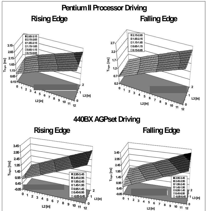
Figure 17. Parametric sweep maximum flight times for single processor design
