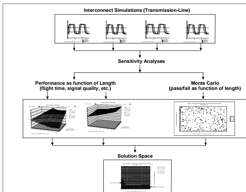
Figure 29. Pre-layout simulation process
