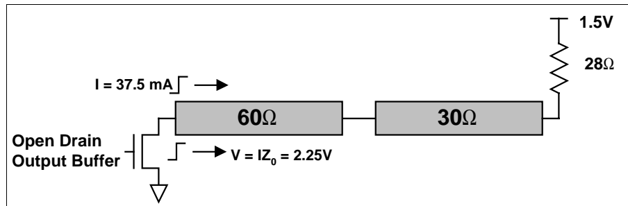
Figure 5. Waveform launch for low-high signal transition.
