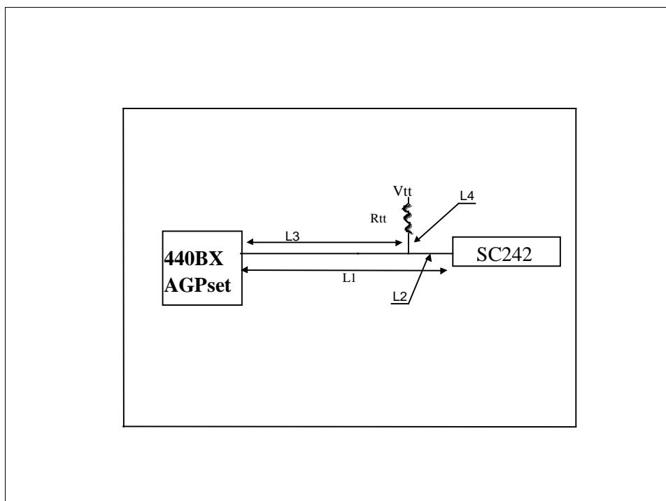
Figure 15. Recommended topology for single processor design
