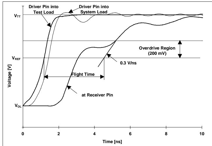
Figure 11. Flight time measurement with edge slower than 0.3 V/ns
