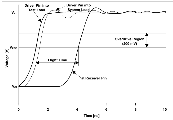
Figure 10. Nominal flight time measurement
