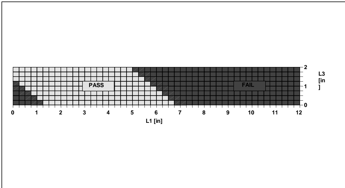
Figure 18. Solution space for single processor design, based on results of parametric sweeps
