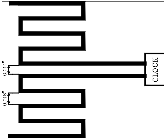
Figure 27. Clock trace spacing guidelines
