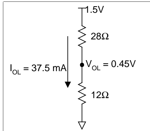
Figure 4. Equivalent circuit for output low state.
