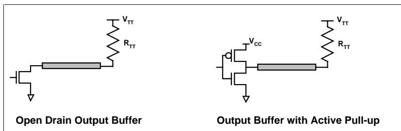
Figure 8. AGTL+ buffer types - open drain and active pull-up
