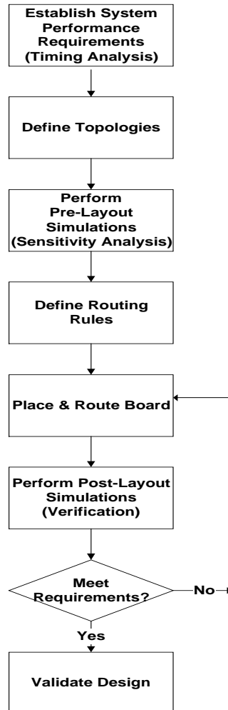
Figure 28. AGTL+ Design Process
