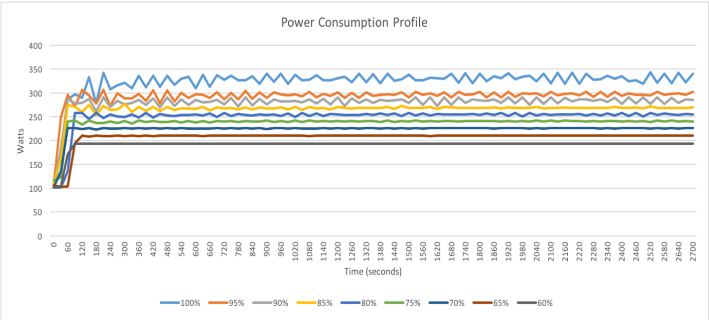
Figure 8: Power consumption profile over the course of our storage-intensive workload test.
