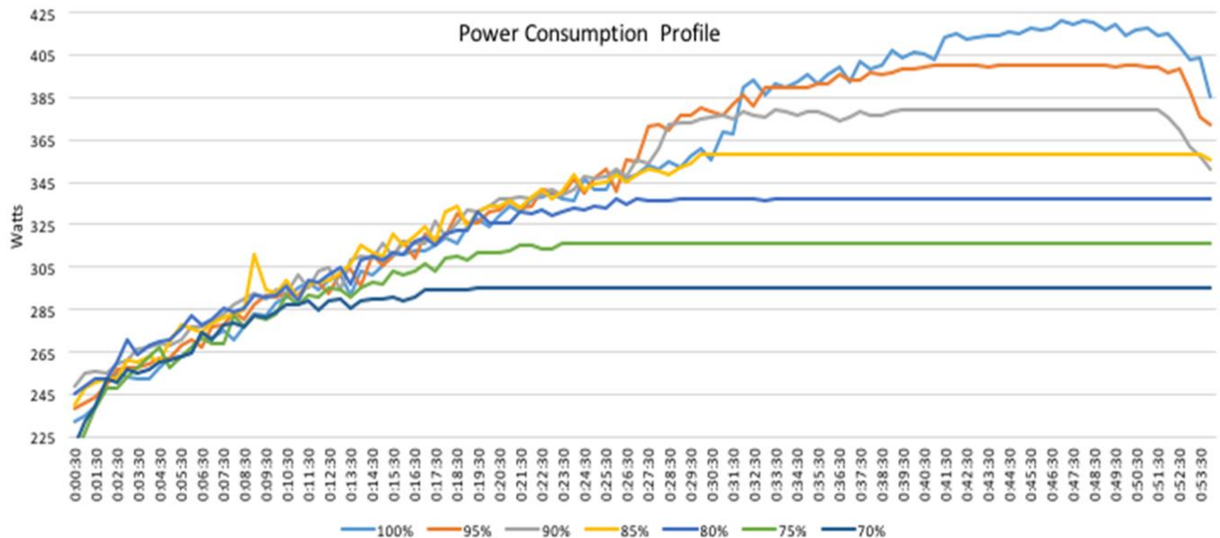
Figure 12: Power consumption profile over the course of our CPU-intensive workload test.
