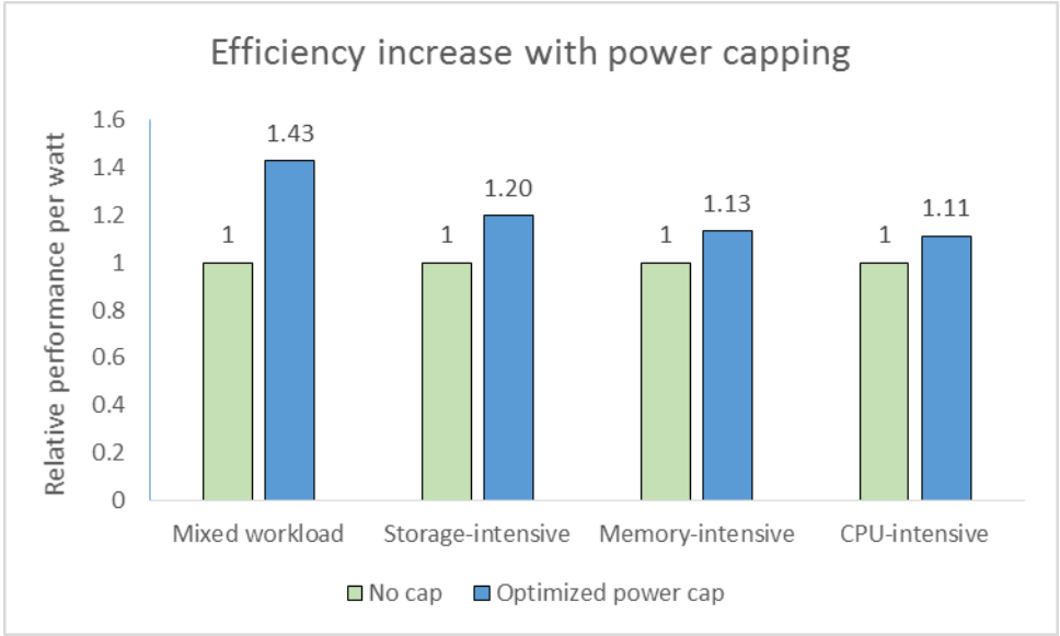
Figure 1: Intel Node Manager let us set power capping policies that increased performance/watt for various common workloads.
