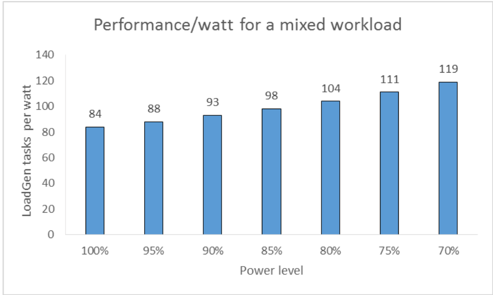
Figure 2: Using Intel Node Manager to set a power cap increased performance/watt up to an optimized 70% cap.
