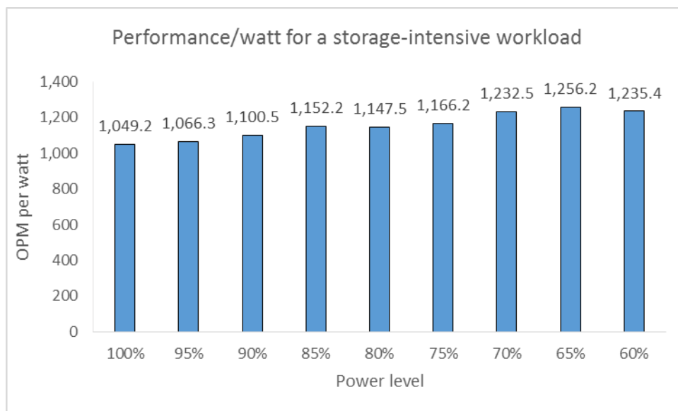
Figure 3: Using Intel Node Manager to set a power cap increased performance/watt up to an optimized 65% cap.
