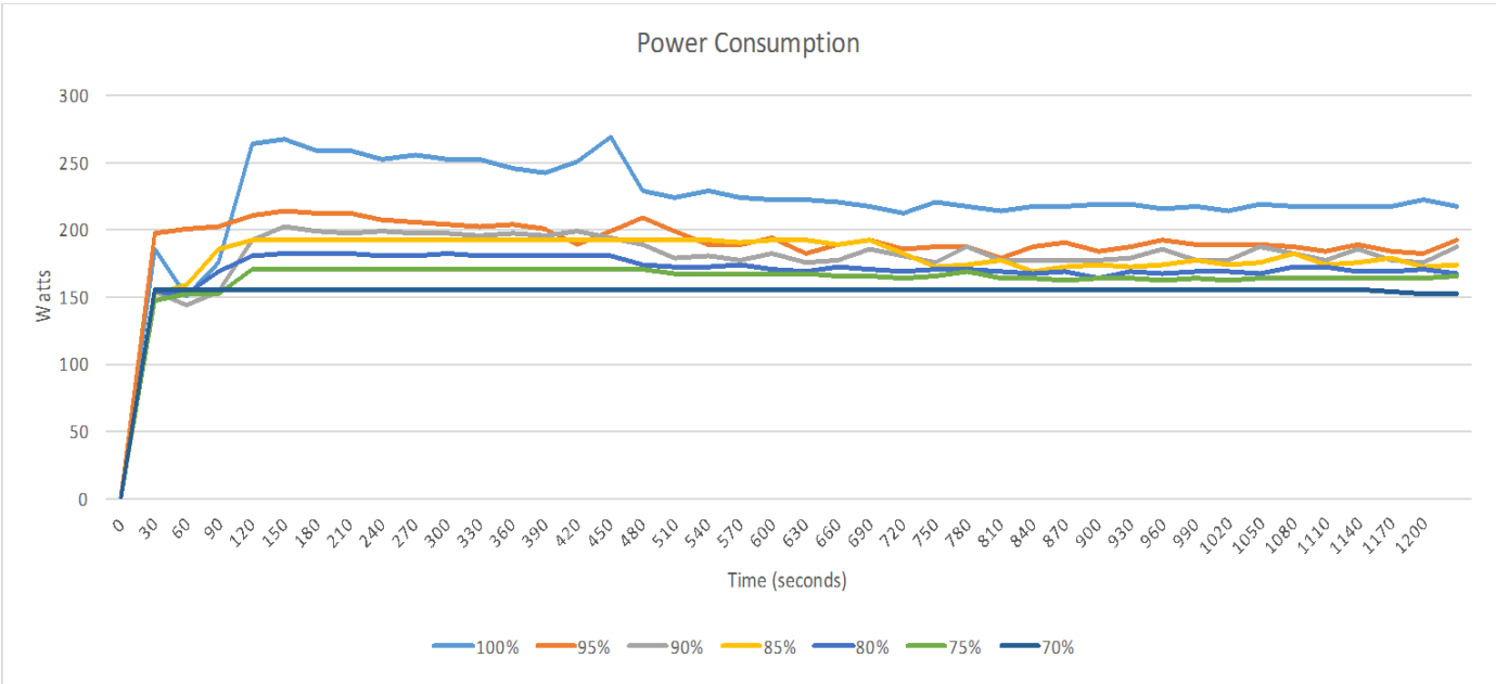
Figure 6: Power consumption profile over the course of our mixed workload test.
