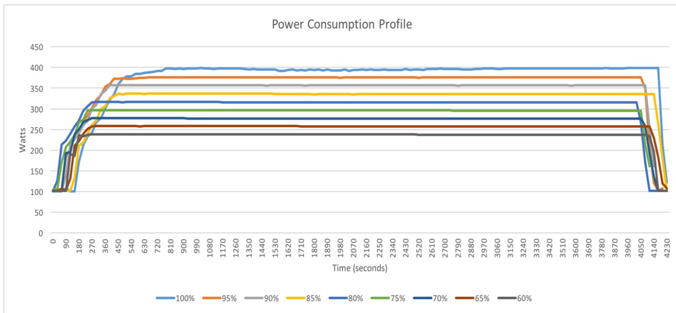
Figure 10: Power consumption profile over the course of our memory-intensive workload test.
