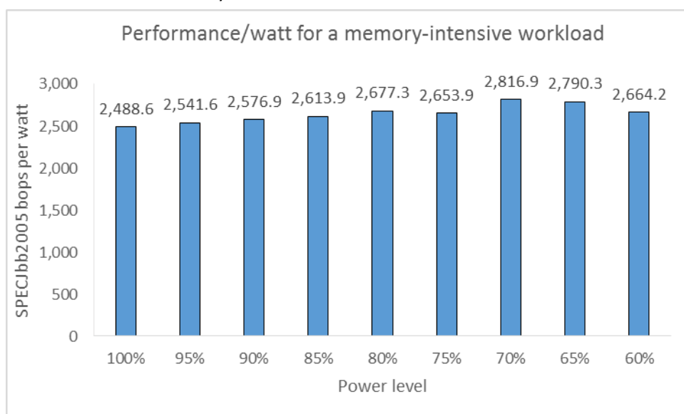
Figure 4: Using Intel Node Manager to set a power cap increased performance/watt up to an optimized 70% cap.
