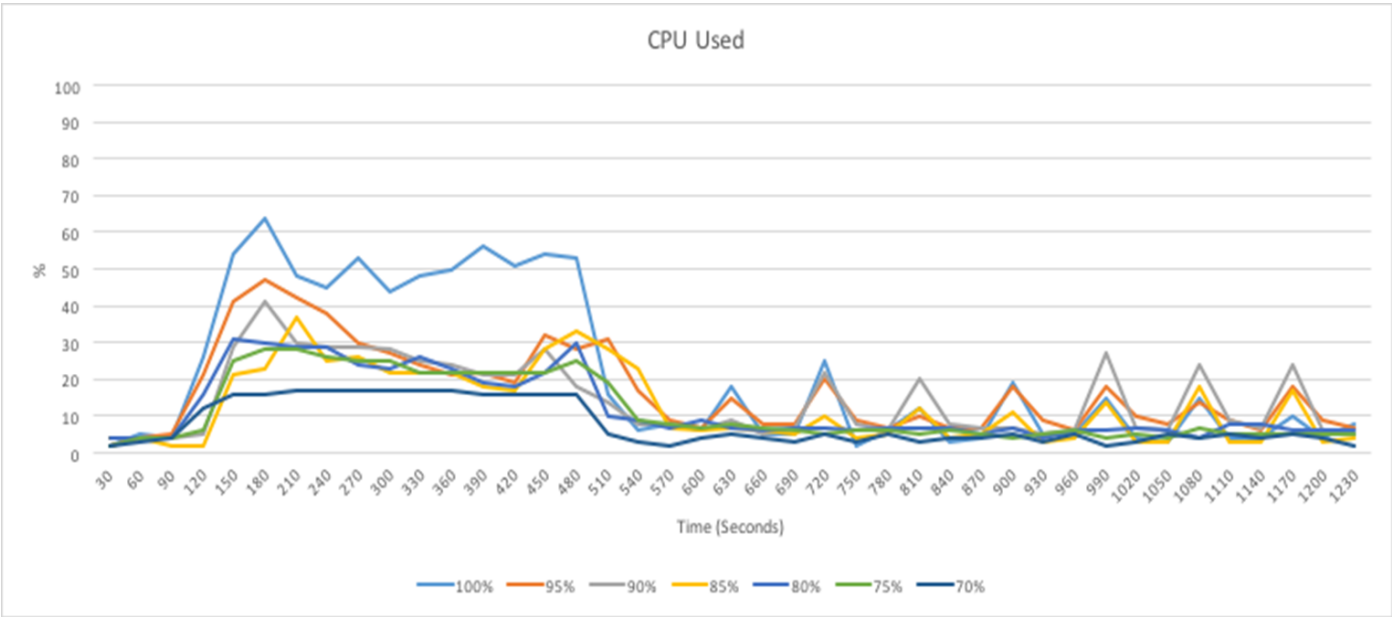
Figure 7: CPU utilization over the course of our mixed workload test.
