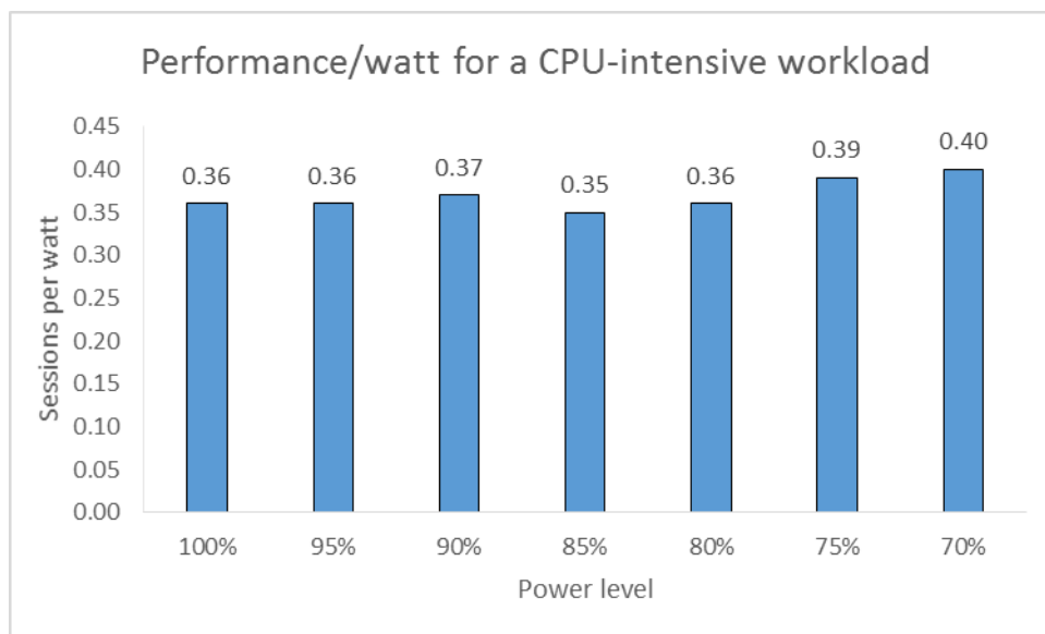
Figure 5: Using Intel Node Manager to set a power cap increased VDI sessions/watt up to an optimized 70% cap.
