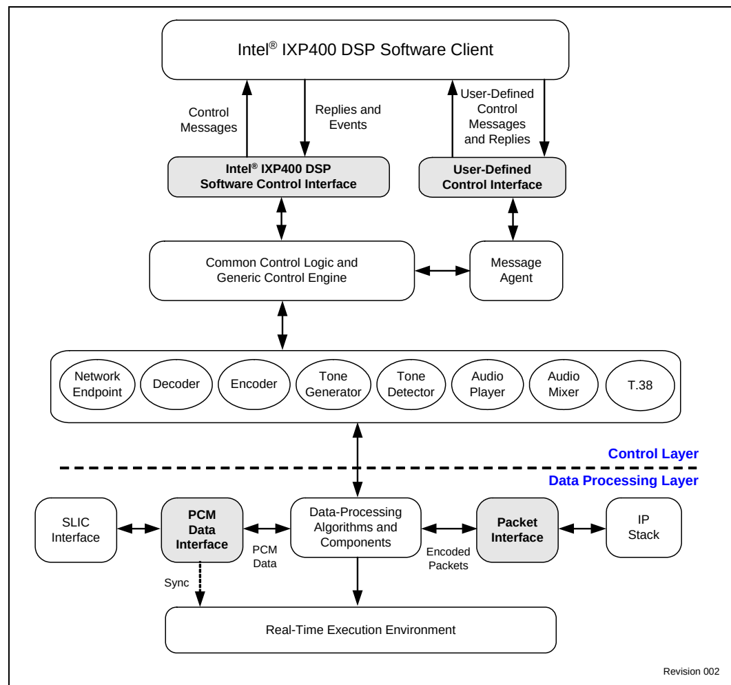
Figure 1. Architecture of Intel® IXP400 DSP Software v2.5
