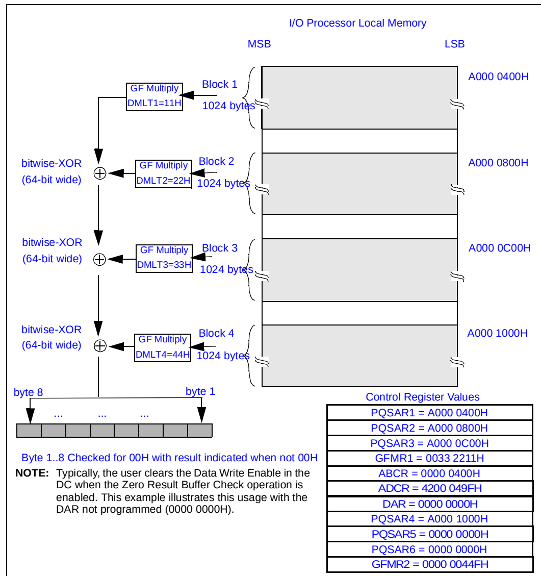
Figure 22. An example of Zero Result Buffer Check with P+Q RAID-6
