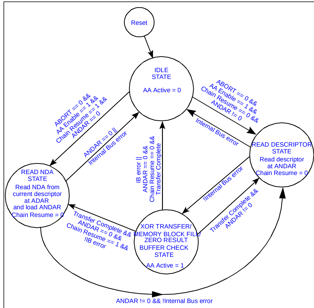
Figure 24. Application Accelerator Programming Model State Diagram
