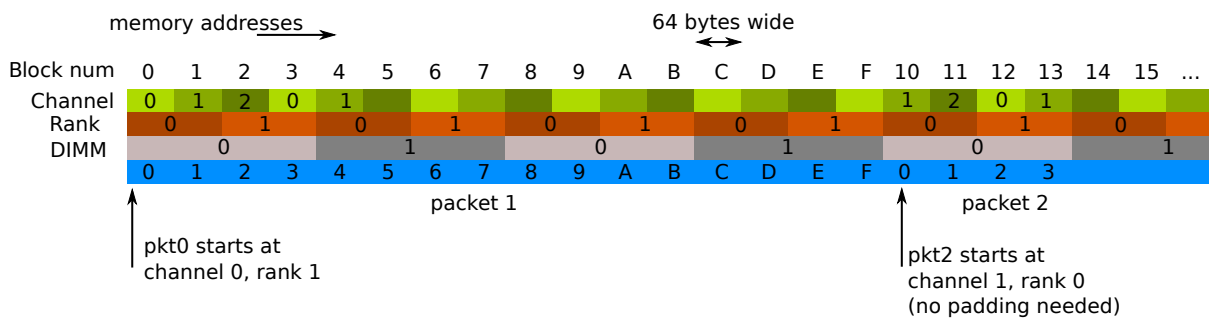
Figure 6.2: Three Channels and Two Dual-ranked DIMM Example
