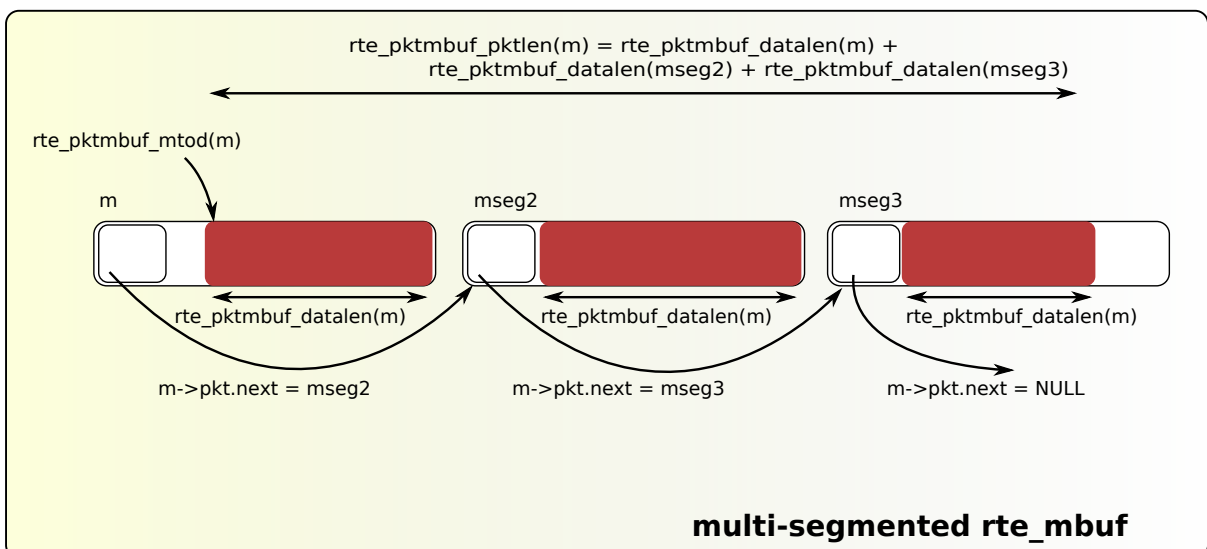
Figure 7.2: An mbuf with Three Segments
