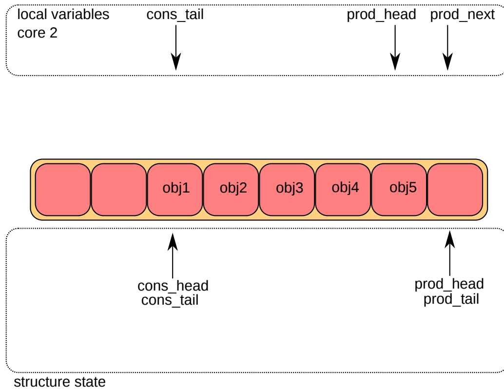
Figure 5.12: Multiple consumer enqueue last step
