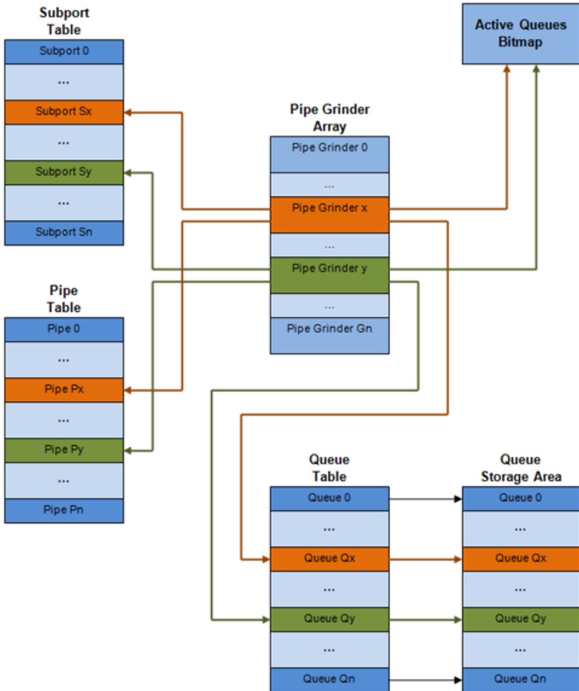
Figure 21.4: Internal Data Structures per Port
