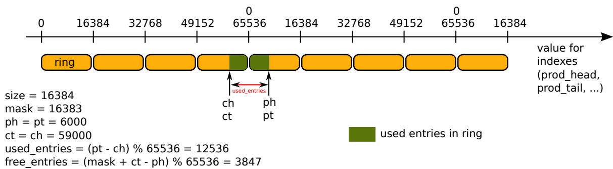
Figure 5.14: Modulo 32-bit indexes - Example 2
