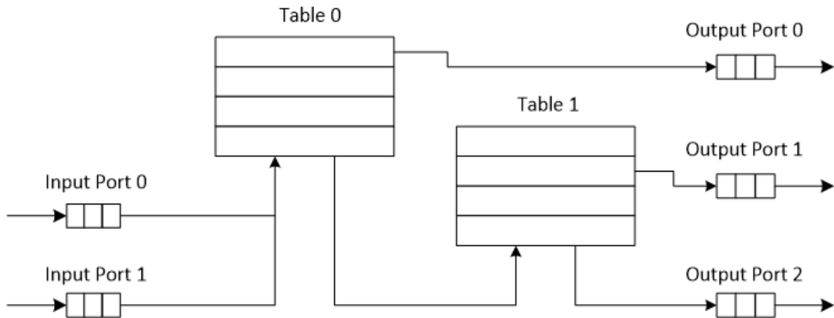
Figure 24.1: Example of Packet Processing Pipeline where Input Ports 0 and 1 are Connected with Output Ports 0, 1 and 2 through Tables 0 and 1
