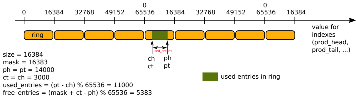
Figure 5.13: Modulo 32-bit indexes - Example 1
