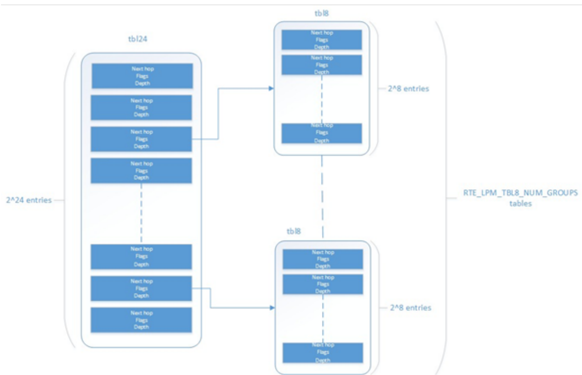
Figure 13.1: Table split into different levels
