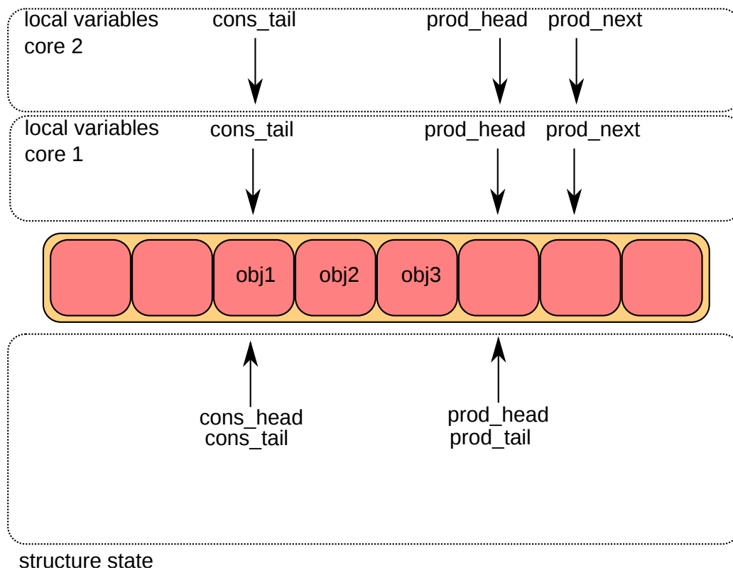
Figure 5.8: Multiple consumer enqueue first step
