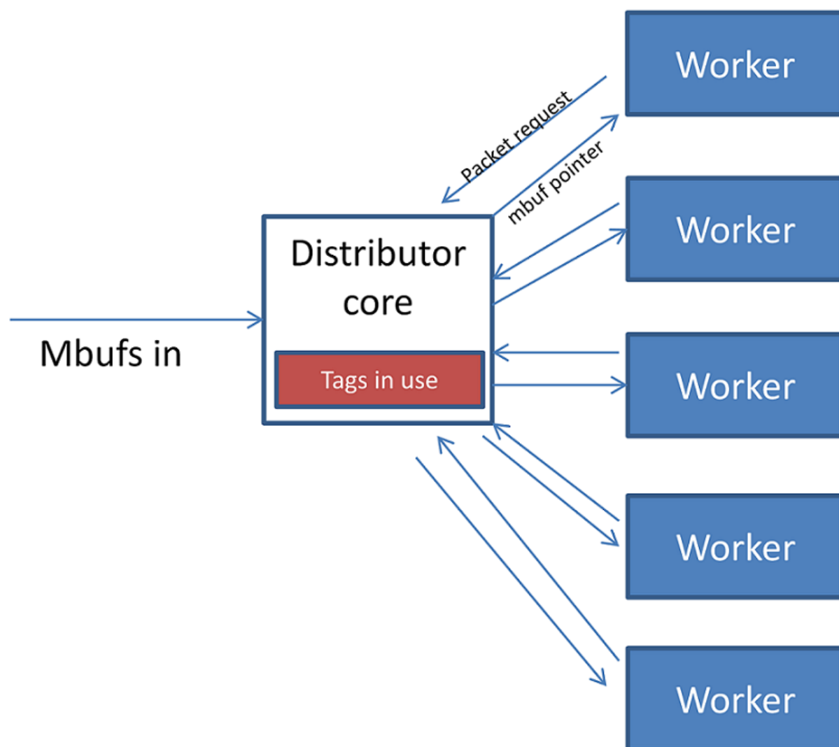
Figure 15.1: Packet Distributor mode of operation
