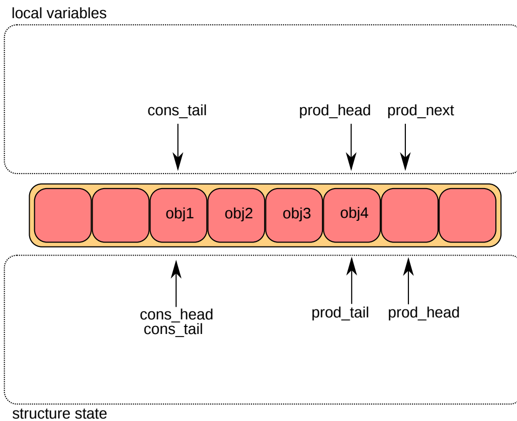
Figure 5.3: Enqueue second step
