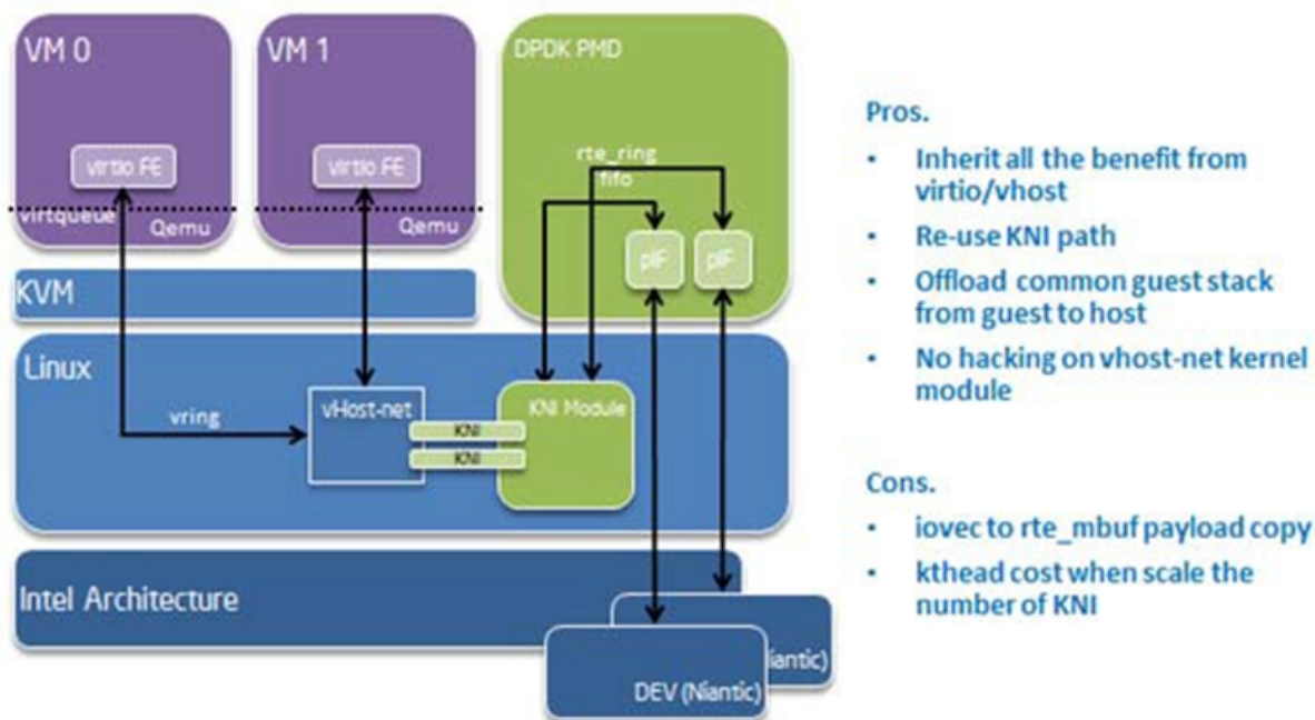
Figure 19.3: vHost-net Architecture Overview
