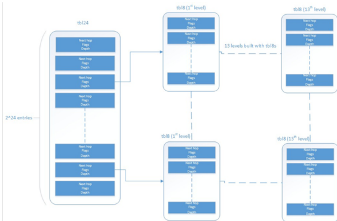
Figure 14.1: Table split into different levels
