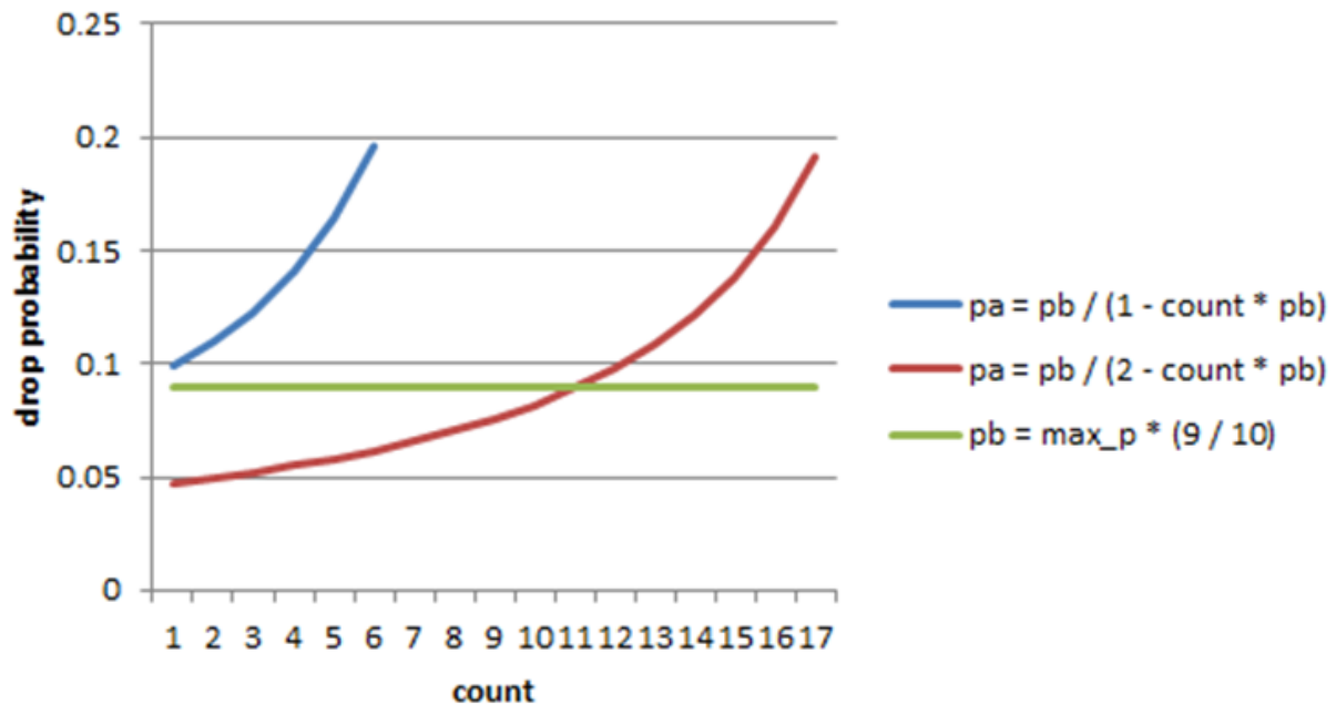
Figure 21.11: Initial Drop Probability (pb), Actual Drop probability (pa) Computed Using a Factor 1 (Blue Curve) and a Factor 2 (Red Curve)
