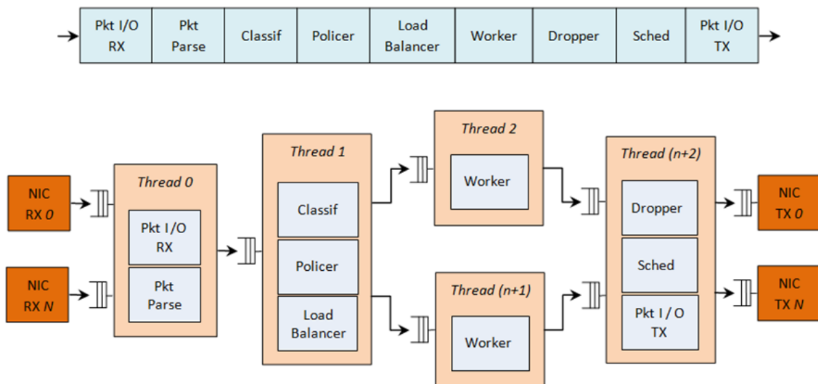
Figure 21.1: Complex Packet Processing Pipeline with QoS Support
