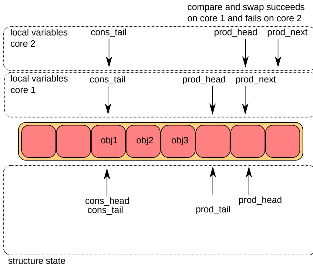
Figure 5.9: Multiple consumer enqueue second step
