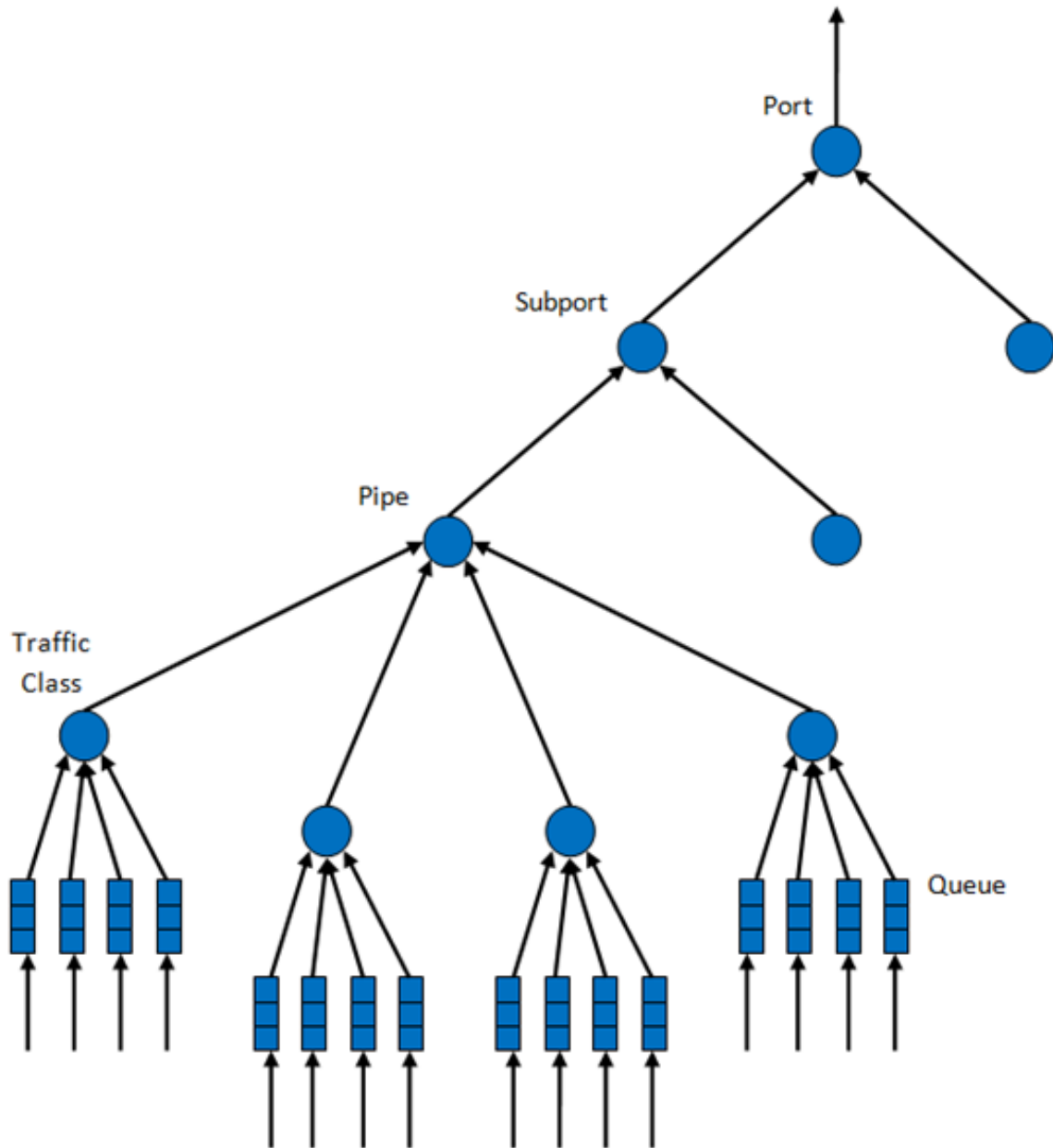
Figure 21.3: Scheduling Hierarchy per Port
