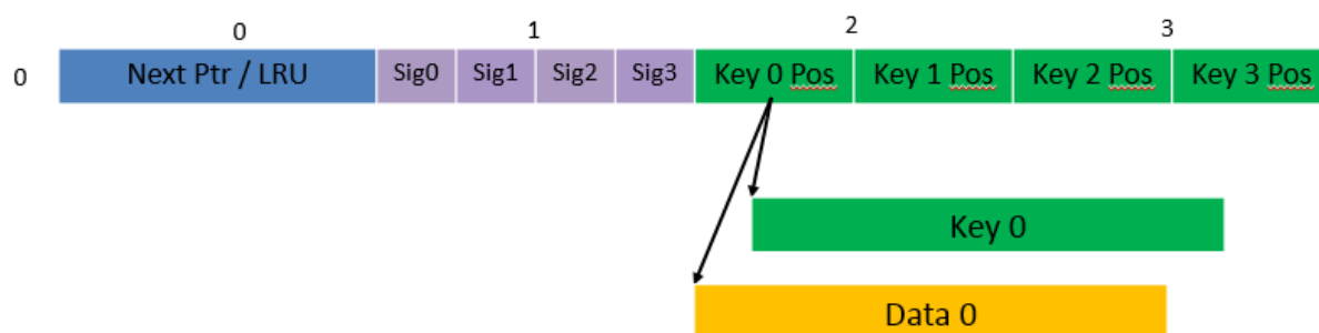
Figure 24.3: Data Structures for Configurable Key Size Hash Tables
