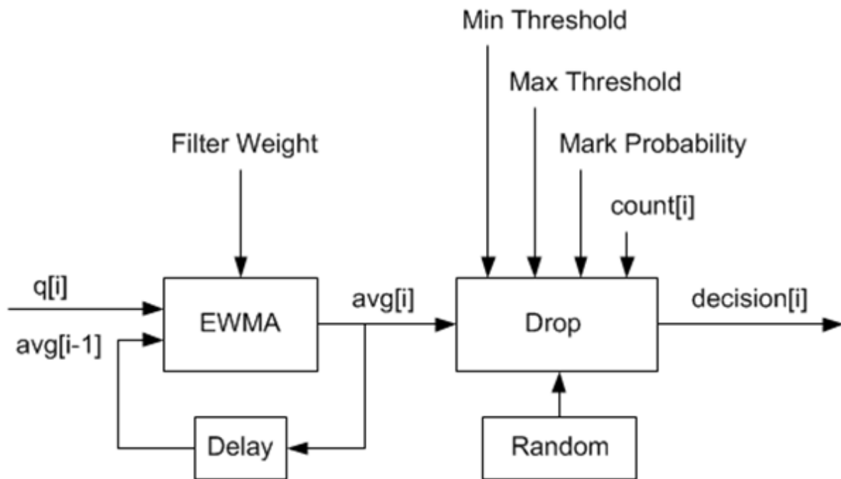
Figure 21.9: Example Data Flow Through Dropper
