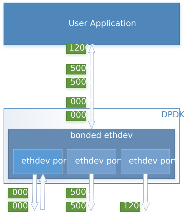
Figure 10.7: Transmit Load Balancing (Mode 5)
