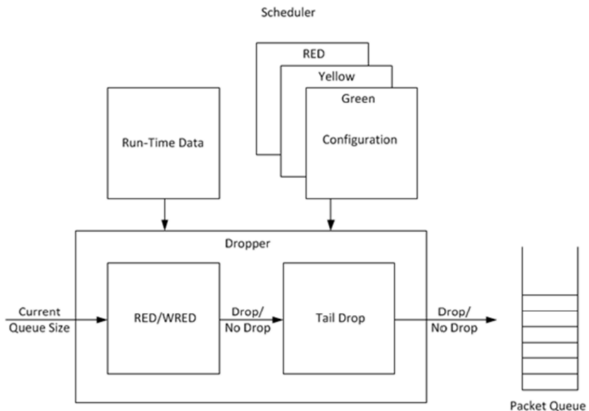
Figure 21.7: High-level Block Diagram of the DPDK Dropper
