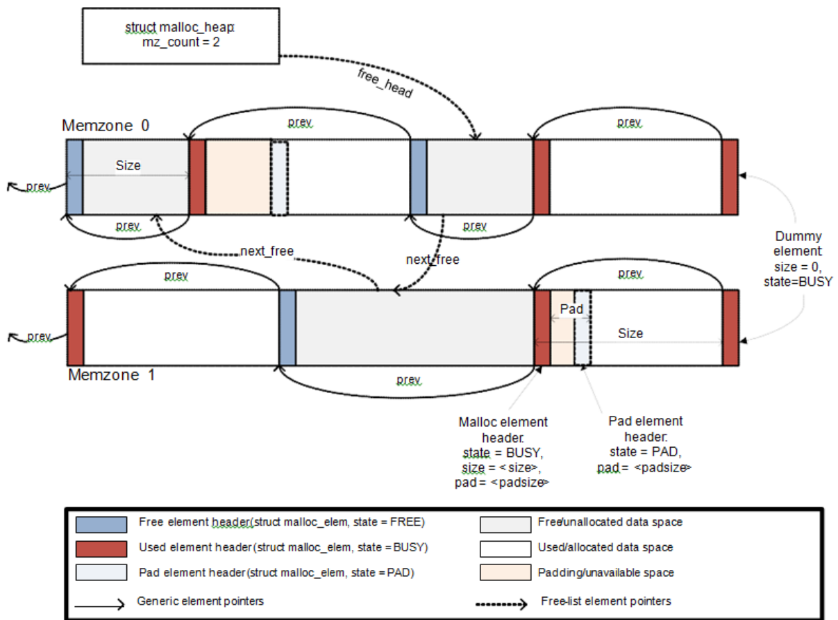
Figure 4.1: Example of a malloc heap and malloc elements within the malloc library
