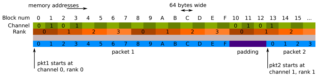
Figure 6.1: Two Channels and Quad-ranked DIMM Example
