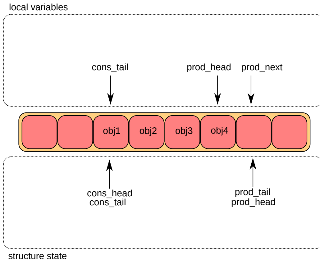
Figure 5.4: Enqueue last step
