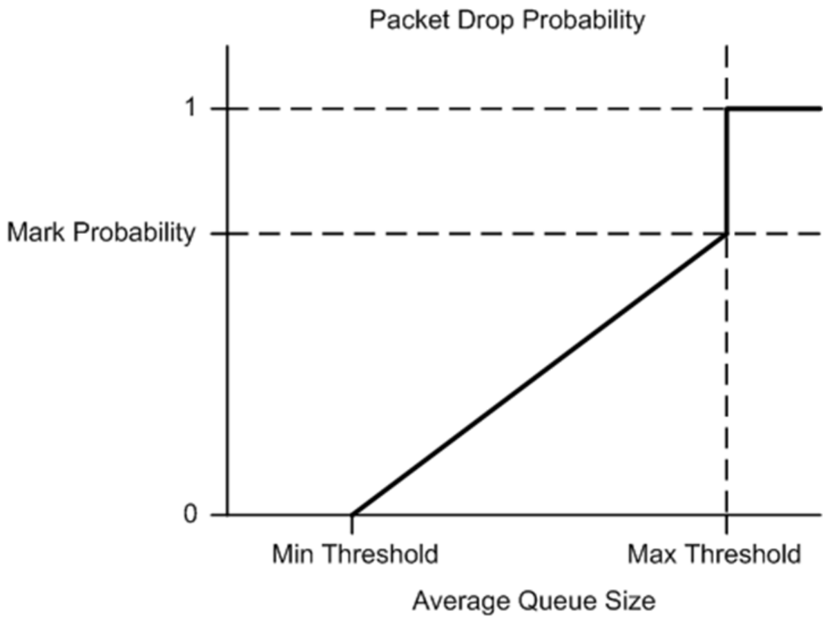
Figure 21.10: Packet Drop Probability for a Given RED Configuration
