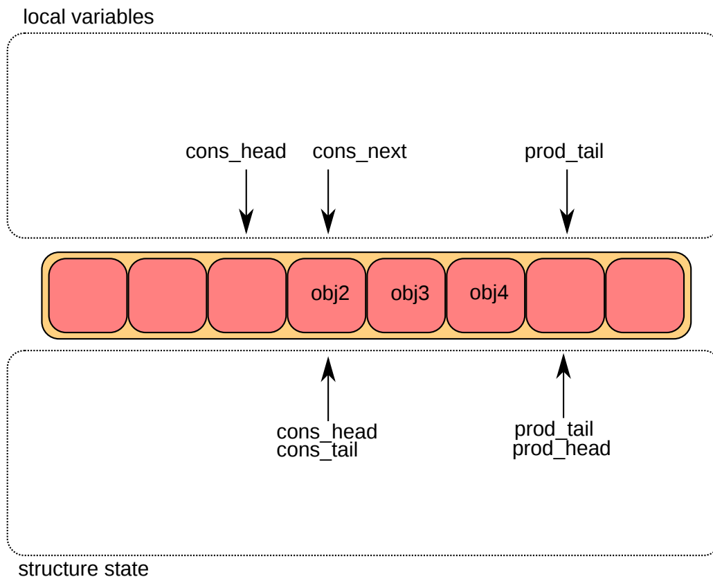
Figure 5.7: Dequeue last step
