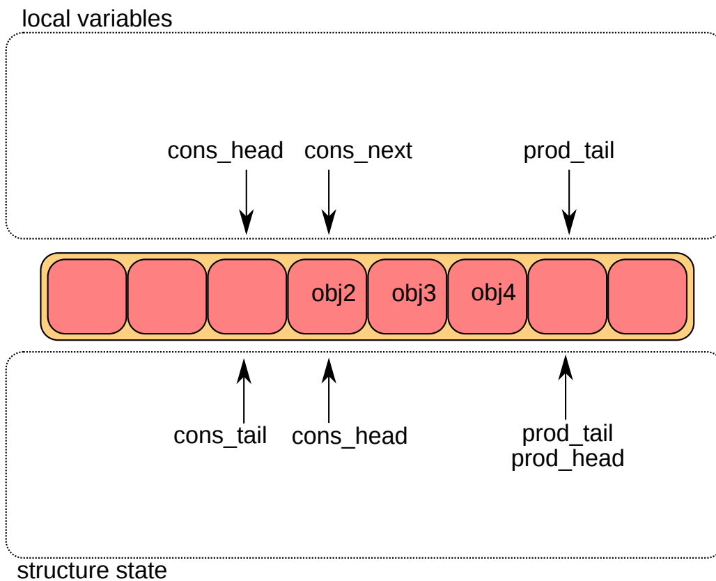
Figure 5.6: Dequeue second step
