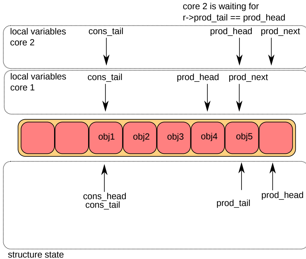
Figure 5.11: Multiple consumer enqueue fourth step
