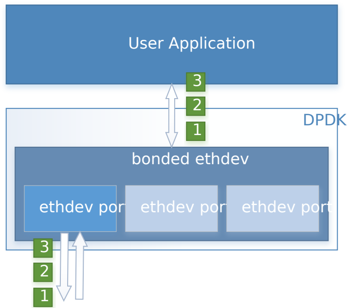
Figure 10.3: Active Backup (Mode 1)
