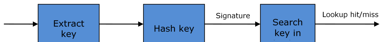
Figure 24.2: Sequence of Steps for Hash Table Operations in a Packet Processing Context
