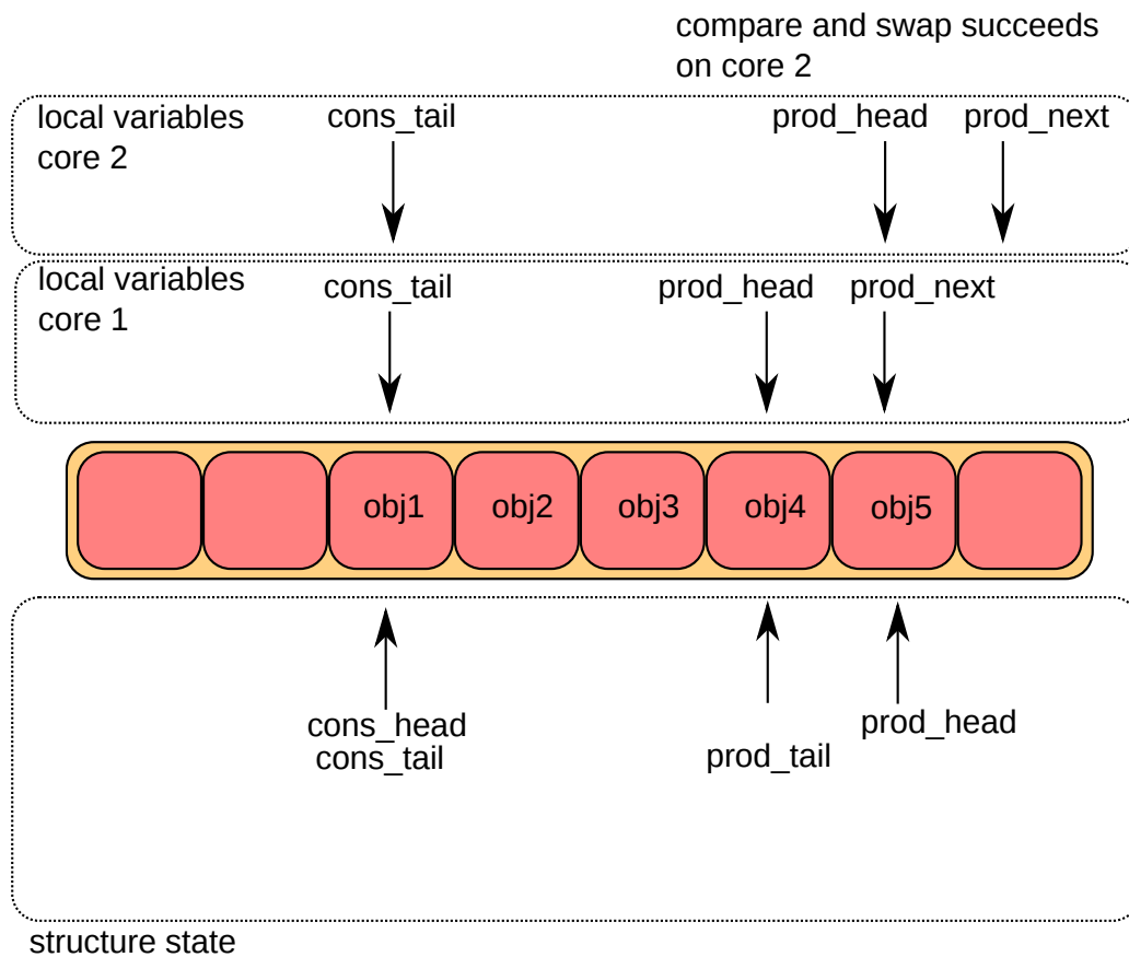
Figure 5.10: Multiple consumer enqueue third step
