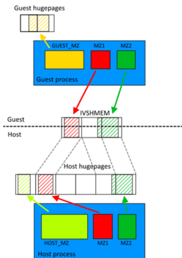
Figure 9.1: Typical Ivshmem use case
