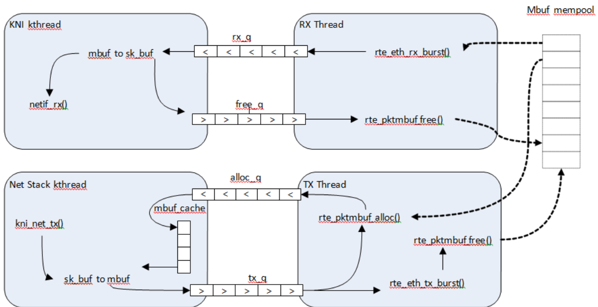
Figure 19.2: Packet Flow via mbufs in the DPDK KNI
