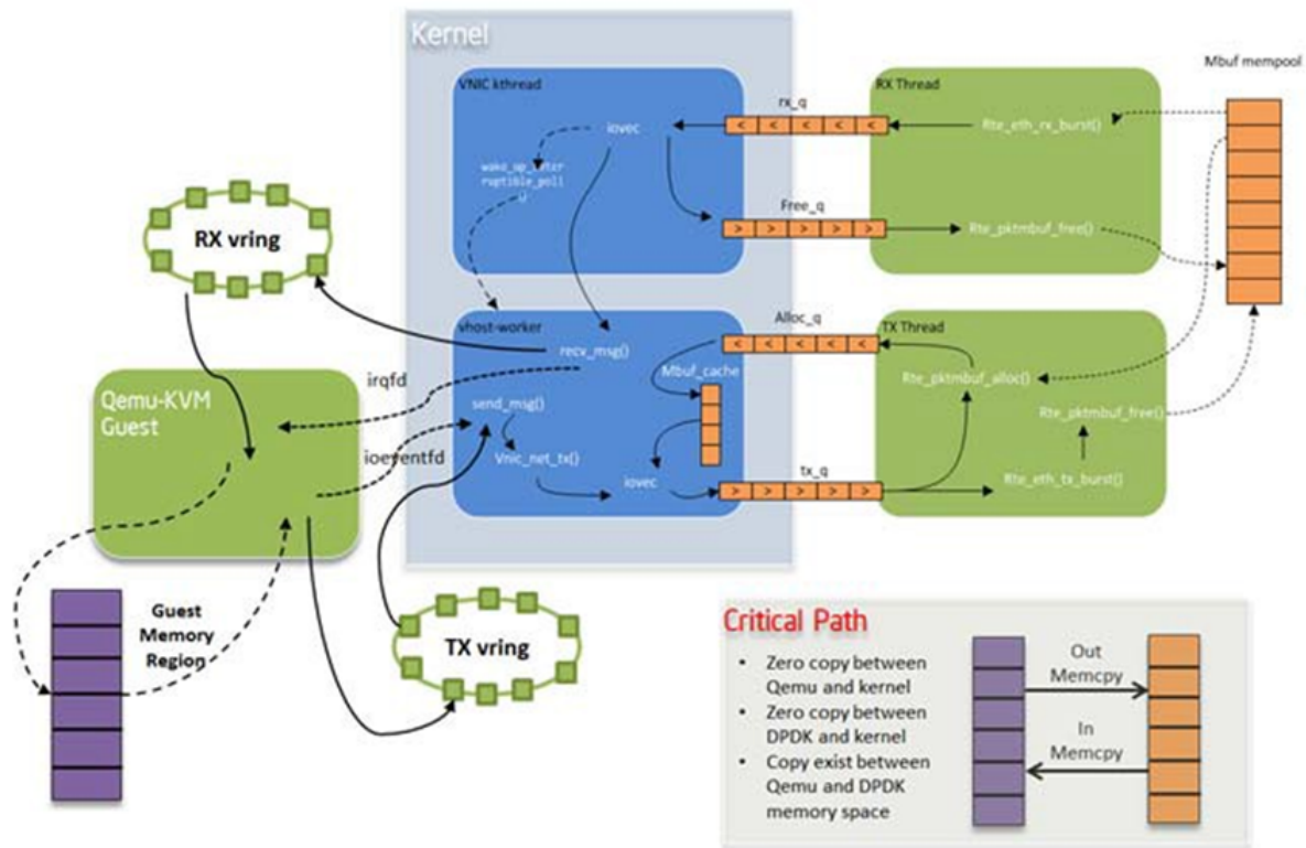
Figure 19.4: KNI Traffic Flow
