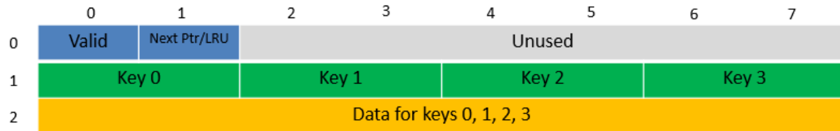
Figure 24.6: Data Structures for 16-byte Key Hash Tables
