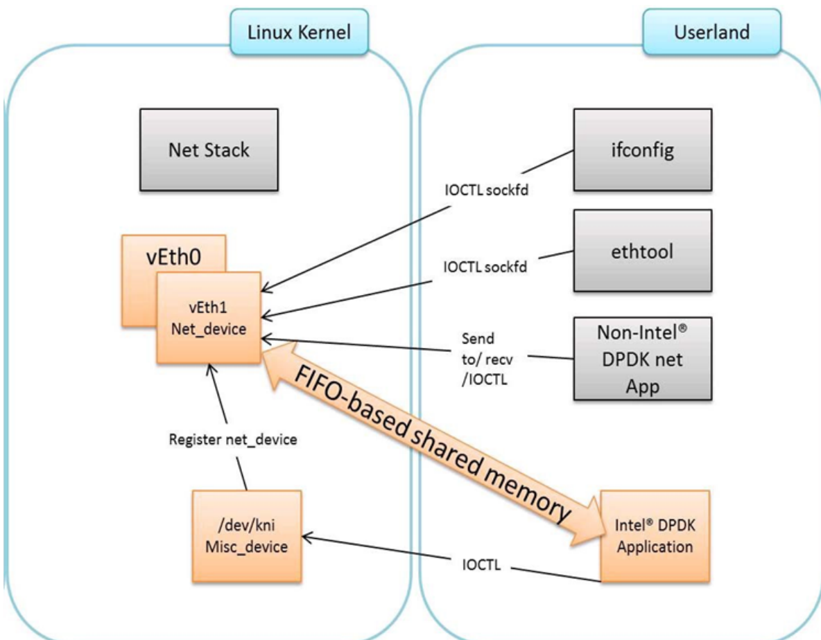
Figure 19.1: Components of a DPDK KNI Application
