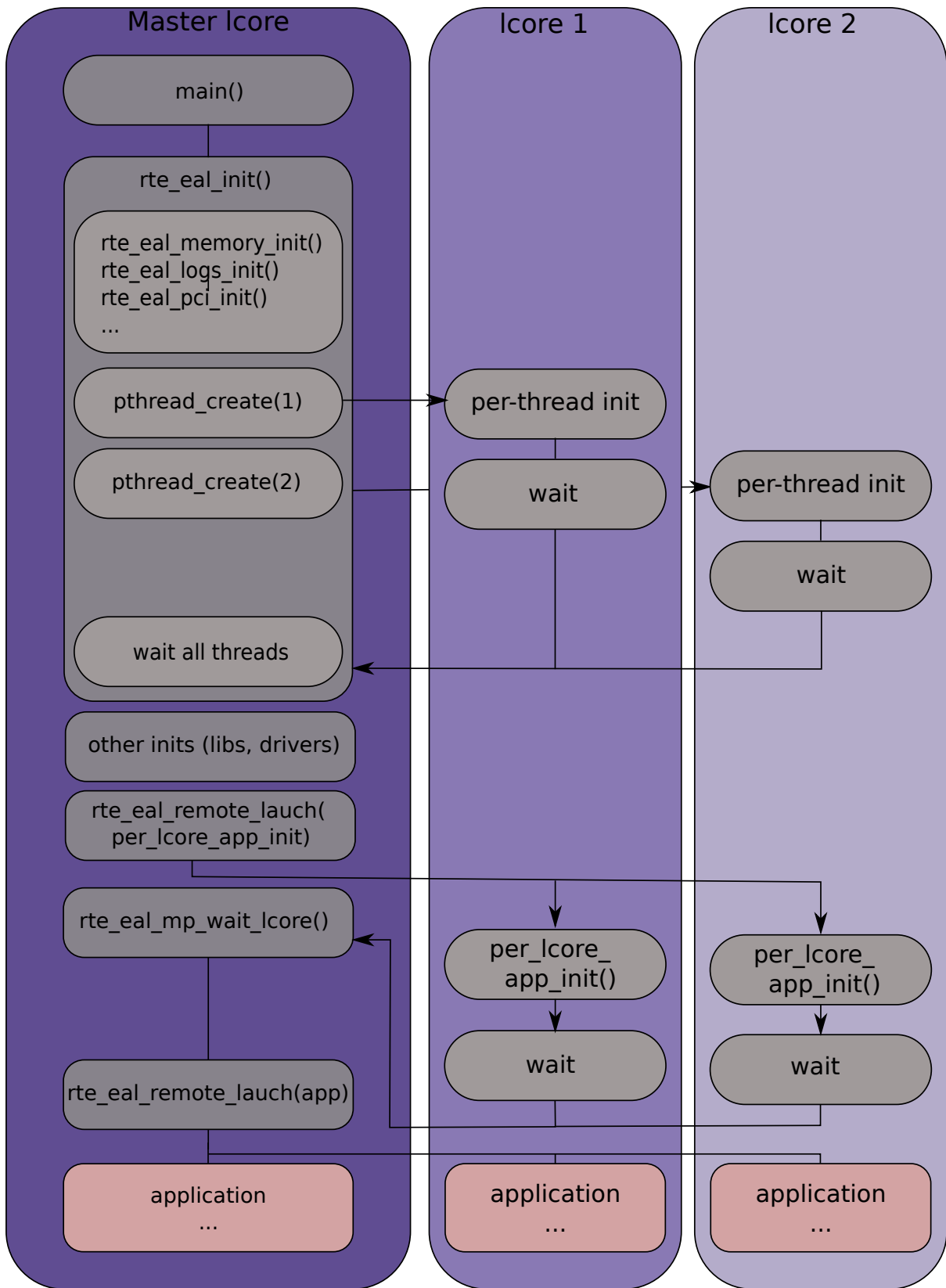
Figure 3.1: EAL Initialization in a Linux Application Environment
