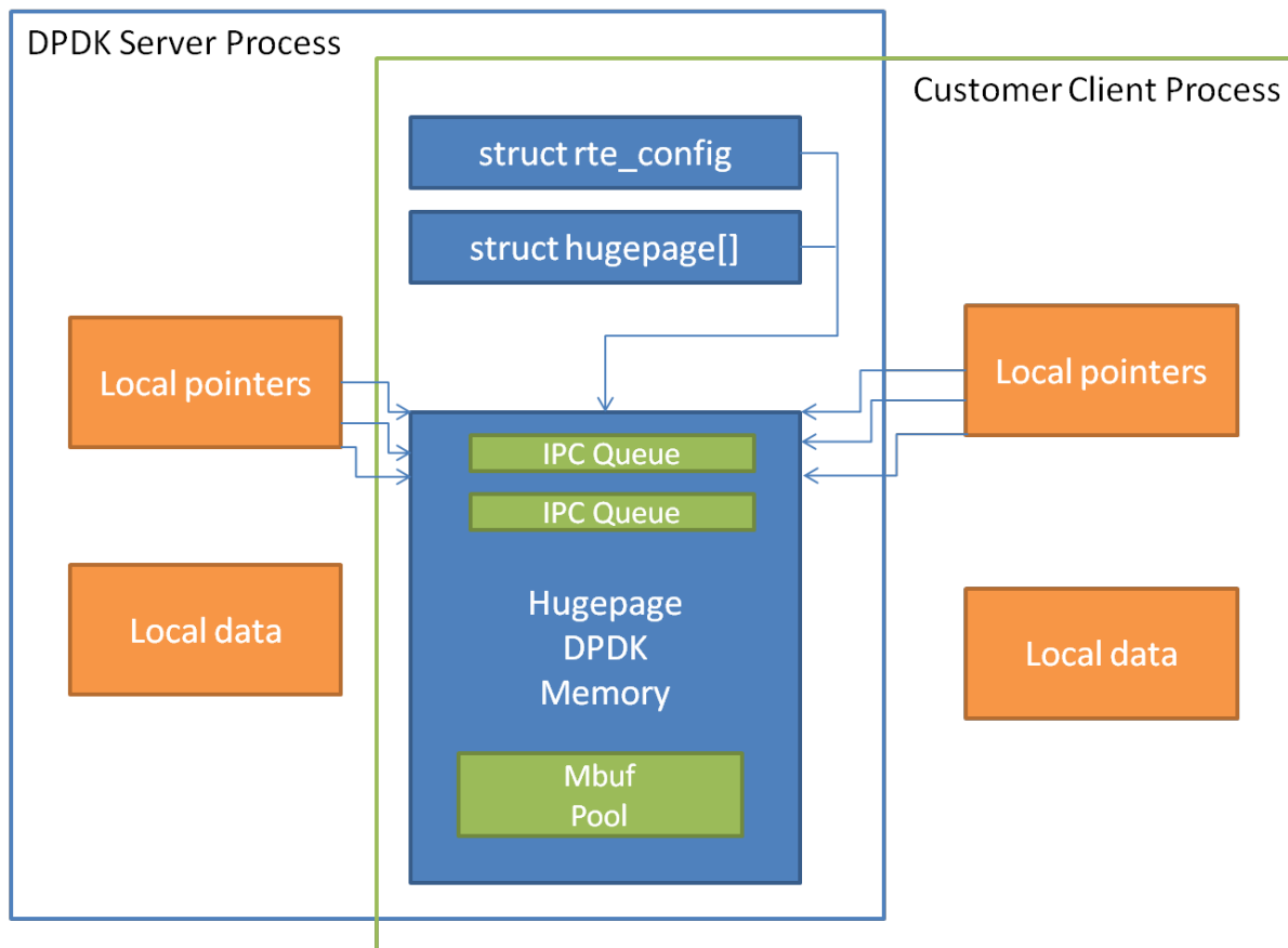
Figure 18.1: Memory Sharing in the DPDK Multi-process Sample Application
