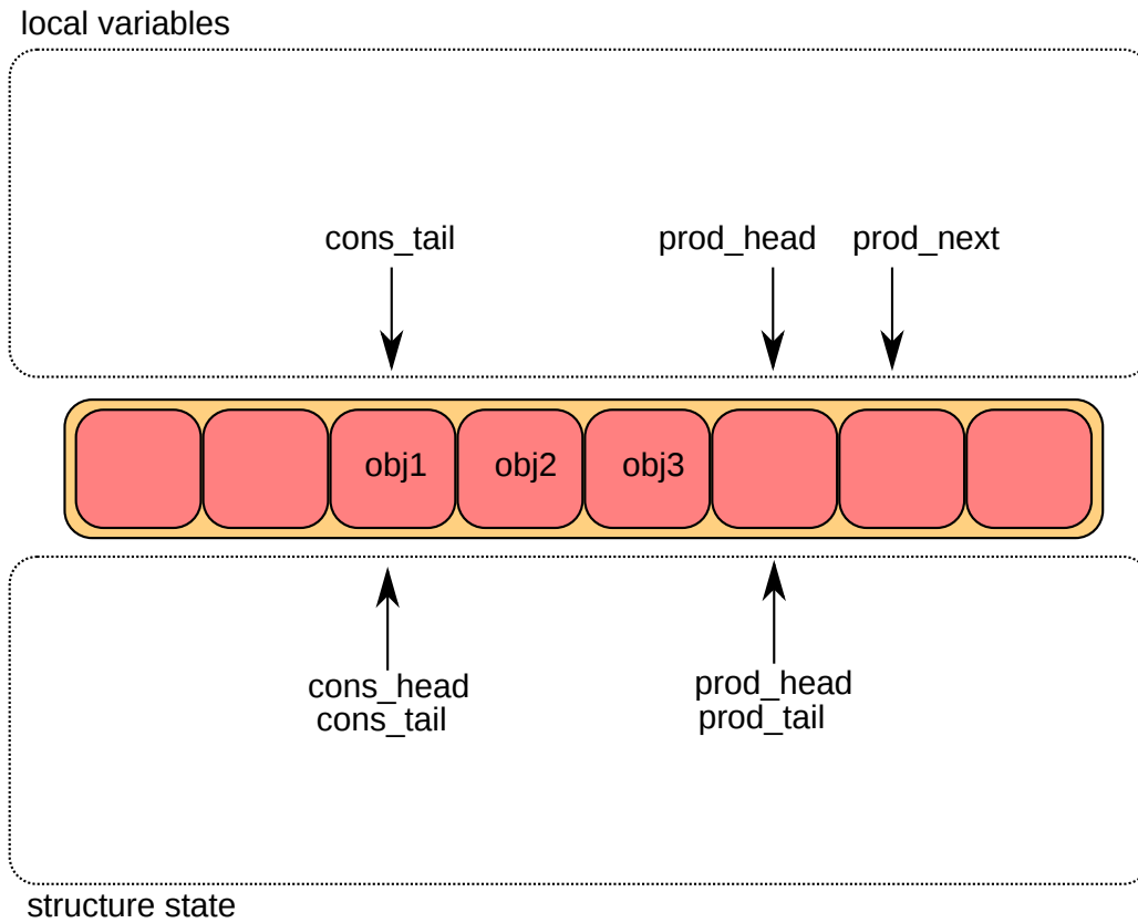
Figure 5.2: Enqueue first step
