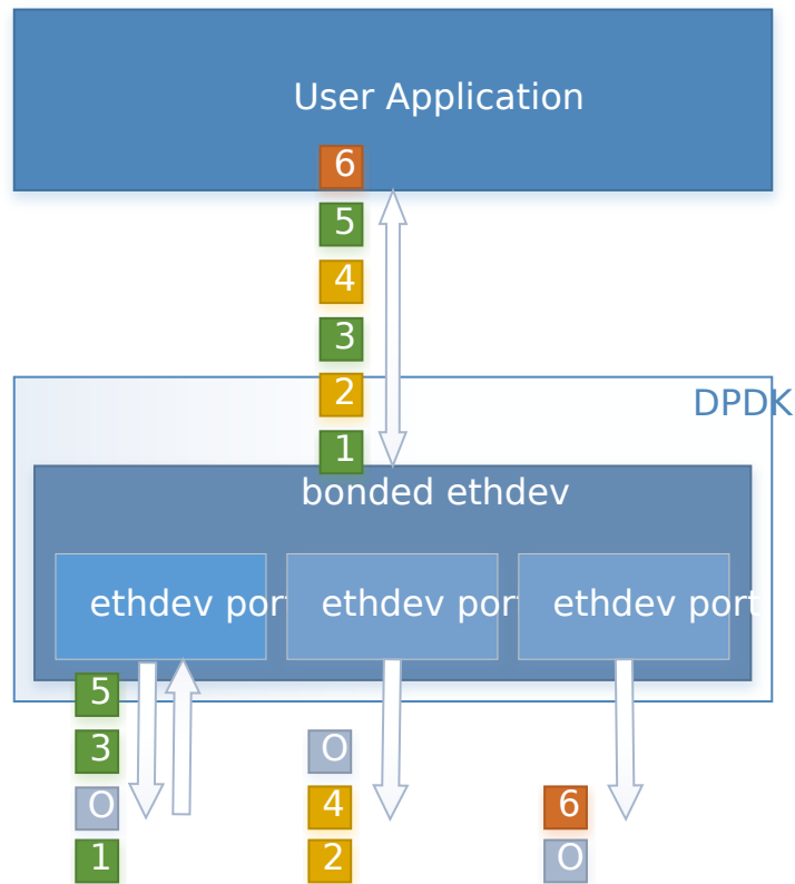
Figure 10.6: Link Aggregation 802.3AD (Mode 4)
