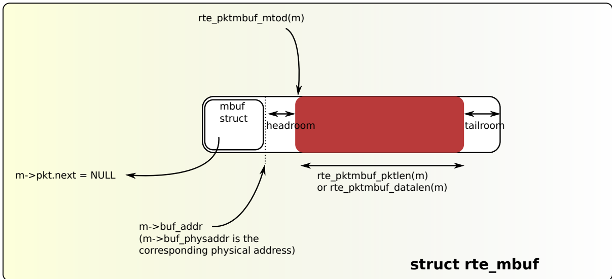
Figure 7.1: An mbuf with One Segment
