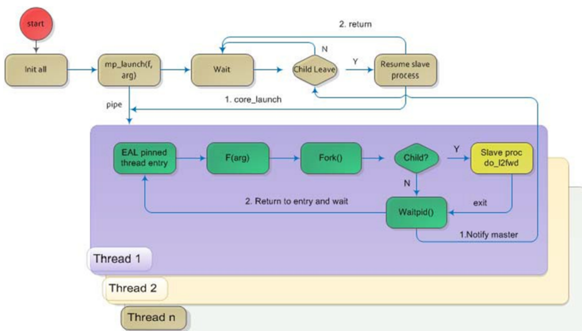
Figure 19.3: Master-slave Process Workflow
