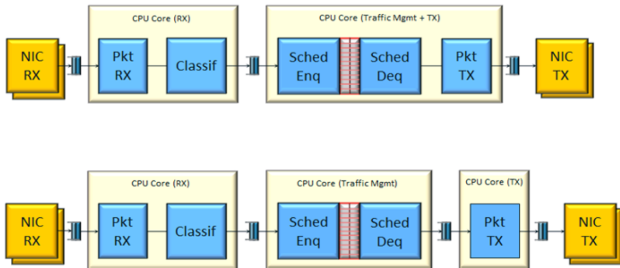
Figure 21.1: QoS Scheduler Application Architecture
