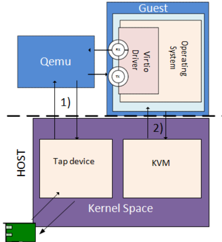
Figure 27.1: System Architecture for Virtio-based Networking (virtio-net).
