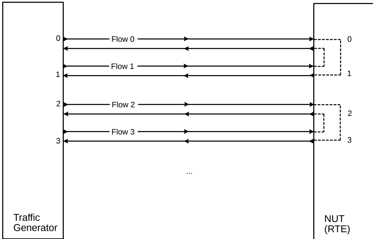
Figure 11.1: Performance Benchmark Setup (Basic Environment)
