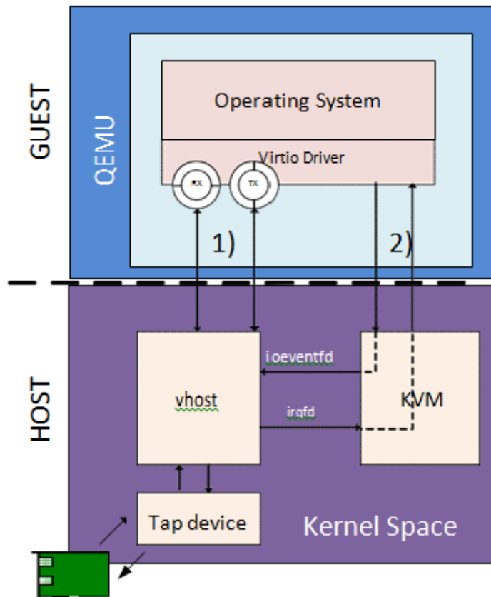
Figure 27.2: Virtio with Linux
