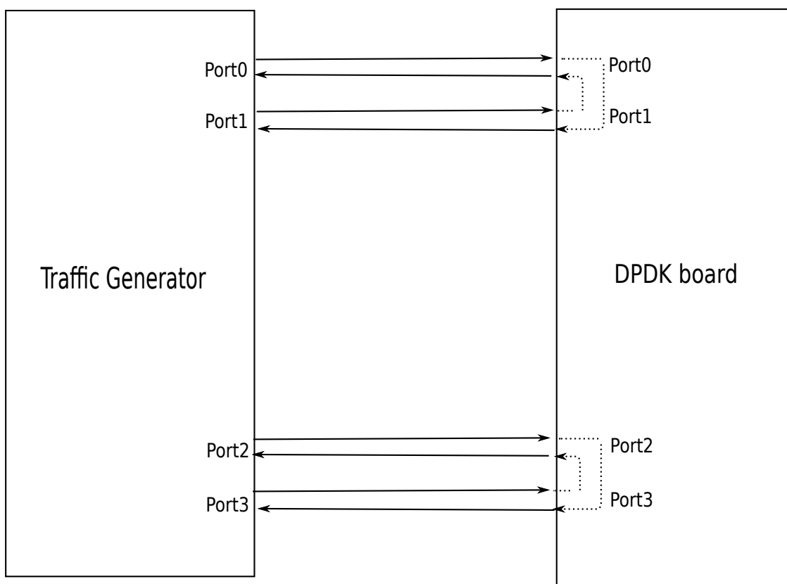
Figure 31.1: Performance Benchmarking Setup (Basic Environment)
