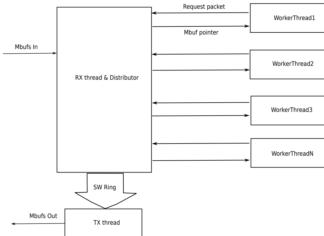
Figure 31.2: Distributor Sample Application Layout
