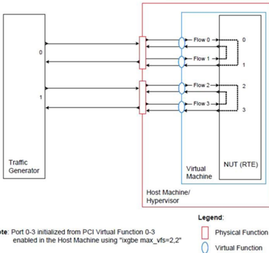
Figure 11.2: Performance Benchmark Setup (Virtualized Environment)
