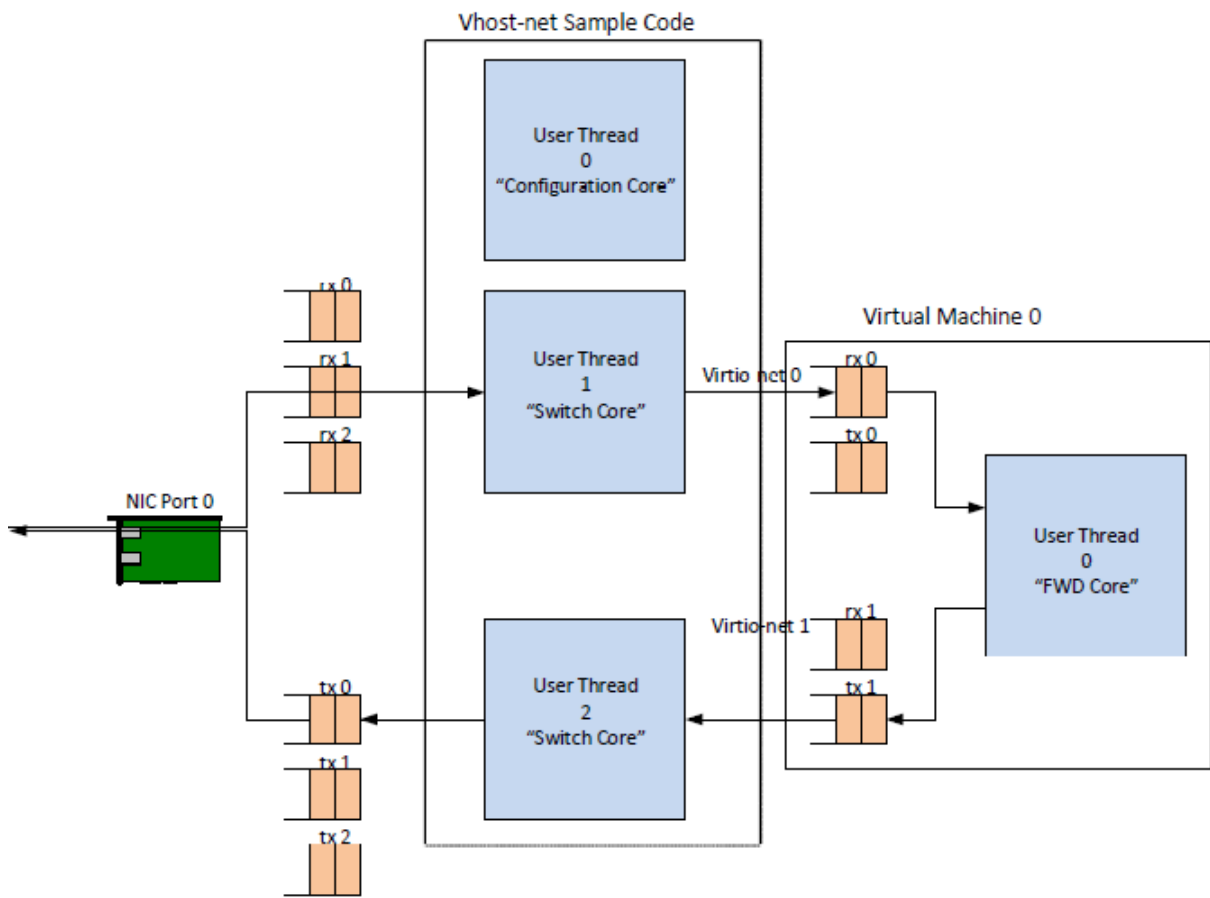
Figure 27.4: Packet Flow Through the vhost-net Sample Application
