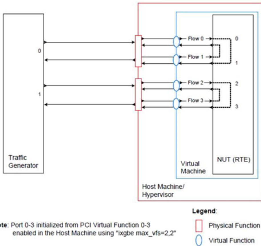
Figure 12.2: Performance Benchmark Setup (Virtualized Environment)
