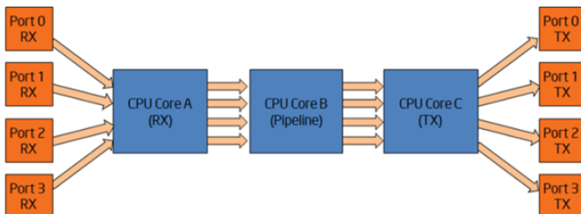
Figure 30.1: Test Pipeline Application
