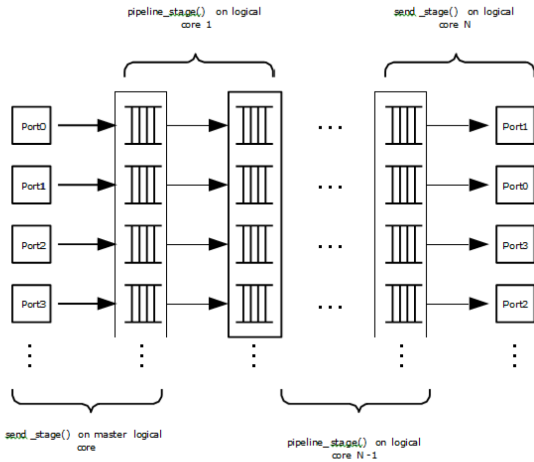
Figure 23.3: Threads and Pipelines
