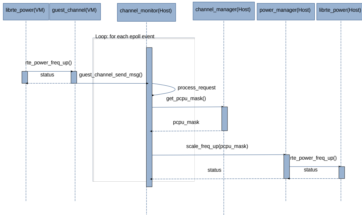
Figure 32.2: VM request to scale frequency
