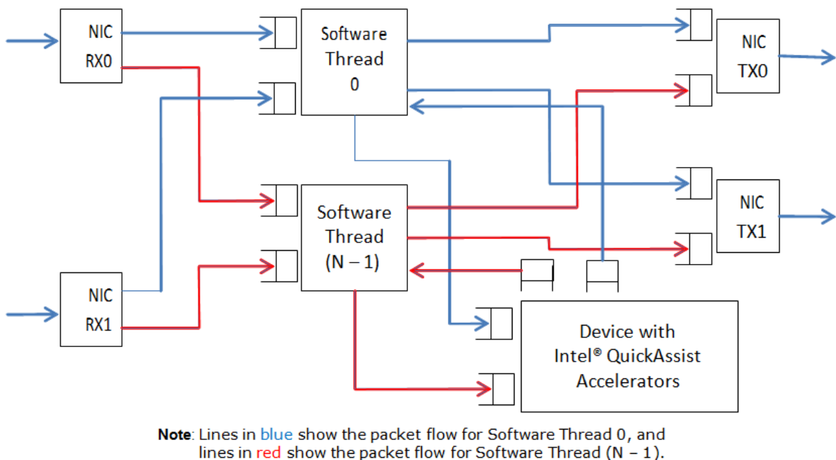
Figure 22.1: Intel® QuickAssist Technology Application Block Diagram
