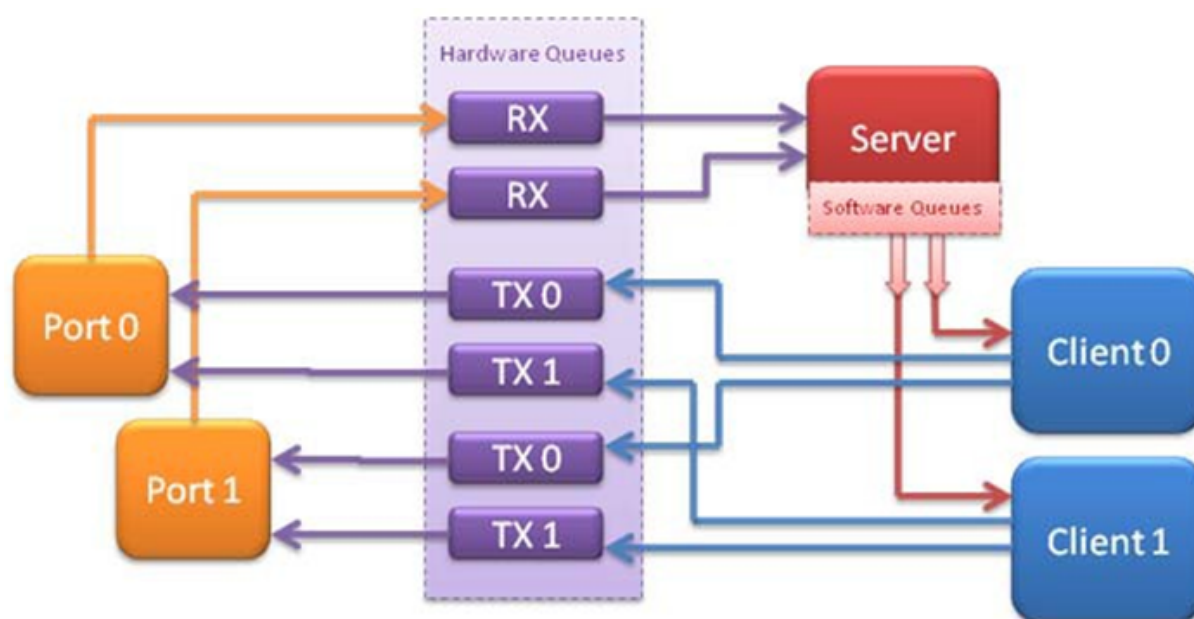
Figure 19.2: Example Data Flow in a Client-Server Symmetric Multi-process Application
