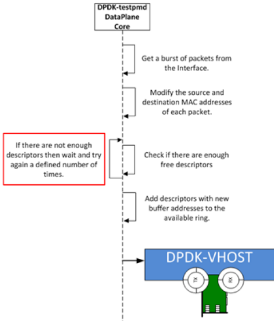
Figure 27.5: Packet Flow on TX in DPDK-testpmd
