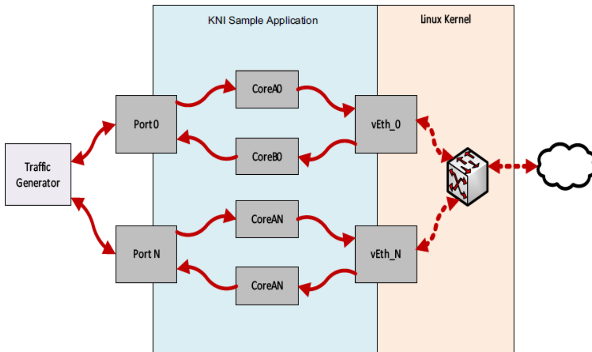
Figure 10.1: Kernel NIC Application Packet Flow
