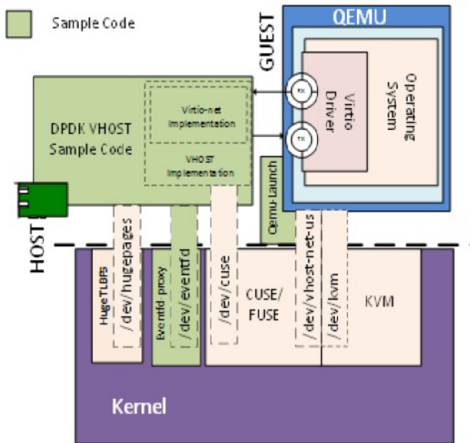
Figure 27.3: Vhost-net Architectural Overview
