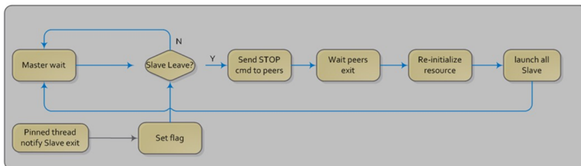
Figure 19.4: Slave Process Recovery Process Flow
