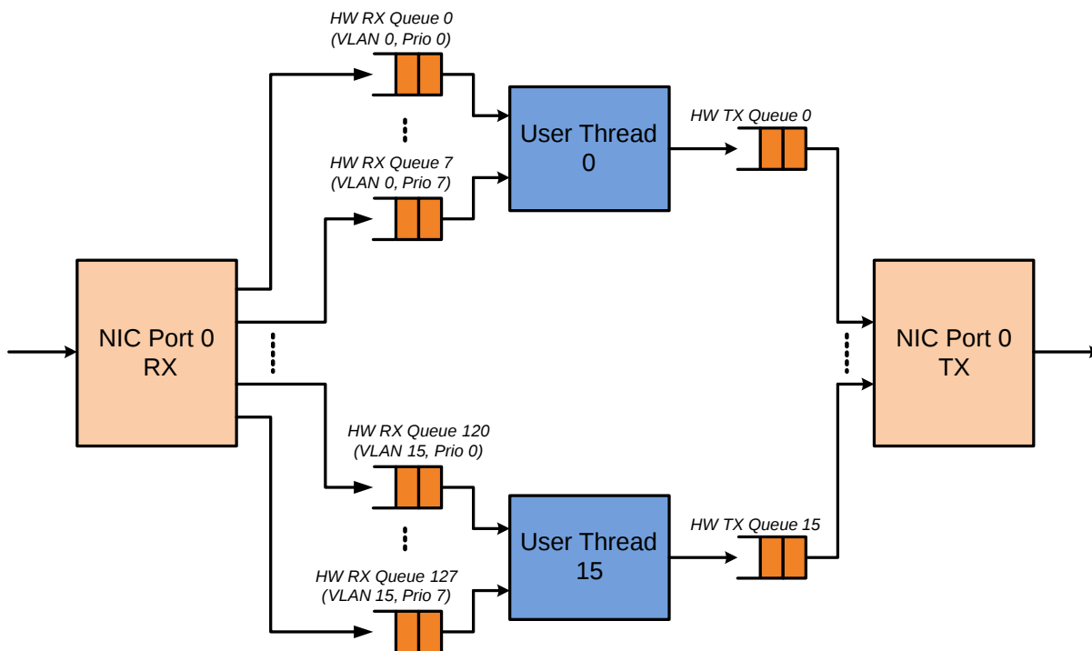
Figure 26.1: Packet Flow Through the VMDQ and DCB Sample Application
