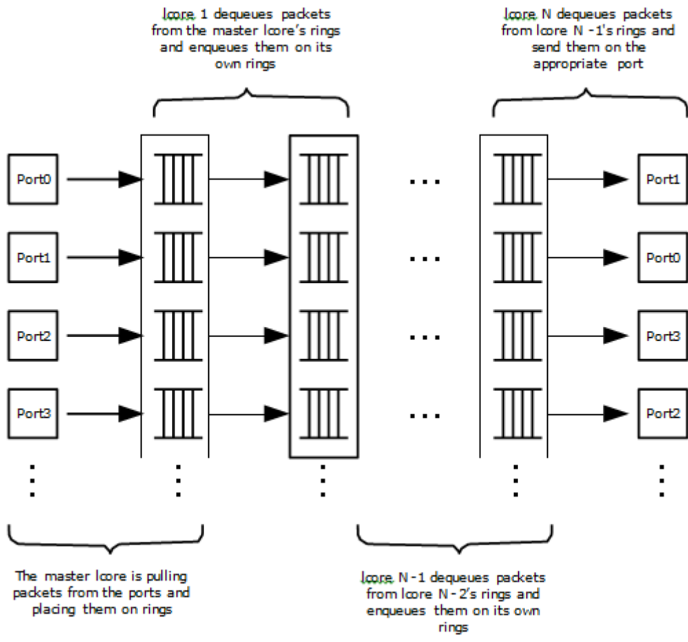
Figure 23.1: Pipeline Overview
