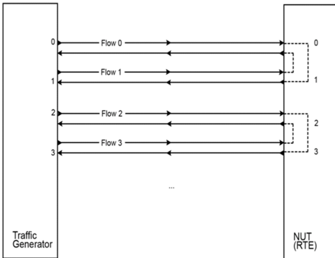
Figure 23.2: Ring-based Processing Pipeline Performance Setup
