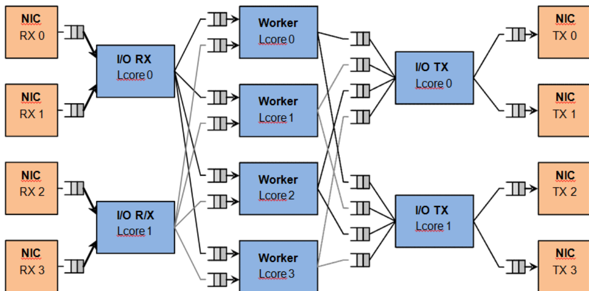
Figure 18.1: Load Balancer Application Architecture
