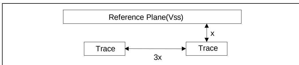
Figure 4-1. Cross-Sectional View of 3:1 Ratio
