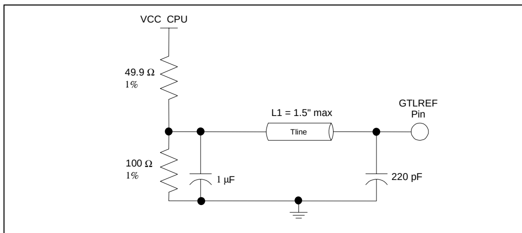
Figure 4-2. GTLREF Routing
