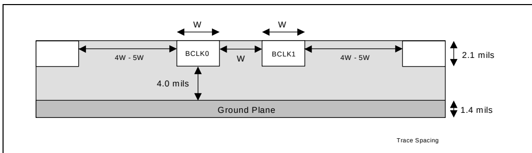
Figure 11-4. Trace Spacing
