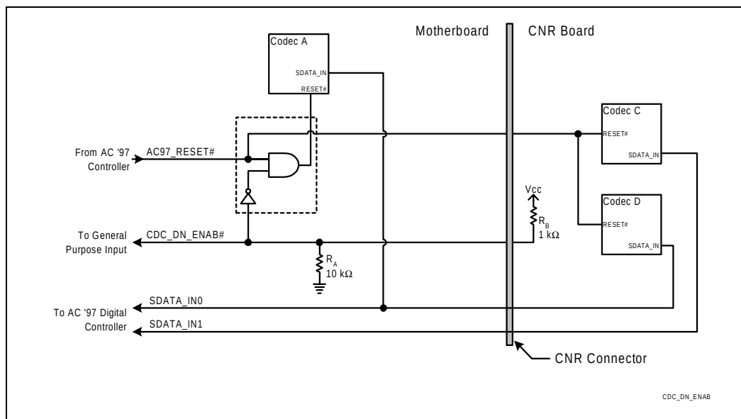
Figure 8-6. CDC_DN_ENAB# Support Circuitry for a Single Codec Motherboard
