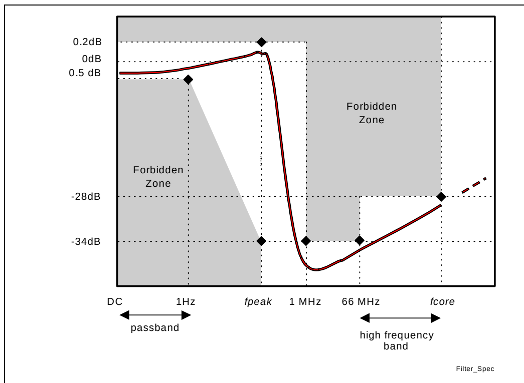
Figure 4-29. Filter Recommendation
