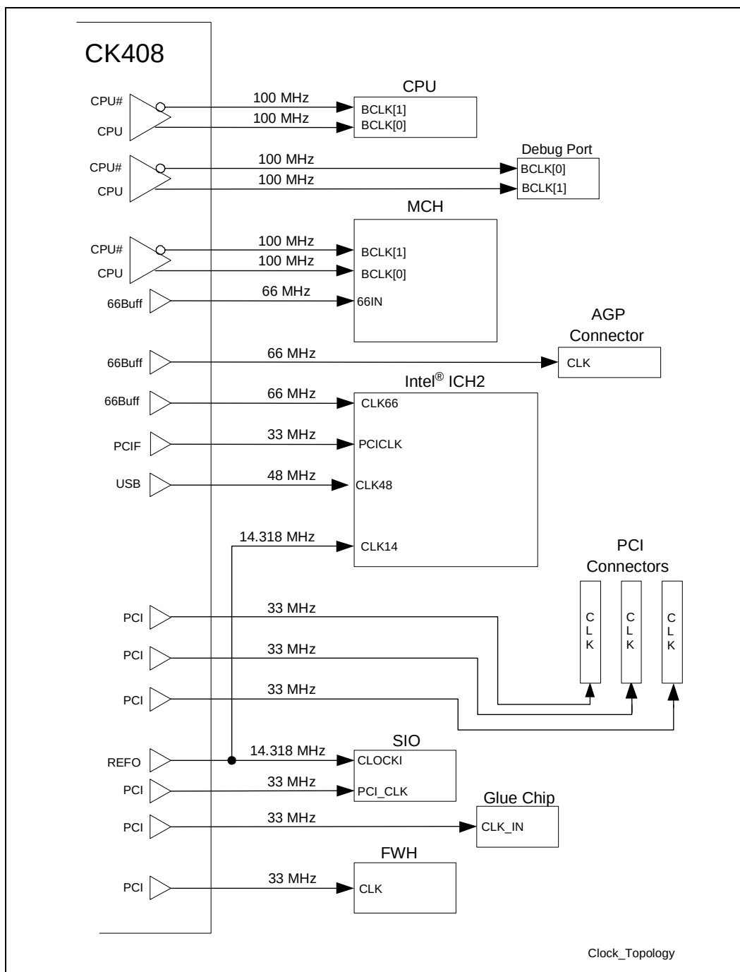
Figure 11-1. Clock Topology
