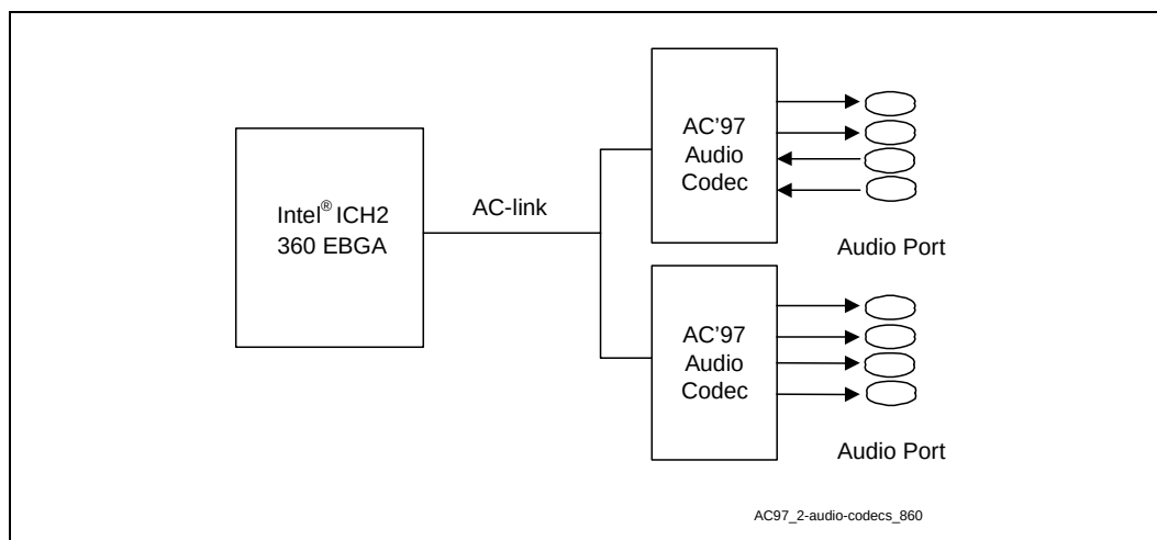
Figure 1-3. AC '97with Audio Codecs (4 Channel Secondary)
