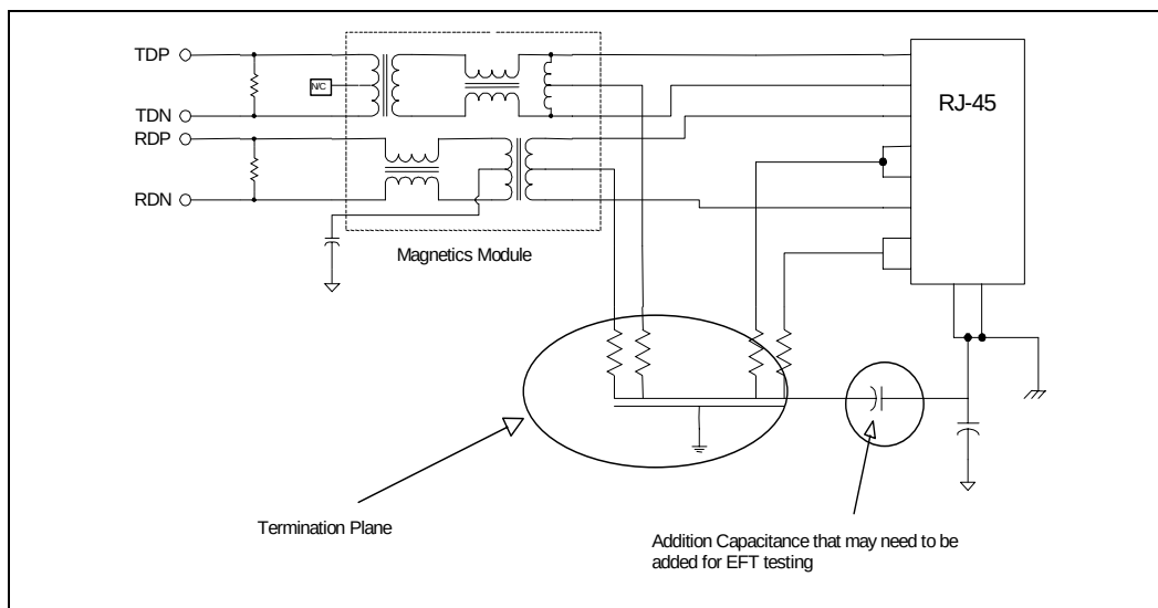
Figure 8-31. Termination Plane
