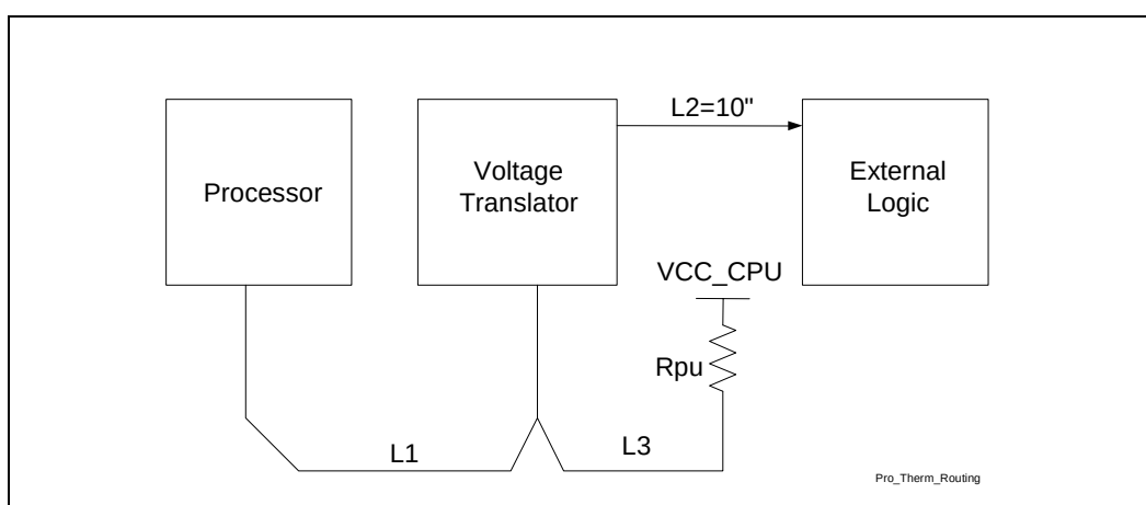
Figure 4-6. Routing Illustration for THERMTRIP#
