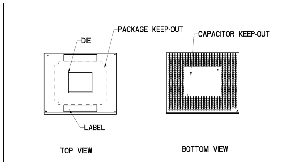
Figure 4. Micro-FCPGA Package Top and Bottom Views
