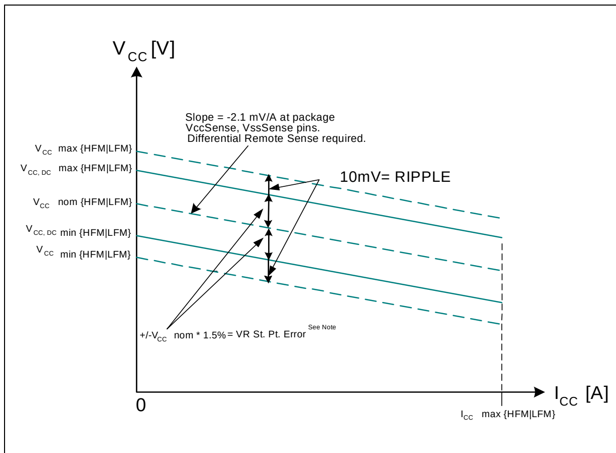
Figure 3. Processor Active V_{CC} and I_{CC} Load Line
