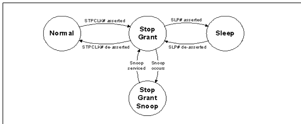
Figure 1. Package-Level Low Power States
