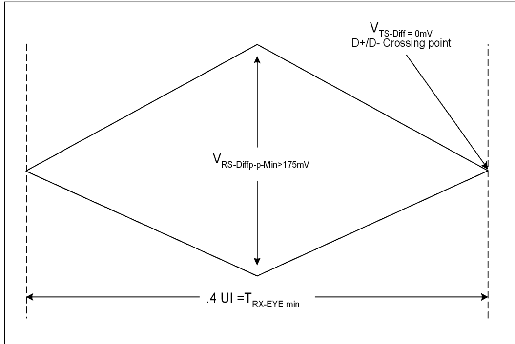
Figure 6-29. PCI Express* Receiver Eye
