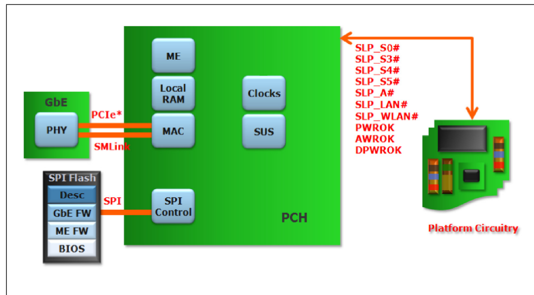
Figure 5-12. PCH Intel® Management Engine (Intel® ME)—High Level Block Diagram
