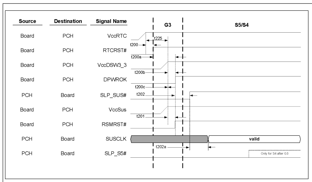
Figure 6-2. G3 w/RTC Loss to S4/S5 (Without Deep Sx Support) Timing Diagram
