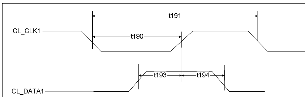
Figure 6-32. Controller Link Receive Timings
