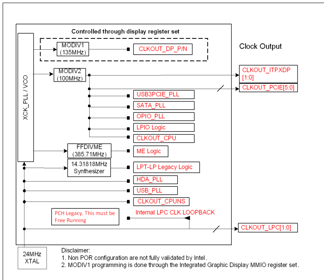
Figure 4-1. PCH Internal Clock Diagram
