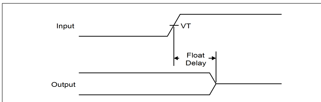
Figure 6-15. Pulse Width
