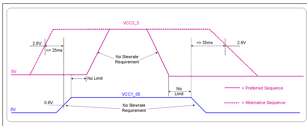
Figure 6-37. Sequencing Requirements Between PCH VCC3_3 and VCC1_05 Core Rail
