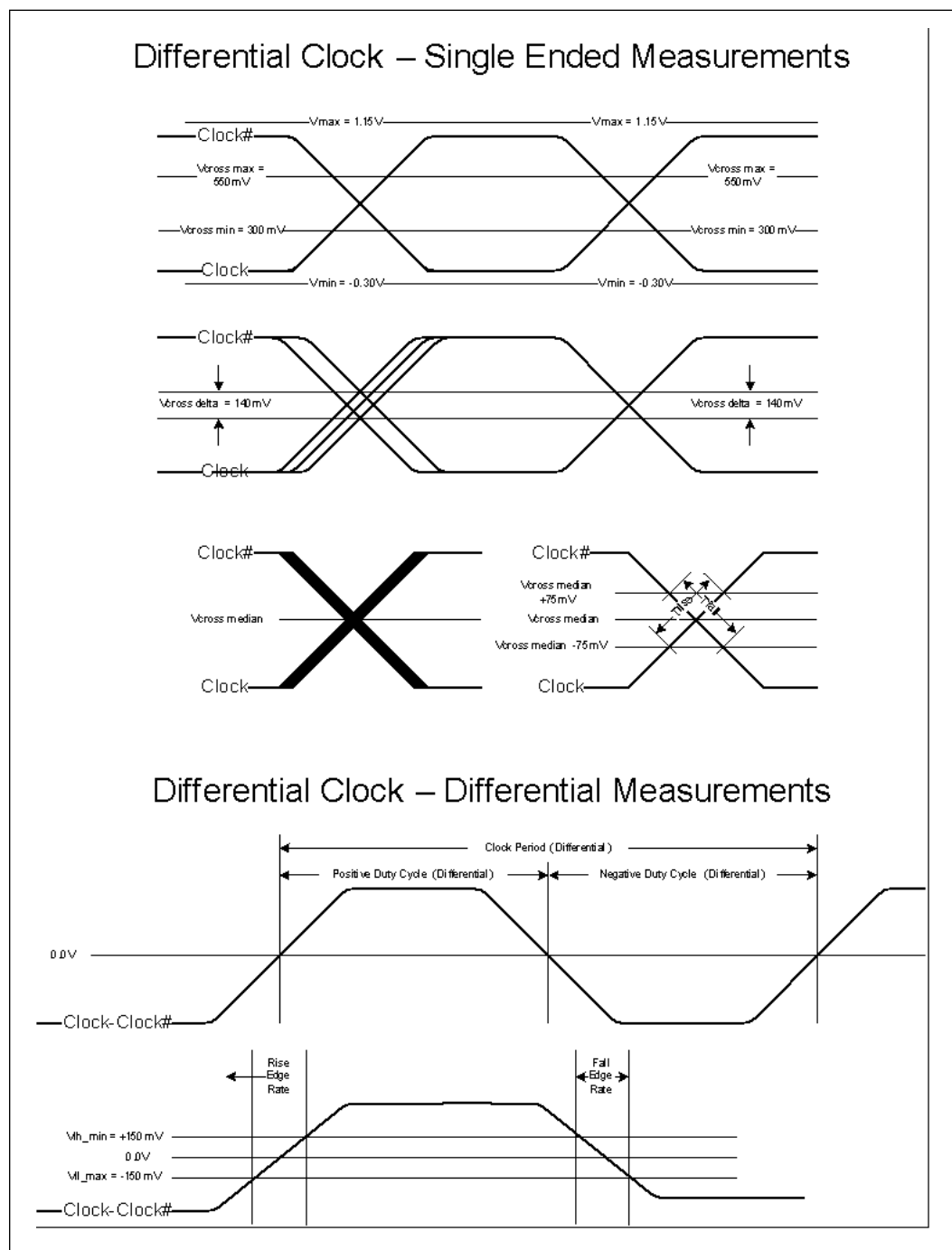
Figure 6-30. Measurement Points for Differential Waveforms
