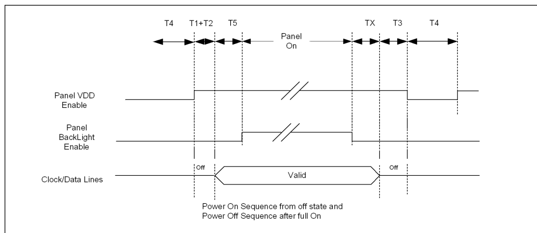
Figure 5-15. Panel Power Sequencing
