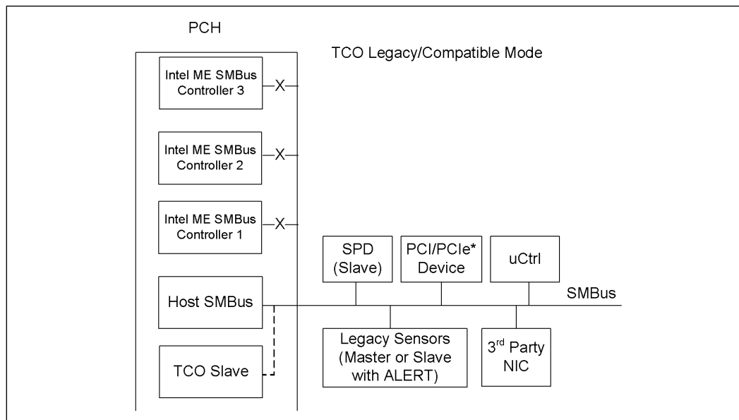
Figure 5-6. Total Cost of Ownership (TCO) Legacy/Compatible Mode SMBus Configuration
