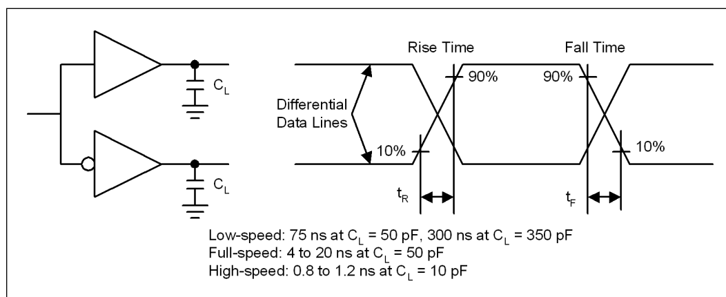
Figure 6-18. USB Jitter
