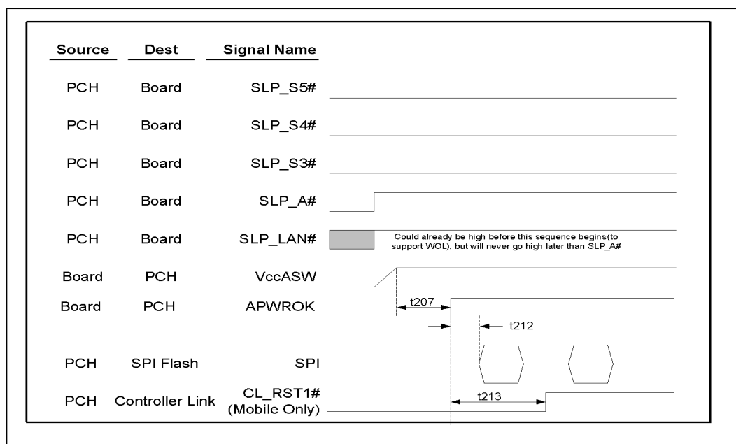
Figure 6-5. S5/M-Off—S5/M3 Timing Diagram
