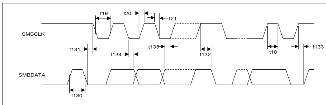
Figure 6-20. SMBus/SMLink Transaction
