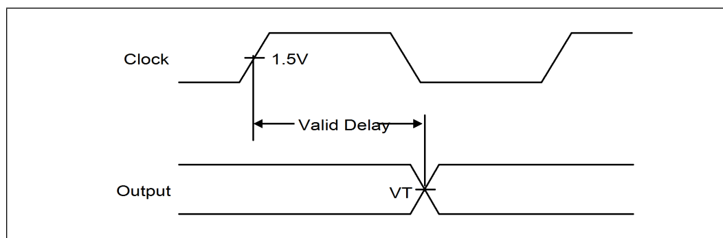
Figure 6-12. Valid Delay from Rising Clock Edge
