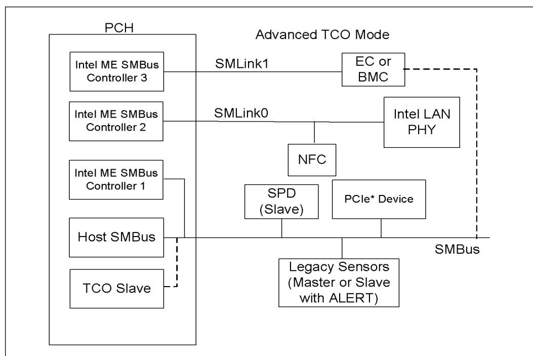
Figure 5-7. Advanced Total Cost of Ownership (TCO) Mode
