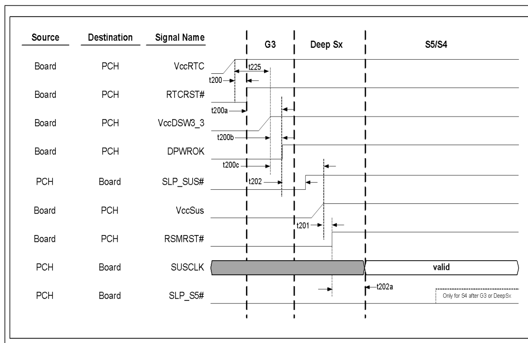
Figure 6-1. G3 w/RTC Loss to S4/S5 (with Deep Sx Support) Timing Diagram
