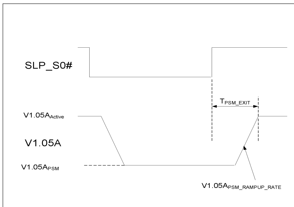
Figure 6-34. Windows* InstantGo Power Save Mode (Windows* InstantGo PSM) Timing Diagram
