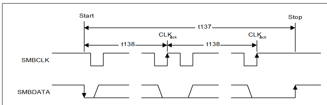
Figure 6-21. SMBus/SMLink Timeout
