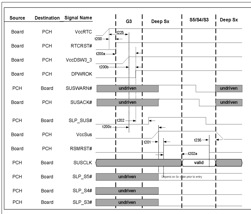
Figure 6-8. G3 to Deep Sx Timing Diagram
