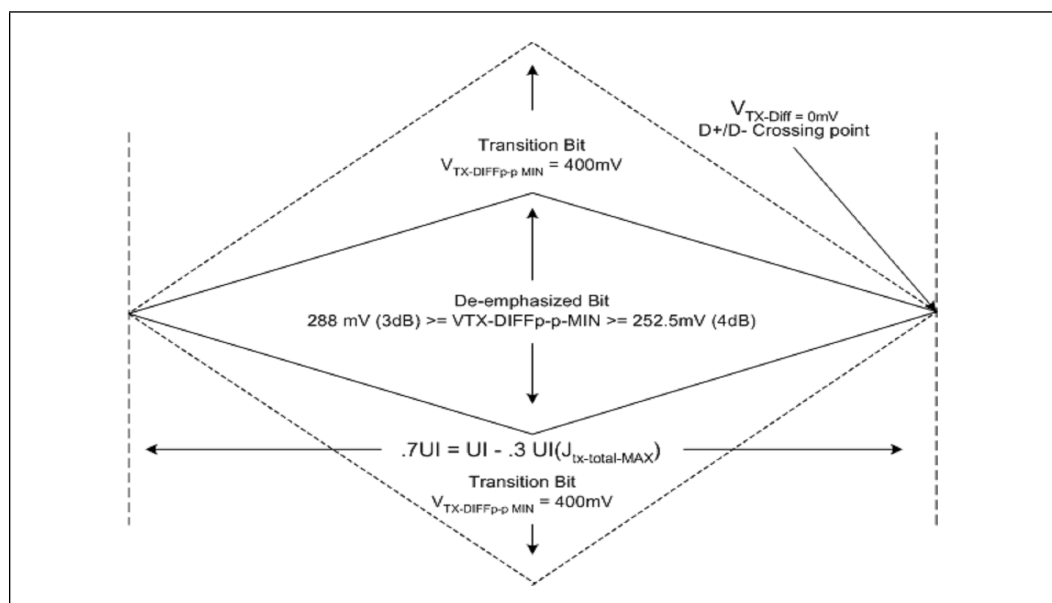
Figure 6-28. PCI Express Transmitter Eye
