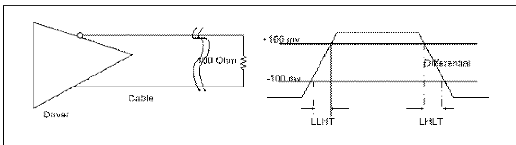
Figure 6-26. LVDS Load and Transition Times
