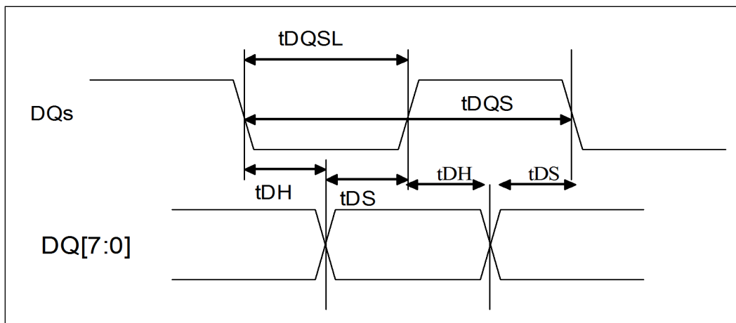
Figure 6-25. Dual Channel Interface Timings—B
