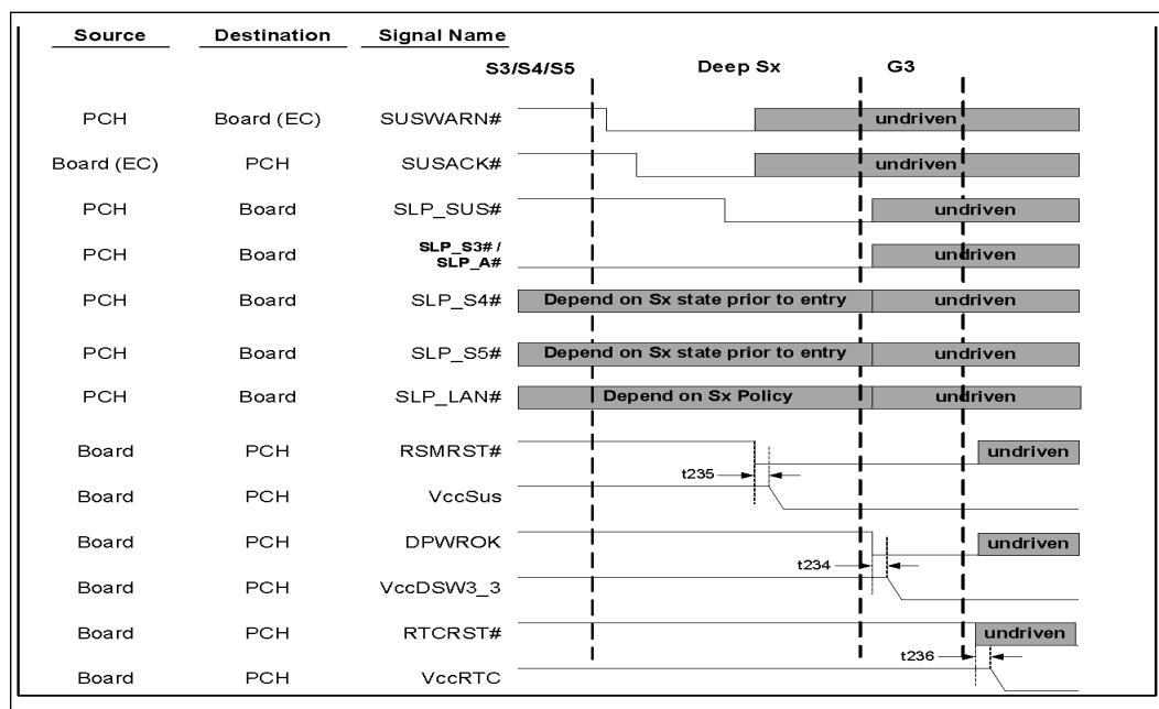
Figure 6-7. S3/S4/S5 to Deep Sx to G3 w/RTC Loss Timing Diagram
