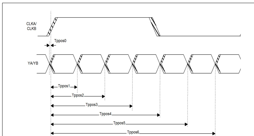
Figure 6-10. Transmitting Position (Data to Strobe)
