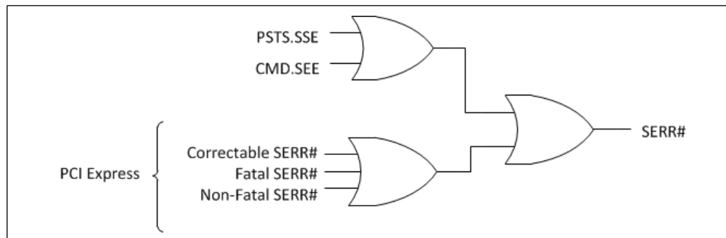
Figure 5-2. Generation of SERR# to Platform
