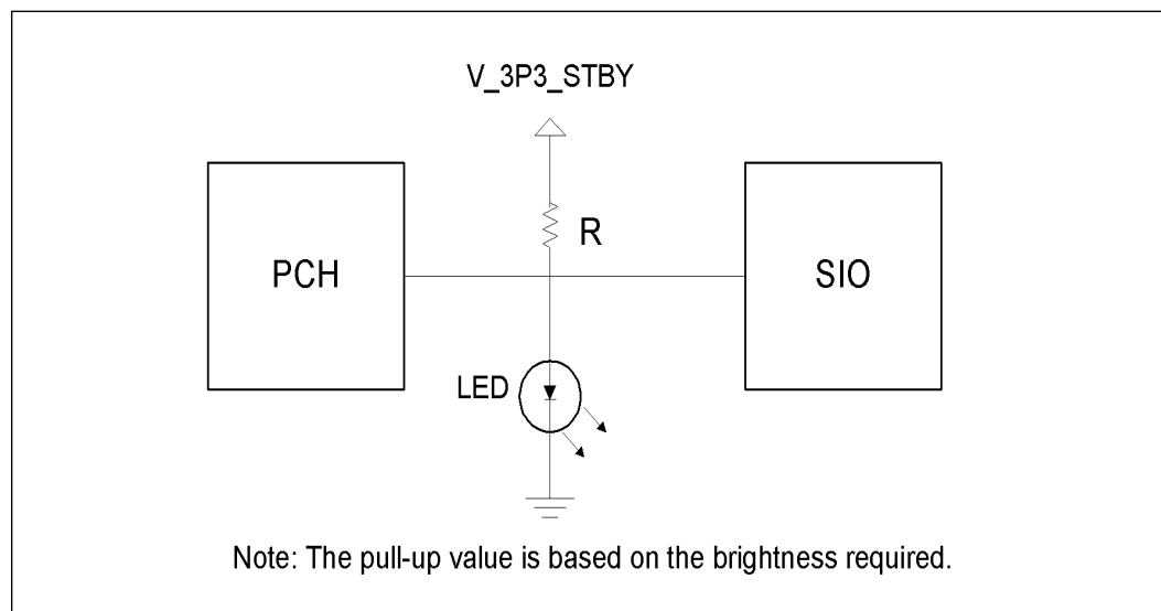
Figure 5-8. Serial POST Over GPIO Reference Circuit
