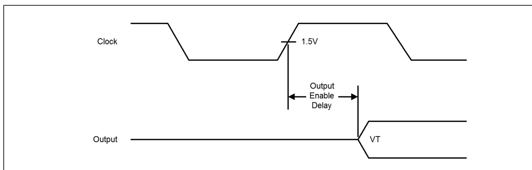
Figure 6-16. Output Enable Delay
