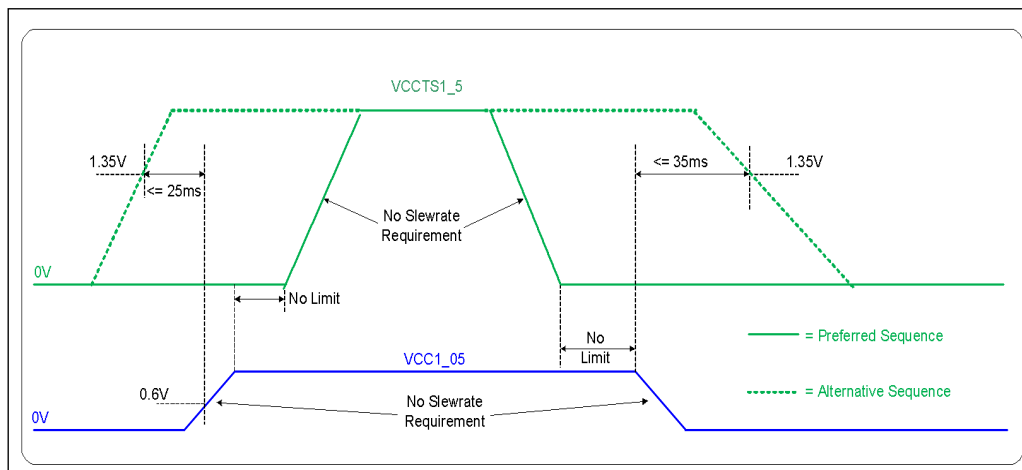
Figure 6-38. Sequencing Requirements Between PCH VCCTS1_5 and VCC1_05 Core Rail
