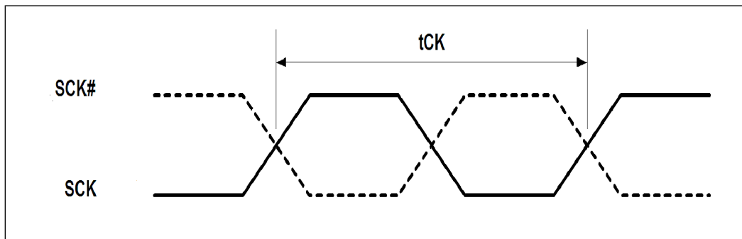
Figure 6-9. Clock Cycle Time
