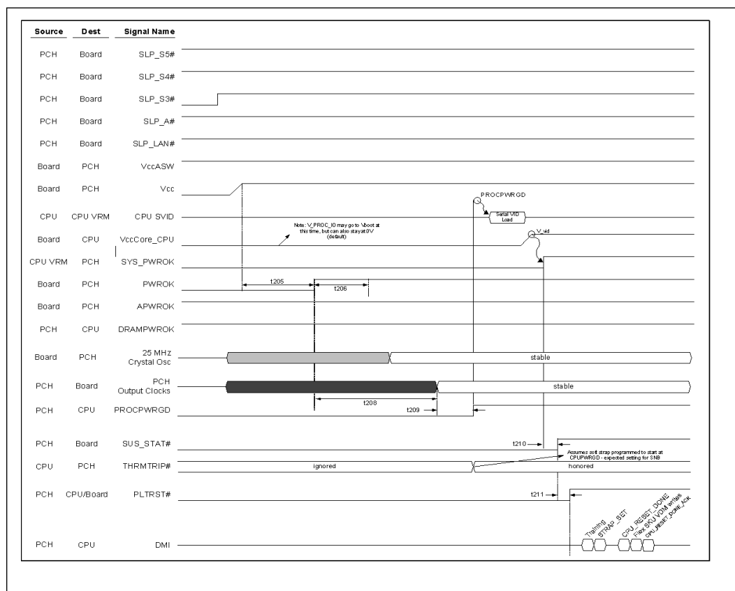
Figure 6-4. S3/M3 to S0 Timing Diagram
