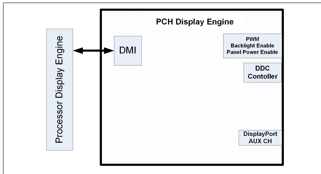
Figure 5-14. PCH Display Architecture
