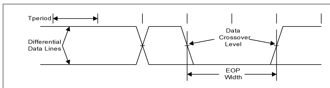
Figure 6-19. USB EOP Width
