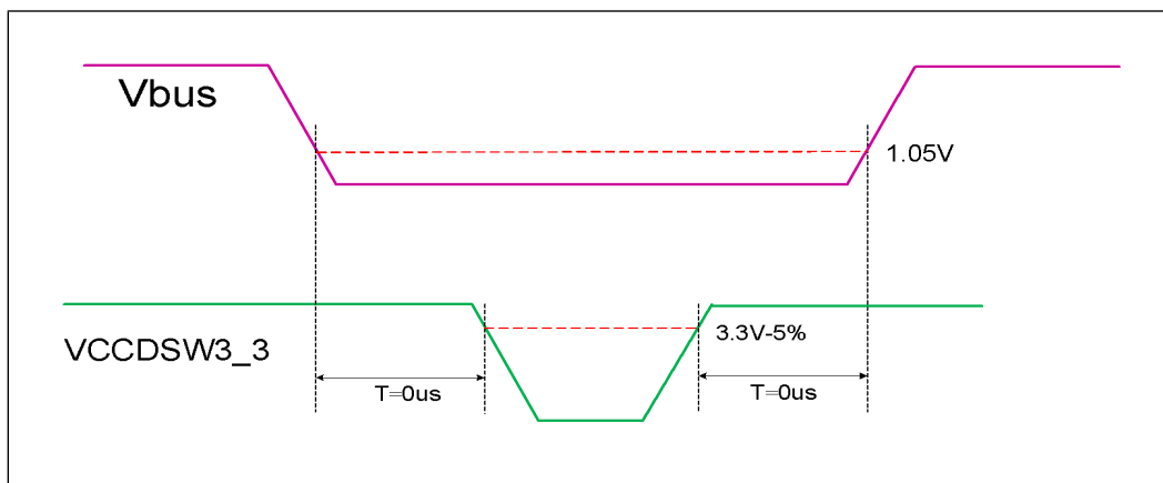
Figure 6-36. Suspend Well Ramp Up/Down Requirement
