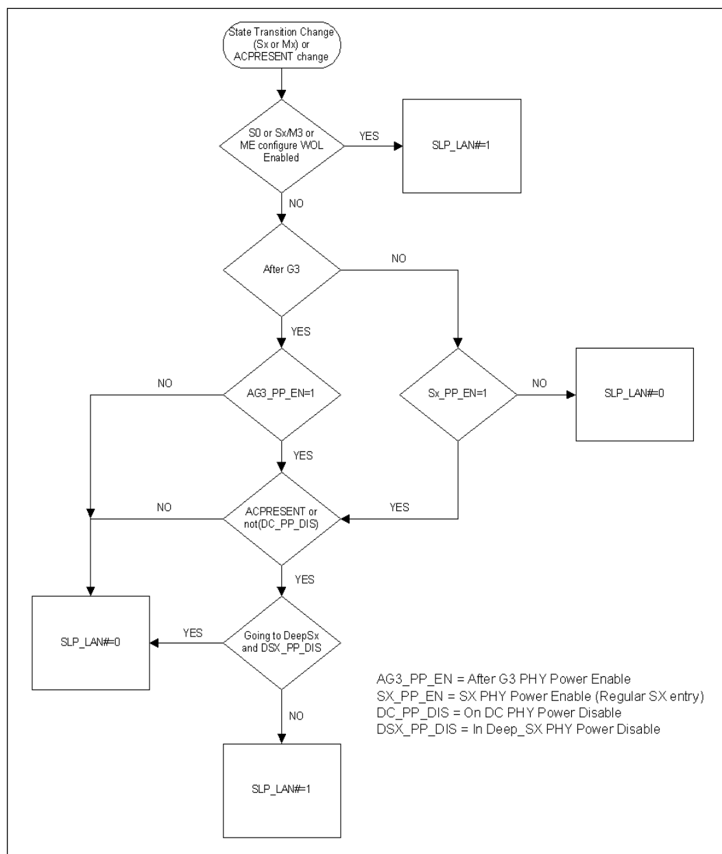
Figure 5-5. Conceptual Diagram of SLP_LAN#
