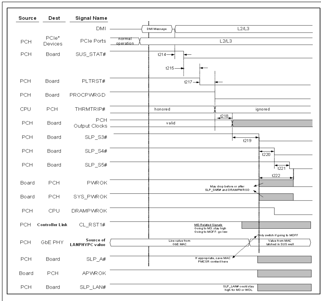
Figure 6-6. S0 to S5 Timing Diagram
