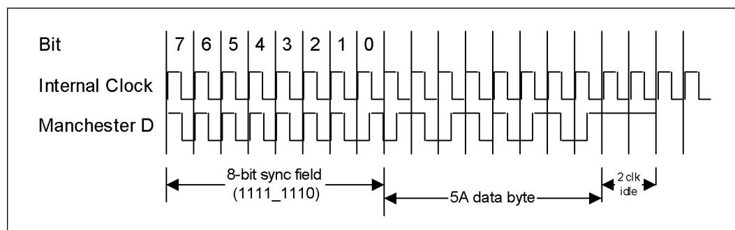
Figure 5-9. One-Byte Serial Write with Data Byte of 5Ah
