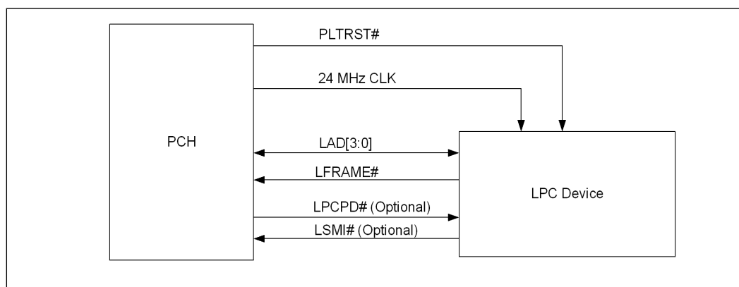
Figure 5-4. Low Pin Count (LPC) Interface Diagram
