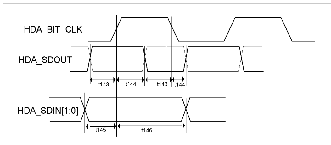
Figure 6-23. Intel® High Definition Audio (Intel® HD Audio) Input and Output Timings
