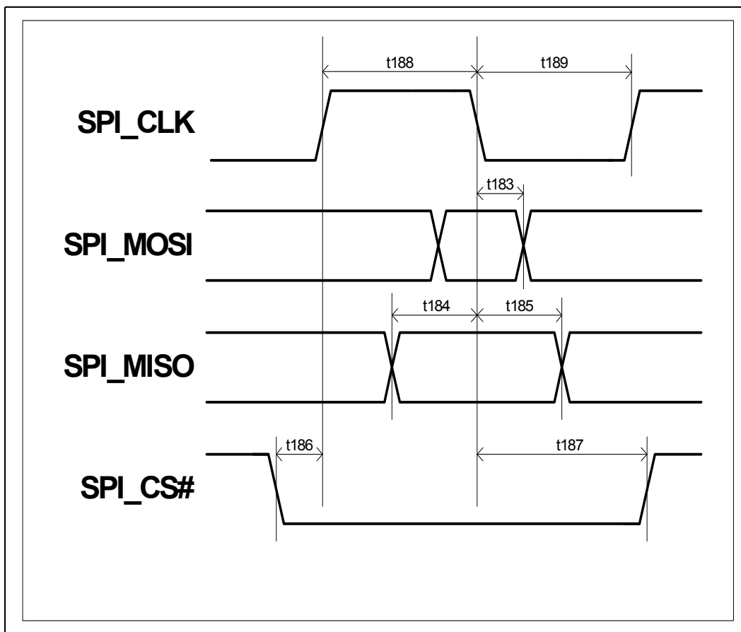
Figure 8-23. SPI Timings
