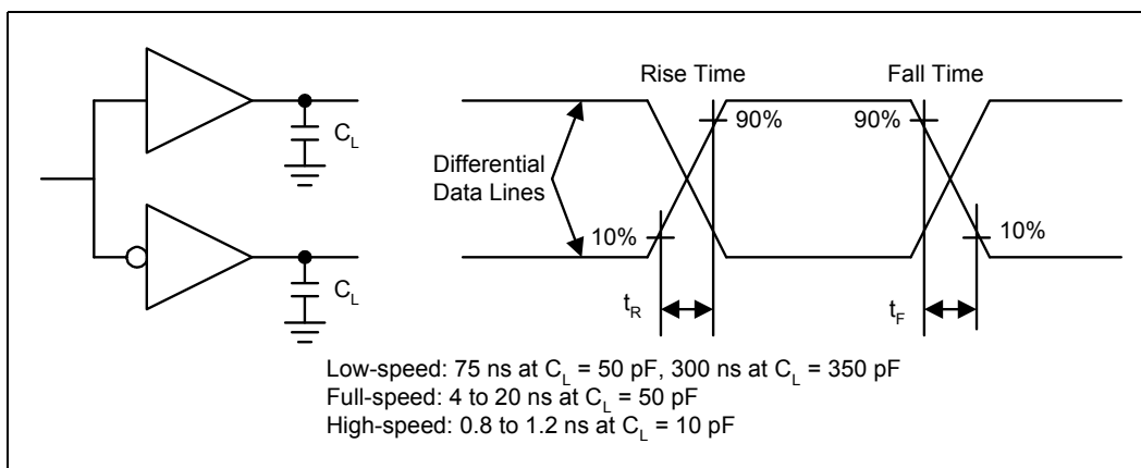
Figure 8-18. USB Rise and Fall Times
