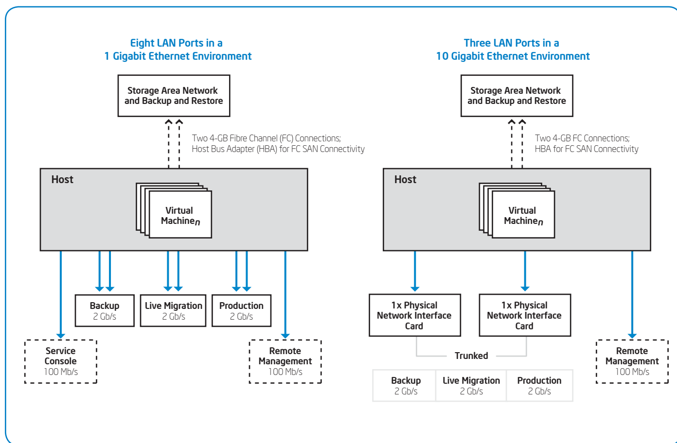
Figure 1. Implementing a 10 gigabit Ethernet data center fabric reduces the number of LAN ports for our virtualized host architecture from eight to three.
