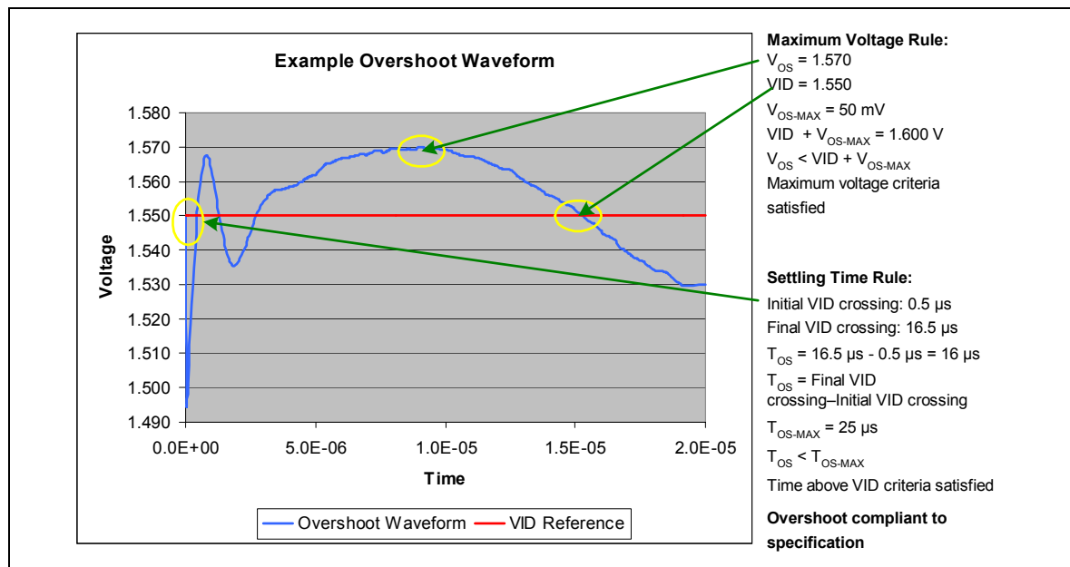
Figure 5. Example Socket Vcc Overshoot Waveform
