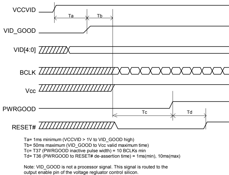
Figure 3: Power-on Sequence Timing Diagram
