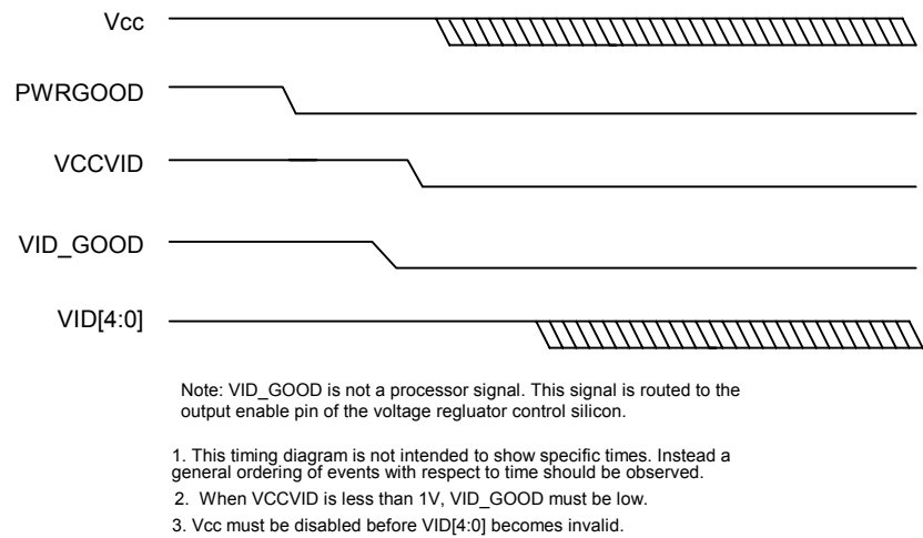
Figure 4: Power-off Sequence Timing Diagram
