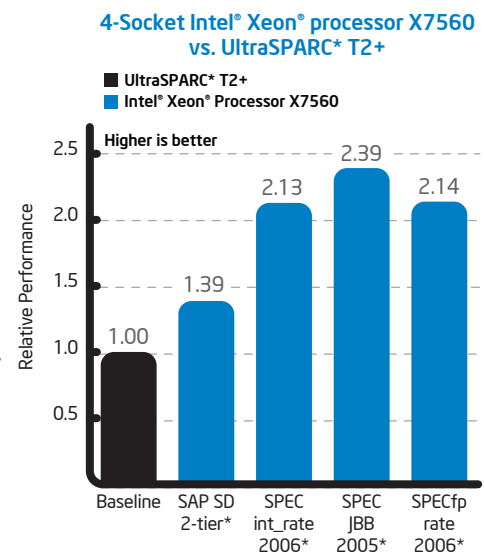
Figure 3. Based on published benchmarks, Intel® Xeon® processor 7500 series-based systems provide up to 2.39x higher performance than UltraSPARC2* processor-based systems. All comparisons based on published/submitted/approved results as of April 2010.
