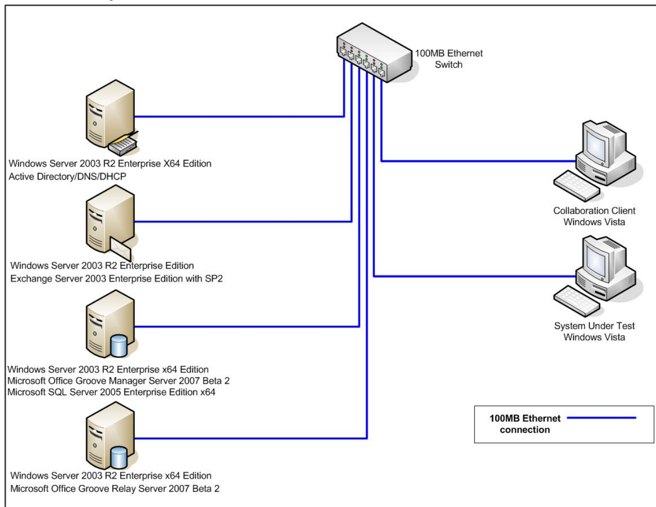
Figure 12: Diagram of the test network.
