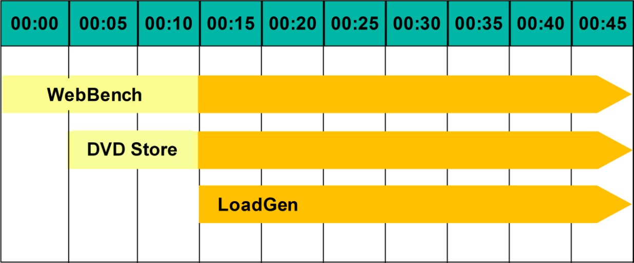
Figure 5: The timeline we followed when starting the benchmarks for the multiple-benchmark runs on all Intel processor-based servers. The shaded areas from 00:15 to 00:45 represent the period during which we measured performance.
