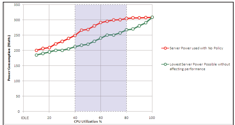
Figure 7. Power savings versus CPU utilization without a power policy and with a power policy
