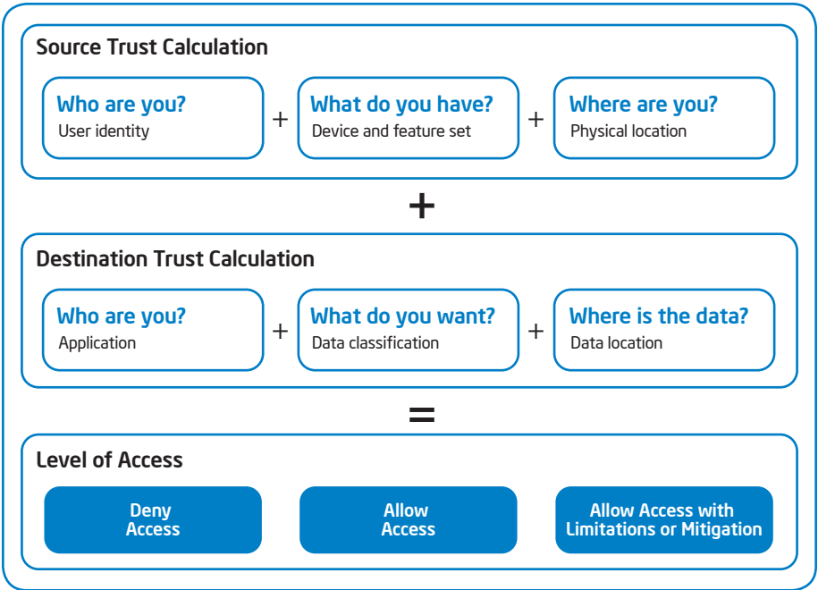
Figure 2. The trust calculation takes into account who, what, and where for both source and destination.
