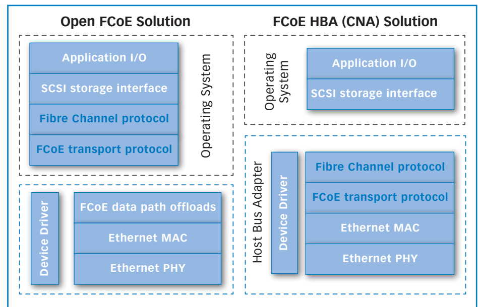
Figure 2. Overview of Fibre Channel over Ethernet (FCoE) host bus adapters (converged network adapters) and Open FCoE initiator solutions
