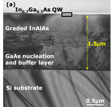
Fig. 6(a): Cross-sectional TEM micrograph of \text{In}_{0.7}\text{Ga}_{0.3}\text{As} QW stack with InP top barrier layer on Si substrate via 1.5\mu\text{m} composite buffer. All III-V layers were grown using MBE.
