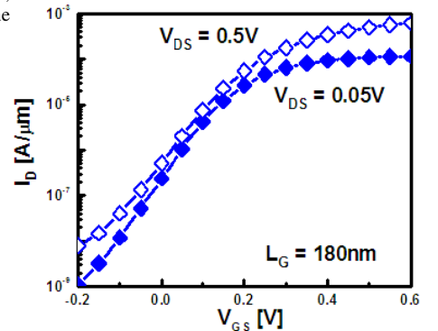
Fig. 10: Drain current ( I_D ) versus gate voltage ( V_{GS} ) of L_G=180\text{nm} \text{In}_{0.7}\text{Ga}_{0.3}\text{As} QWFET with composite 4nm \text{TaSiO}_x -2nm InP gate stack ( t_{\text{OXE}}=22\text{\AA} ). At V_{DS}=0.5\text{V} the device shows excellent subthreshold slope ( SS ) = 85\text{mV}/\text{dec} and drain induced barrier lowering (DIBL) = 35\text{mV}/\text{V} .
