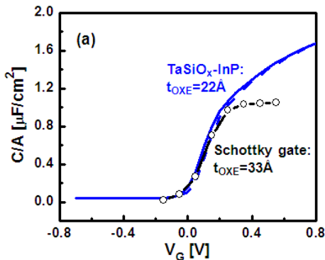
Fig. 9(a): C-V_G measured on the \text{In}_{0.7}\text{Ga}_{0.3}\text{As} QWFET with the composite 4nm \text{TaSiO}_x -2nm InP gate stack showing minimal hysteresis and t_{\text{OXE}}=22\text{\AA} . Included is C-V_G of the Schottky-gate QWFET (extracted at RF due to high J_G ) with t_{\text{InAlAs}}=5\text{nm} and t_{\text{OXE}}=33\text{\AA} .
