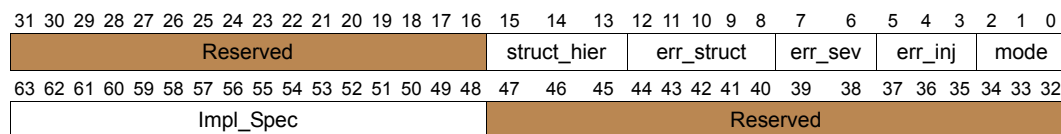
Figure 11-25. err_type_info
