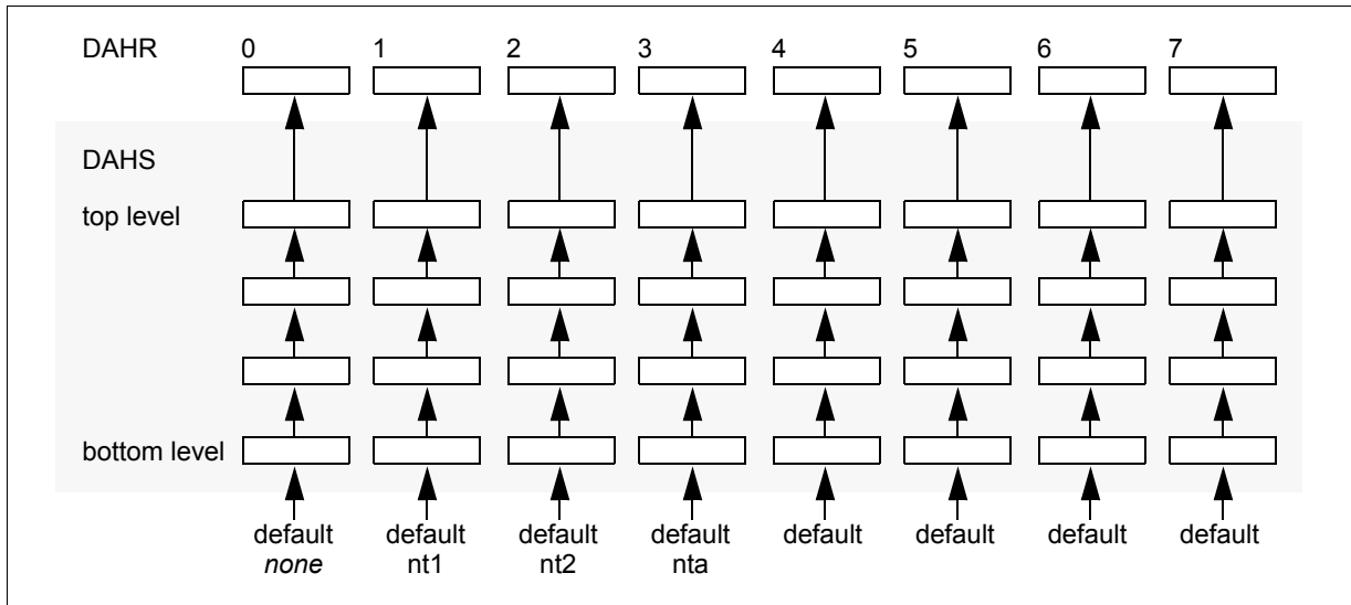
Figure 4-5. Data Access Hint Stack Operation on br.ret
