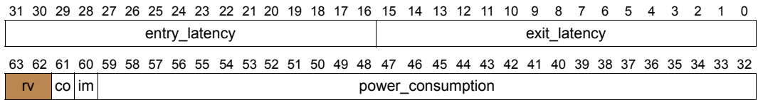
Figure 11-14. Layout of power_buffer Return Value
