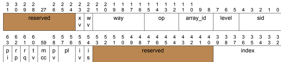
Figure 11-24. uarch_check Layout
