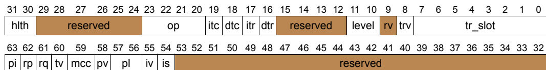
Figure 11-21. tlb_check Layout
