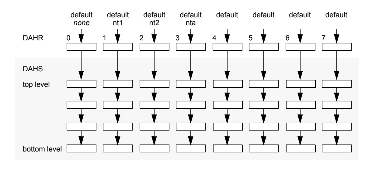
Figure 4-4. Data Access Hint Stack Operation on br.call
