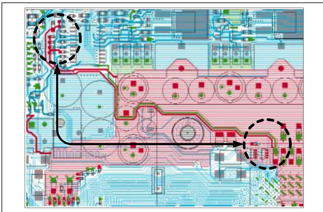
Figure 36. Routing of VR Feedback Signal
