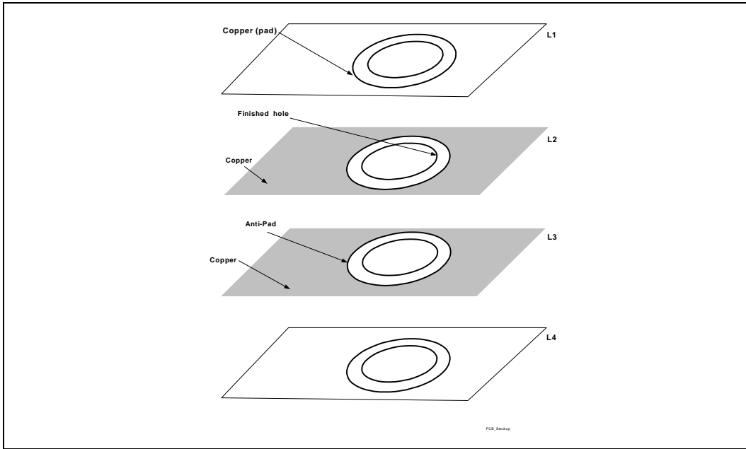
Figure 10. PCB Technologies—Stack-Up
