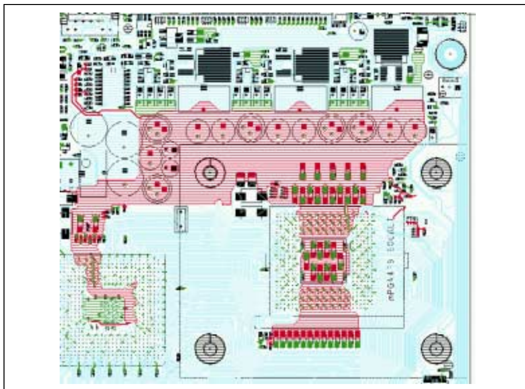
Figure 30. Top Layer Power Delivery Shape ( V_{CC\_CPU} )
