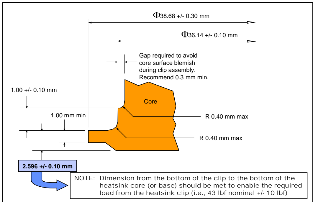
Figure 23. Critical Core Dimension
