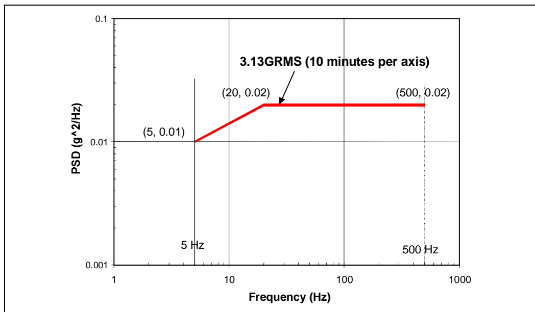
Figure 17. Random Vibration PSD
