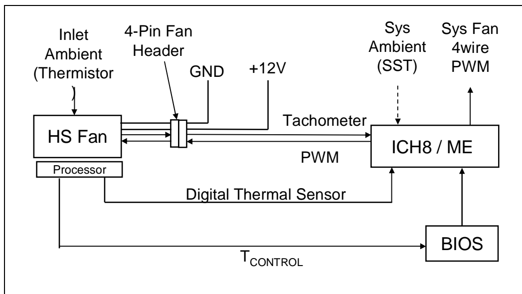
Figure 62. Example Fan Speed Control Implementation
