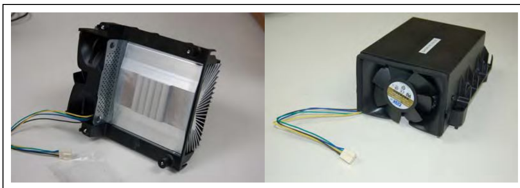
Figure 13. Intel Type II TMA 65W Reference Design
