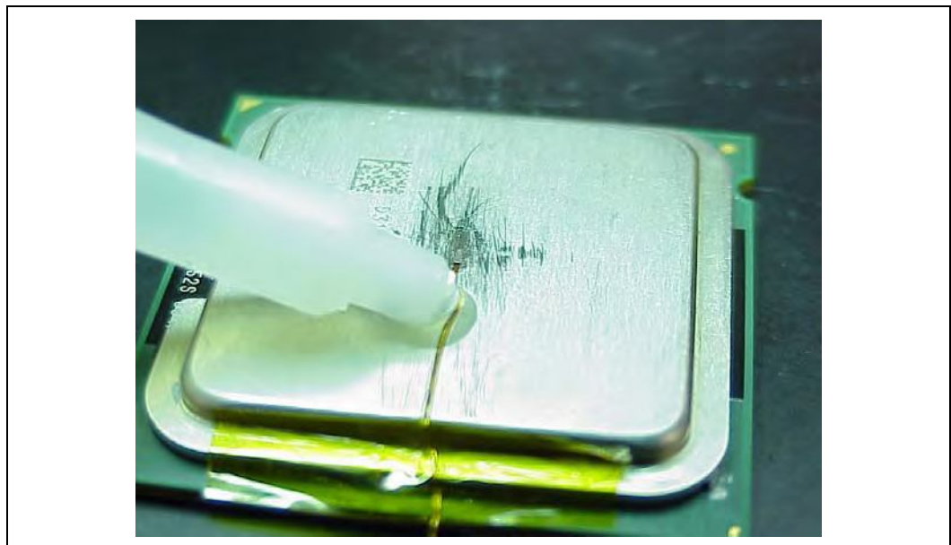
Figure 56. Filling Groove with Adhesive
