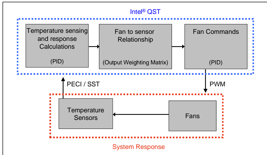
Figure 24. Intel® QST Overview
