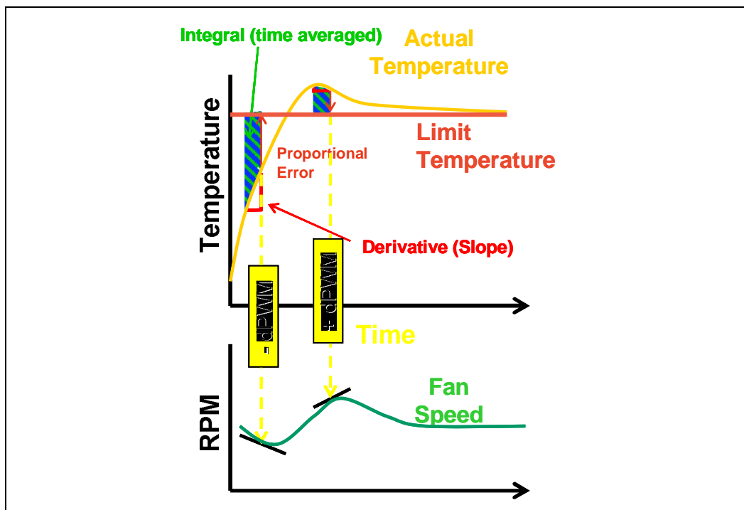
Figure 25. PID Controller Fundamentals
