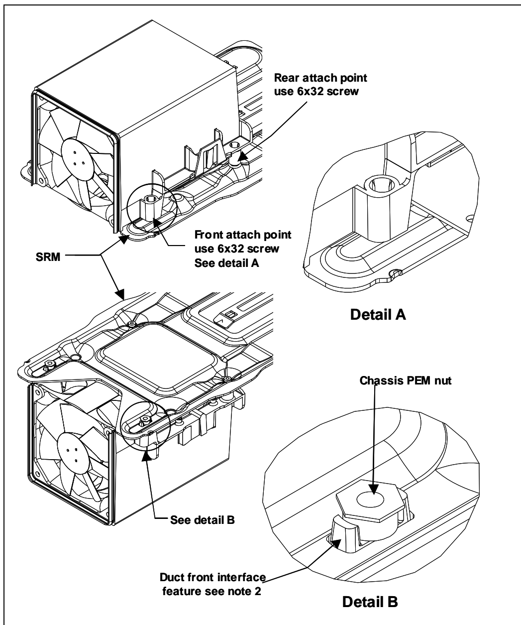
Figure 16. Thermal Module Attach Pointes and Duct-to-SRM Interface Features
