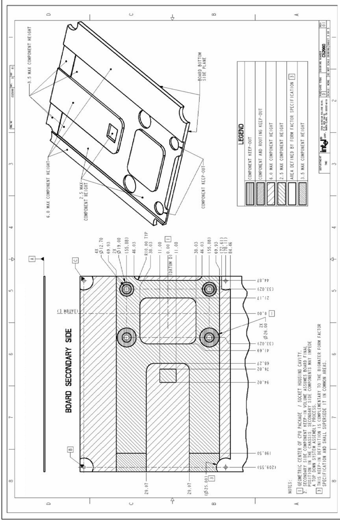
Figure 75. Balanced Technology Extended (BTX) Thermal Module Keep Out Volumetric – Sheet 3
