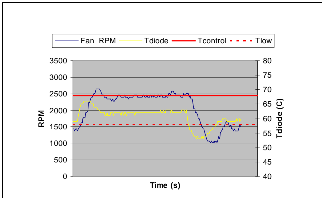
Figure 65. Temperature Range = 10 °C
