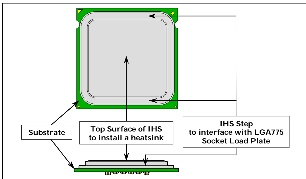
Figure 1. Package IHS Load Areas
