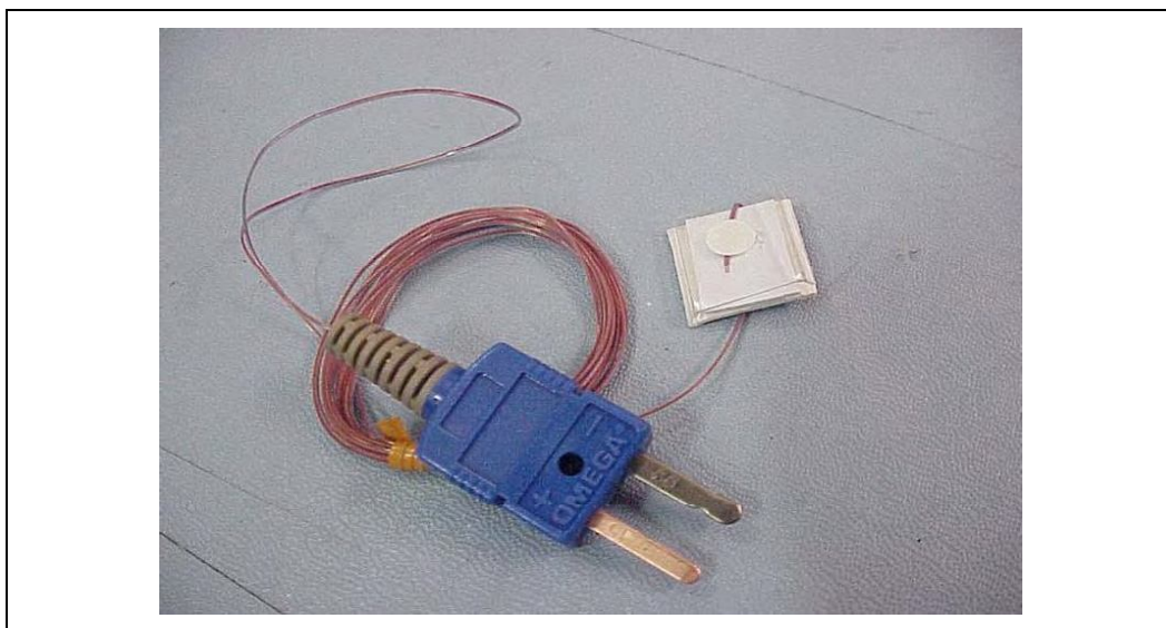
Figure 34. Omega Thermocouple
