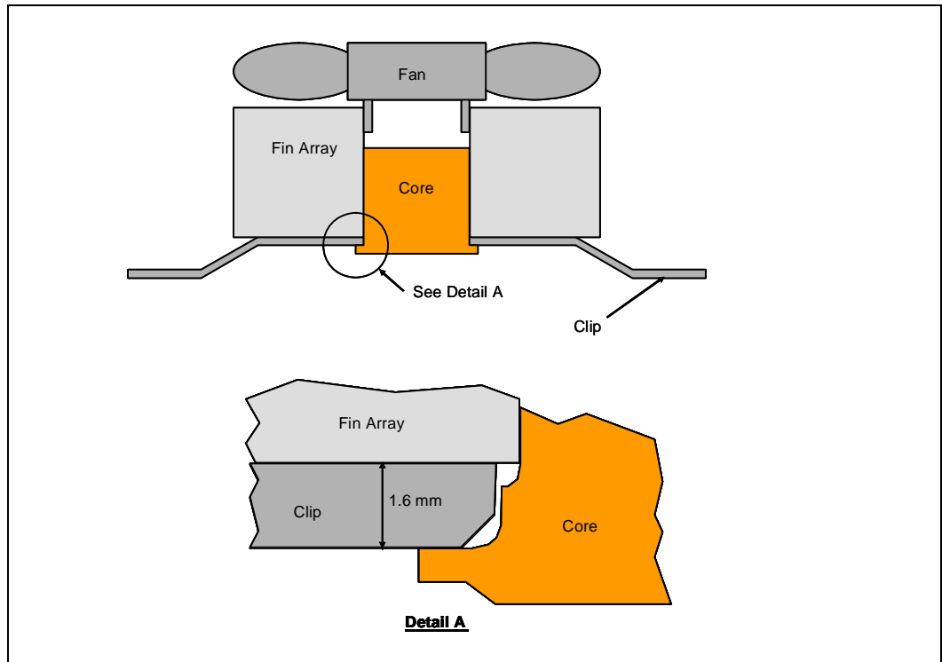
Figure 22. Critical Parameters for Interfacing to Reference Clip
