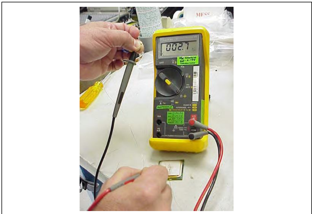
Figure 46. Measuring Resistance between Thermocouple and IHS
