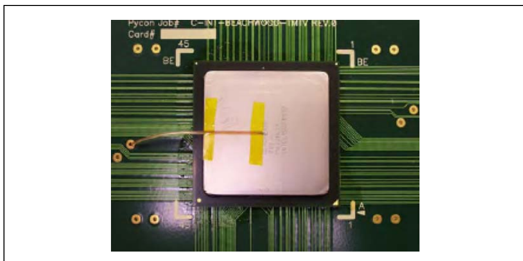
Figure 5-10. Tapes Installation
