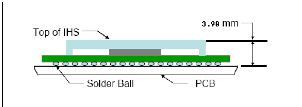
Figure 2-5. Package Height
